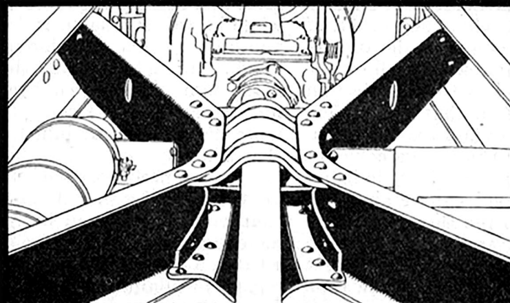
Twist-proof X-frame originated by Auburn makes Auburn's frame the strongest and most rigid.
