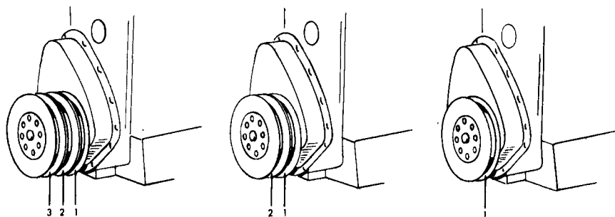
(8 cylinder) Drive Pulley, (Crankshaft) Groove No. 1, (1, 2, or 3 pulley systems)
