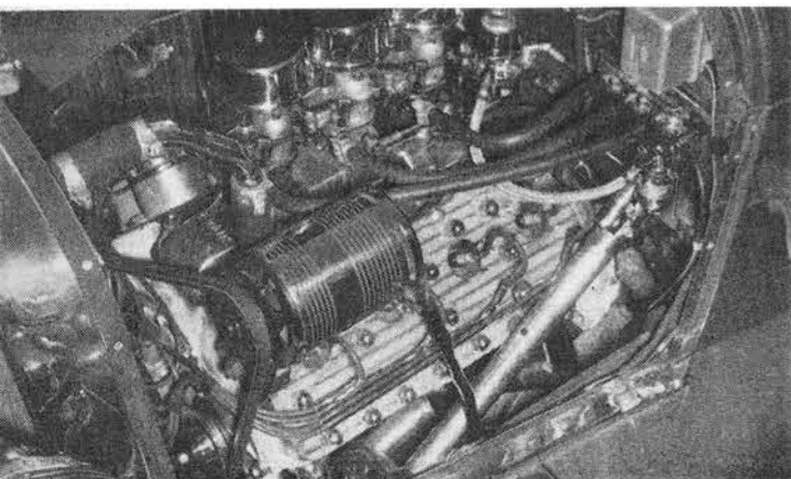
Roadster carries '48 block with .080 overbore running Weber cam, Evans heads and manifold, Harman and Collins ignition
