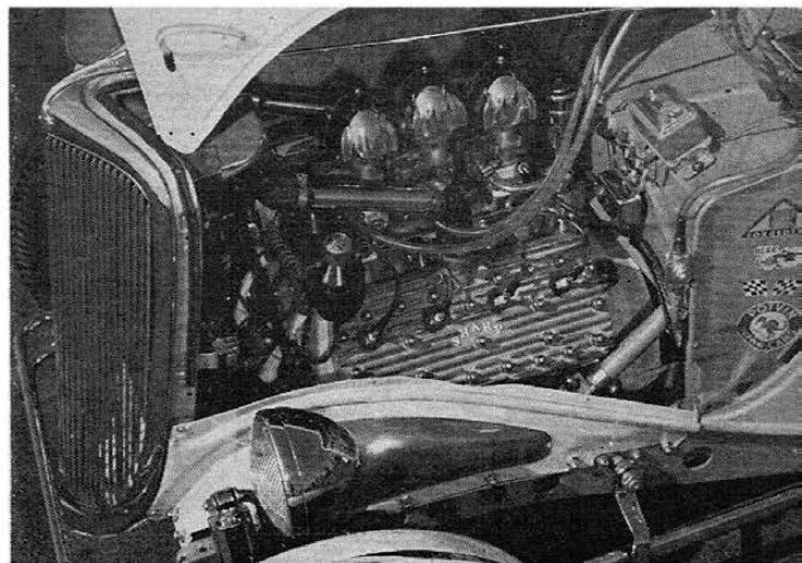
Full house 286 ci Merc carries Potvin cam, Weber crank. Bumper is homemade
