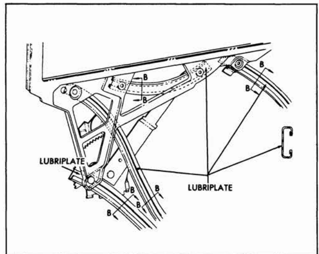
Fig. 10-12 Rear Quarter Window Cams
