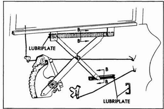
Fig. 10-11 Rear Door Window Regulator Cams
