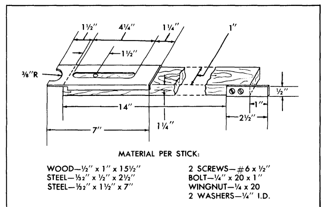
Fig. 22-34 Spacer Stick Dimensions
