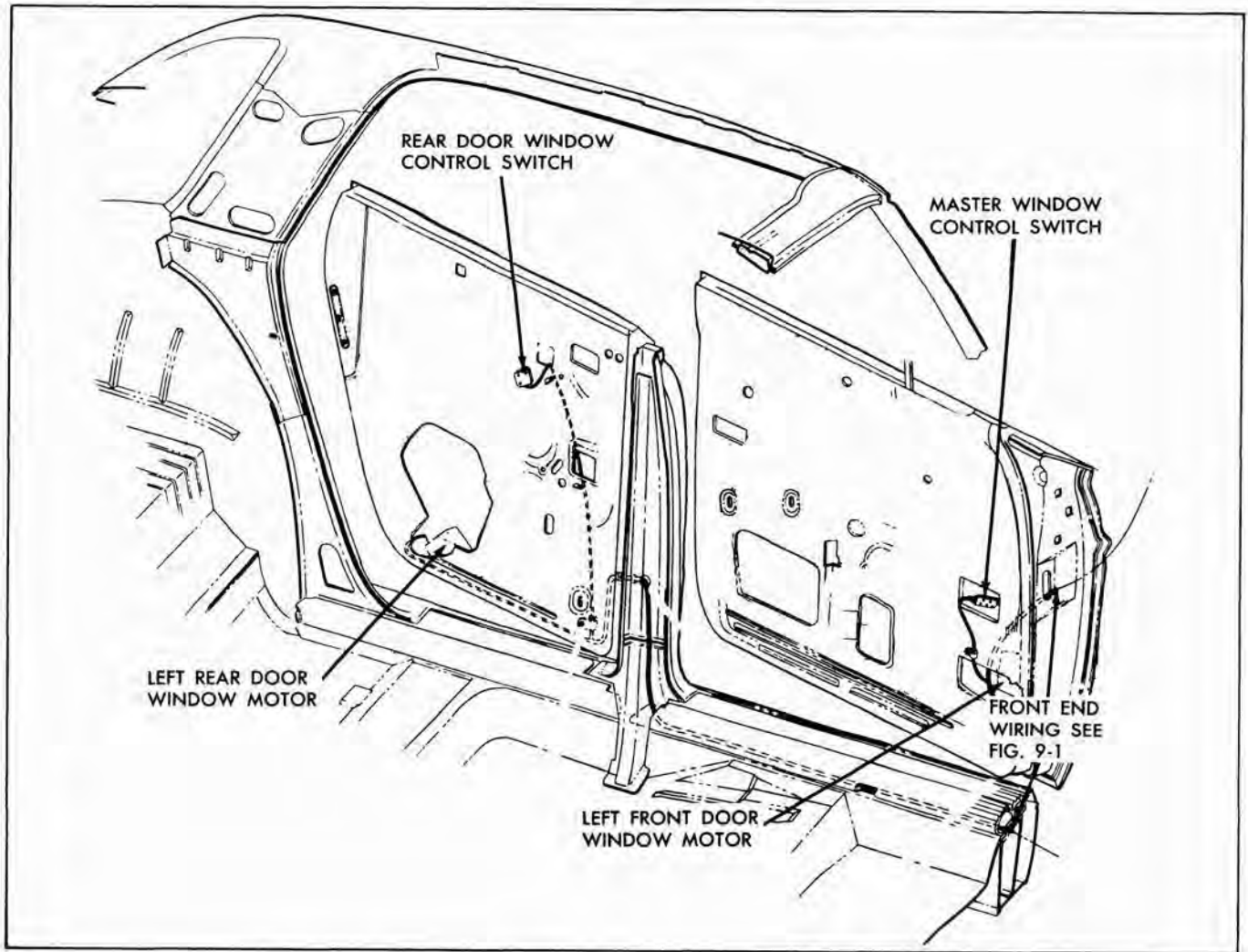
Fig. 9-2 Left Side Power Window Wiring Installation
