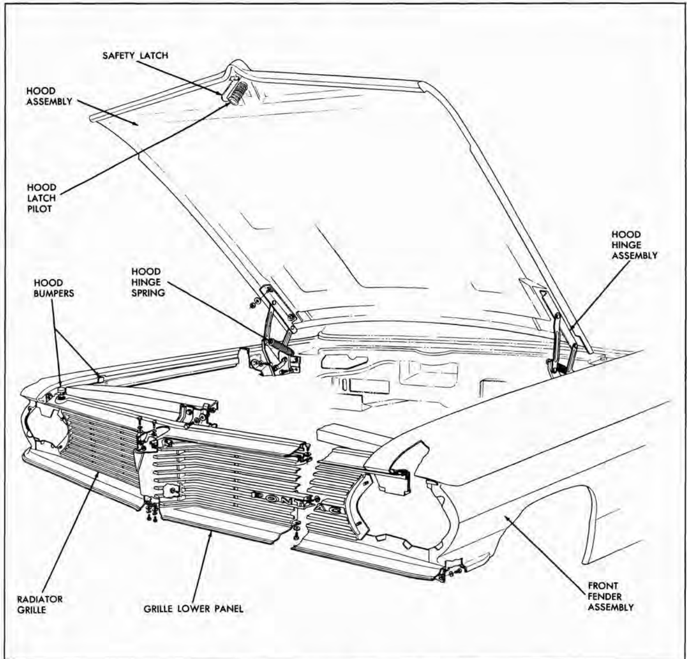
Fig. 1-7 Sheet Metal Parts - Installation
