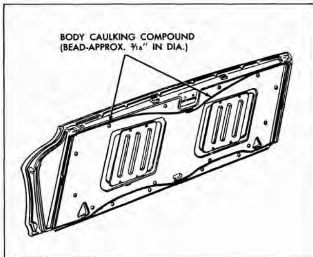
Fig. 5-23 Tail Gate Inner Panel
