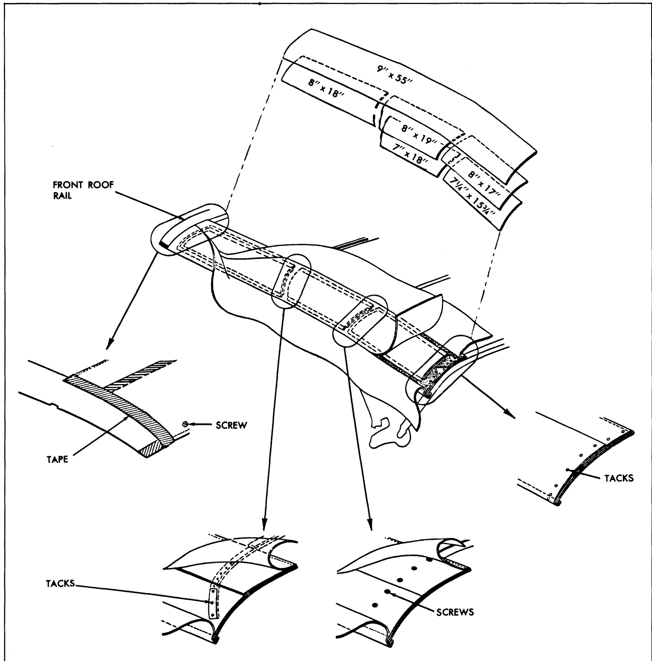
Fig. 22-37 Installation of Side Stay Pads ("Y" Styles)
