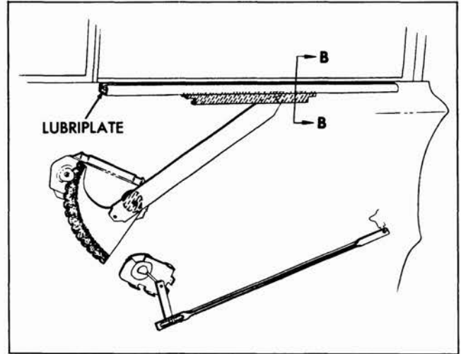
Fig. 10-10 Front Door Window Regulator Cams
