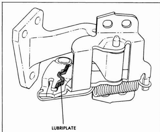
Fig. 10-1 Front Door Hinge and Hold Open
