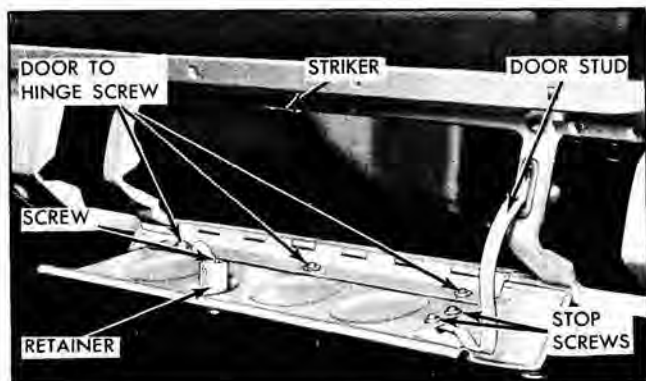
Fig. 2-11 Instrument Panel Compartment Door
