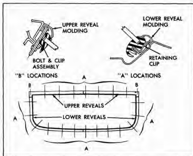
Fig. 5-4 Back Window Reveal Moldings
