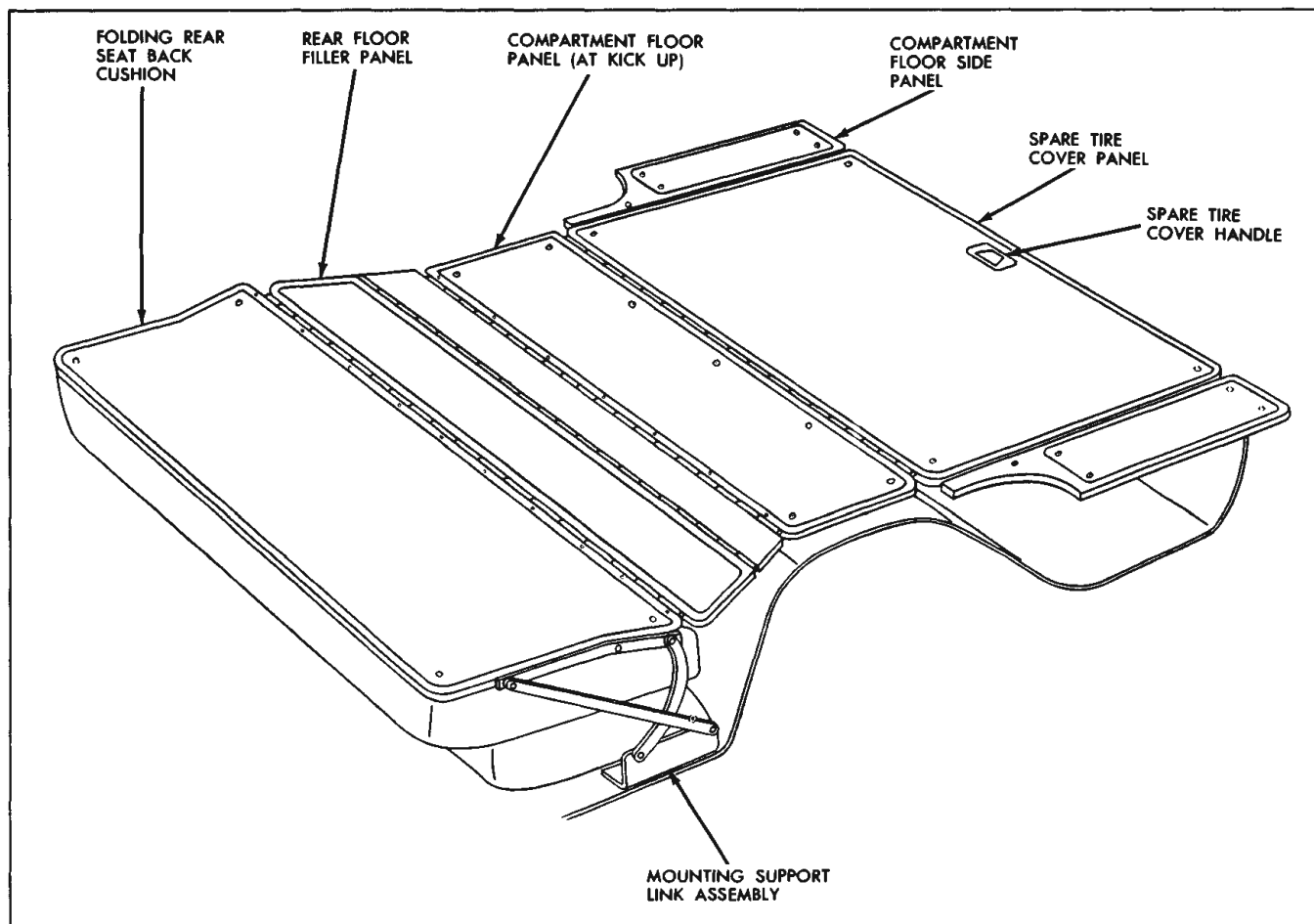
Fig. 18-6 Folding Rear Seat Back and Rear Compartment Floor Panels
