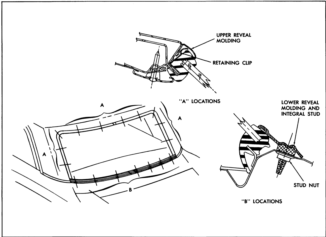
Fig. 15-2 Back Window Reveal Moldings (17 Style)
