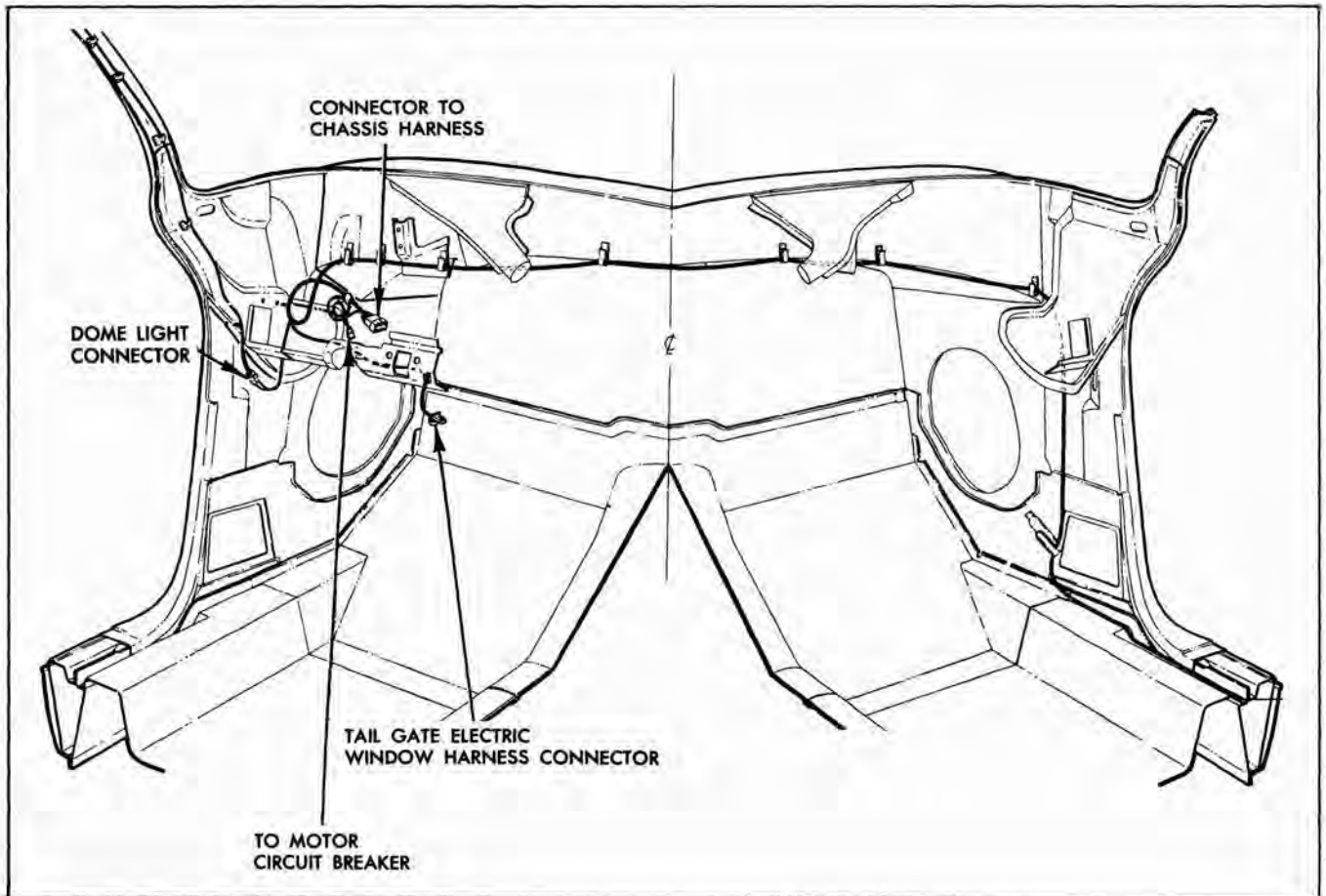
Fig. 9-7 Wiring For Tail Gate
