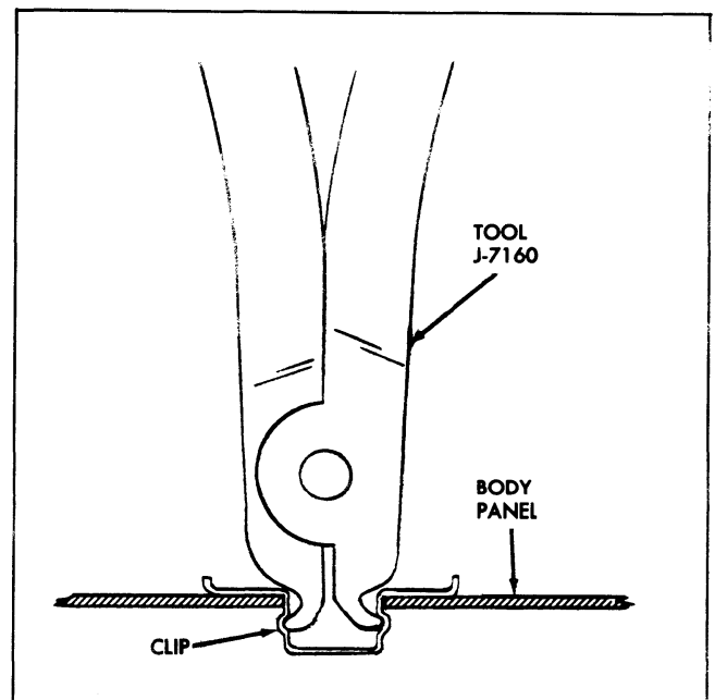
Fig. 16-5 Installing Clip
