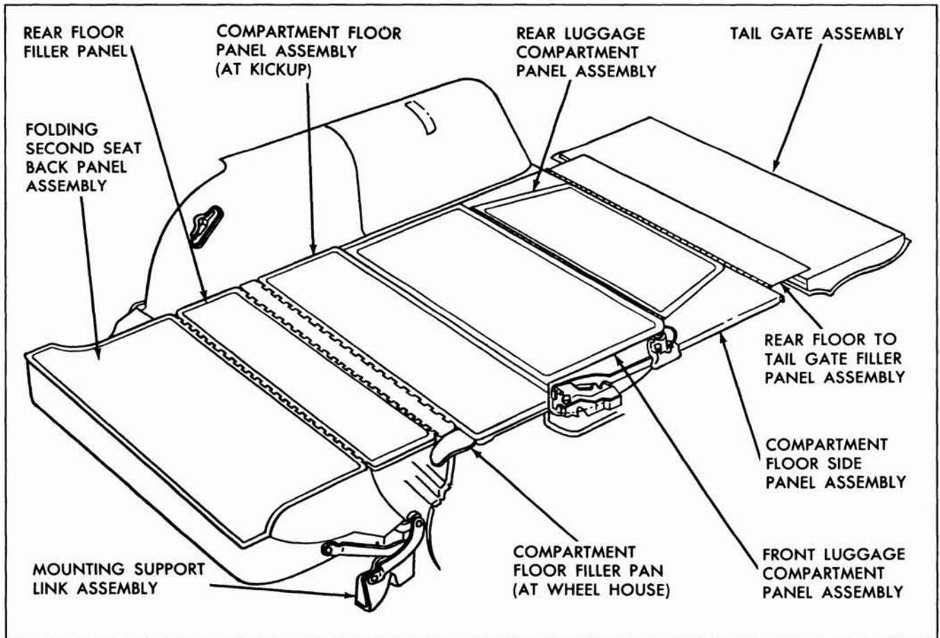
Fig. 8-2 Folding Seat and Rear Compartment Panels - 6 Passenger
