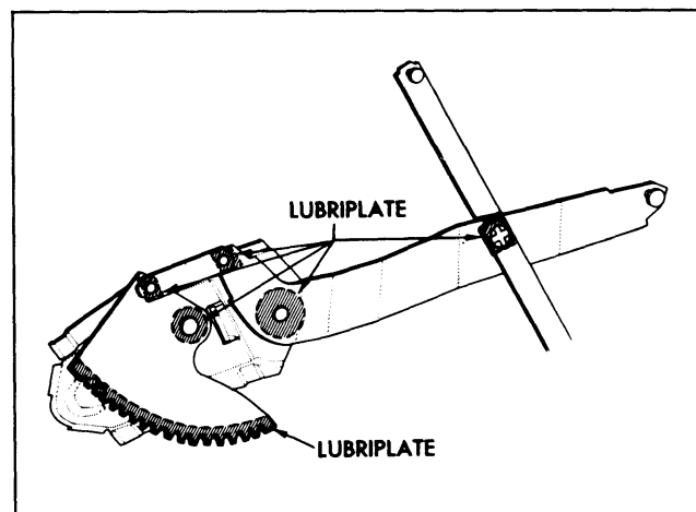
Fig. 20-8 Door Window Regulator
