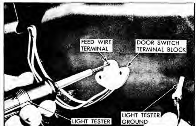
Fig. 9-3 Checking Feed Circuit
