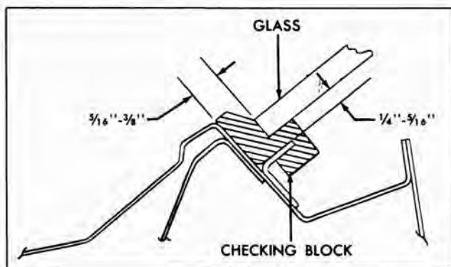
Fig. 2-8 Windshield Opening Checking Block
