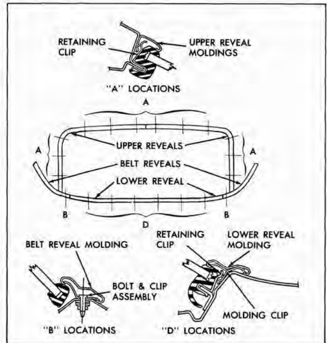
Fig. 5-5 Back Window Reveal Moldings
