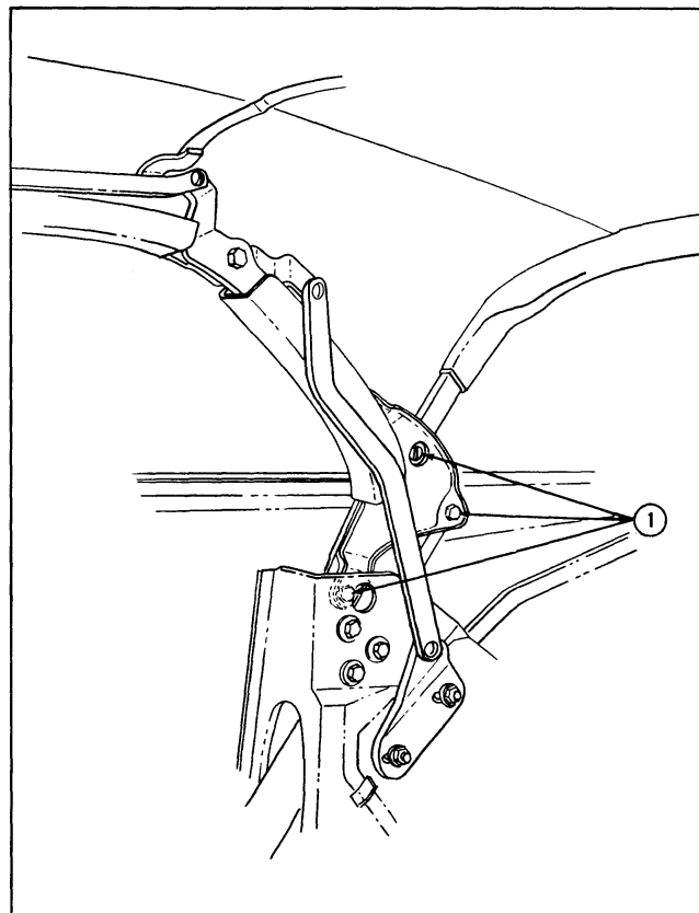
Fig. 20-14 Convertible Top Linkage
