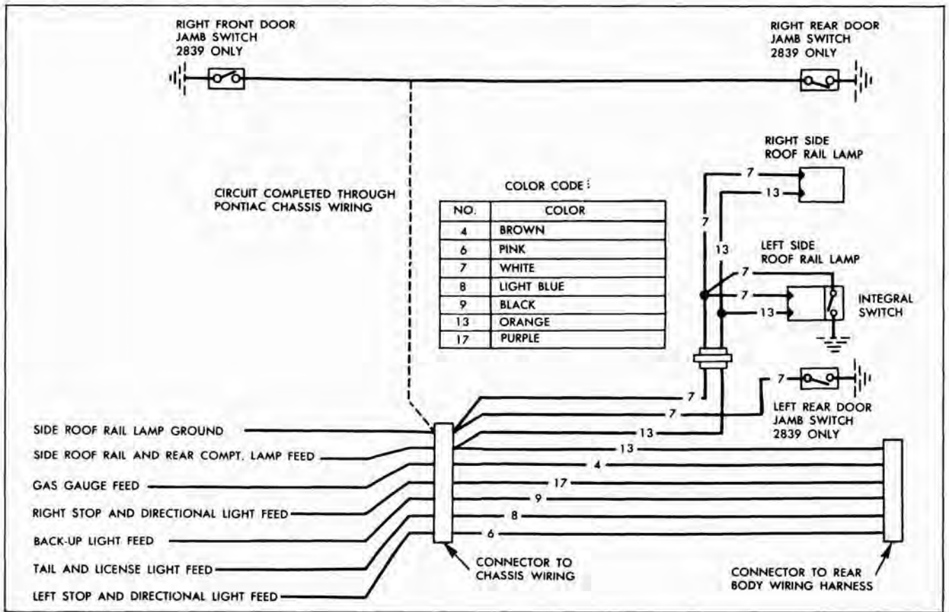
Fig. 9-15 Front Body Wiring Diagram - 2639, 2847, 2839
