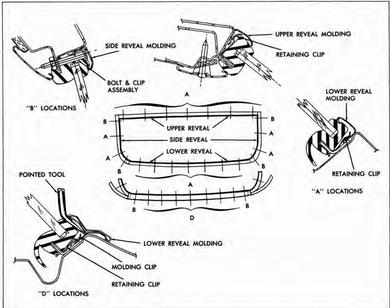
Fig. 5-6 Back Window Reveal Moldings
