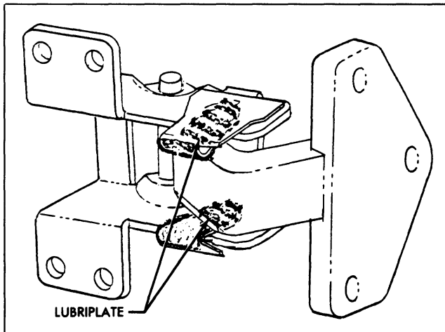
Fig. 20-1 Front Door Hinge and Hold Open
