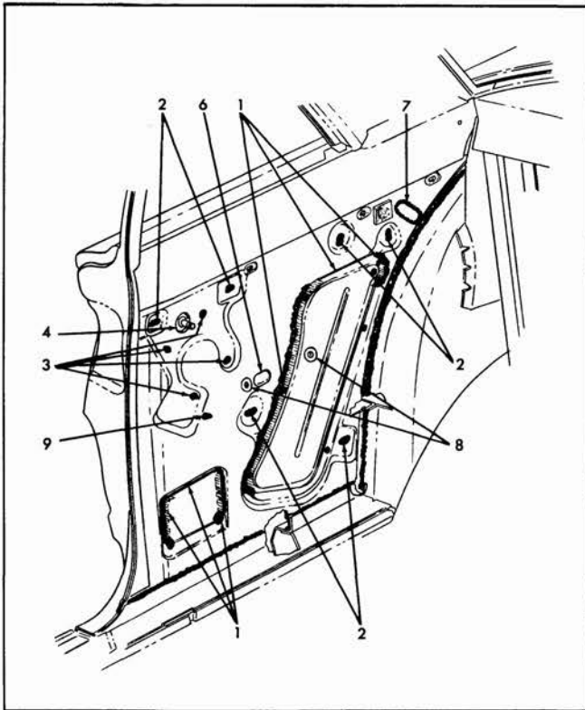
Fig. 14-7 Rear Quarter Sealing "17" and "27" Styles
