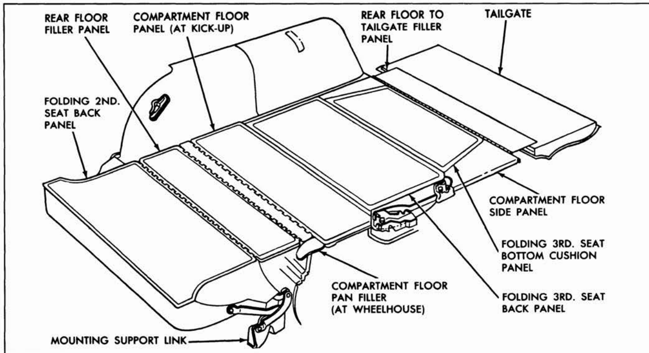
Fig. 8-3 Folding Seat and Rear Compartment Panels - 9 Passenger
