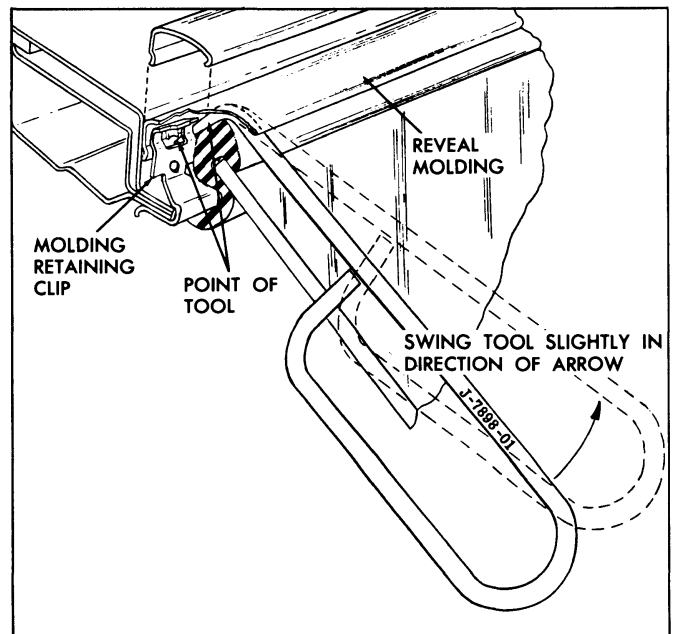
Fig. 15-1 Back Window Reveal Molding Removal Tool
