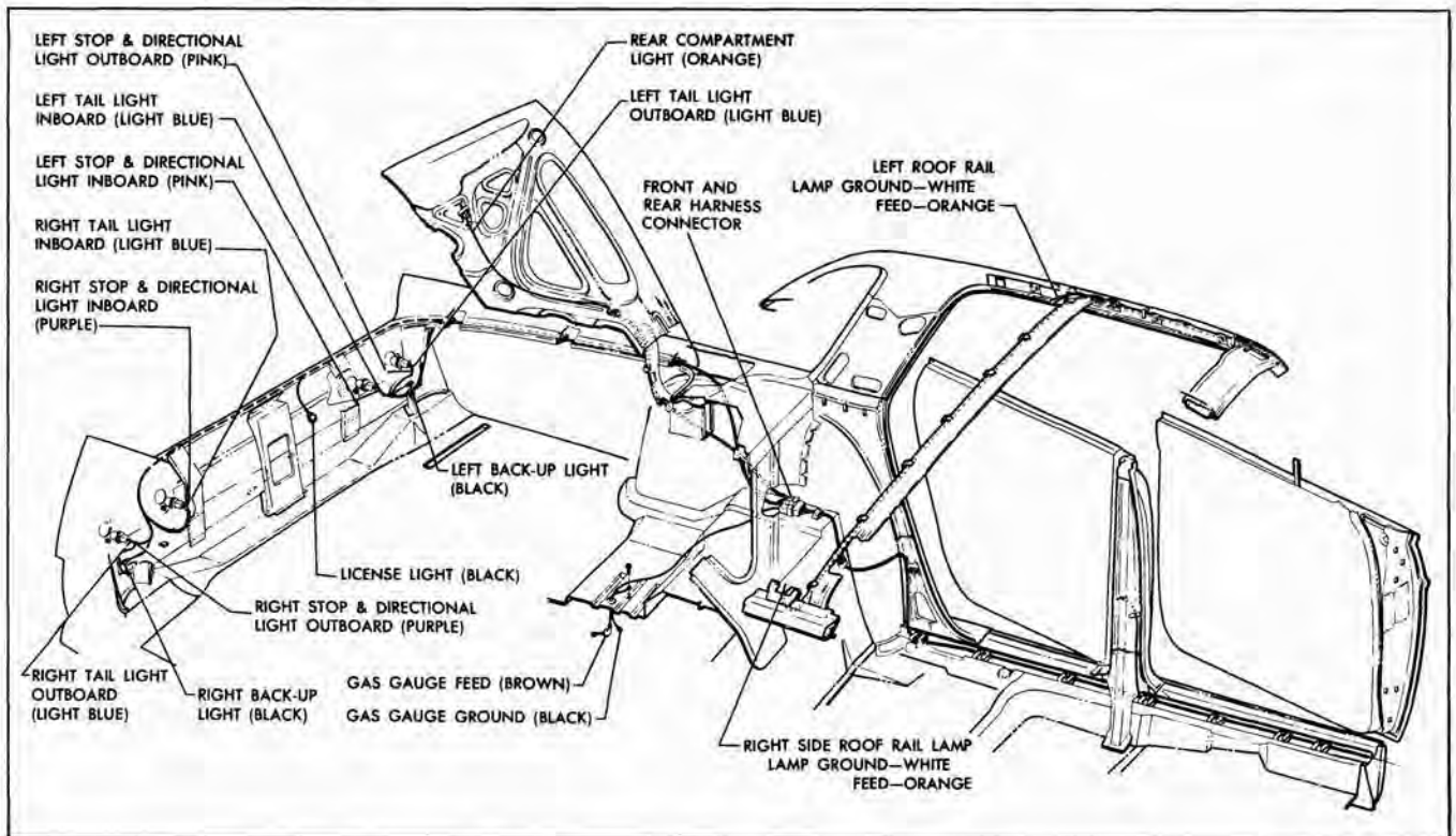
Fig. 9-16 Typical Body Wiring - 2639 Shown
