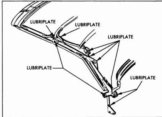
Fig. 10-6 Folding Top Linkage
