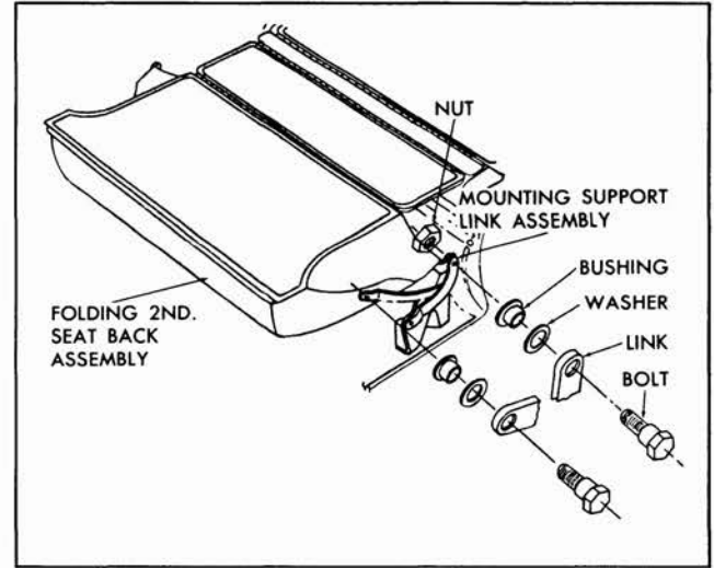
Fig. 8-6 Second Seat Mounting Support Link
