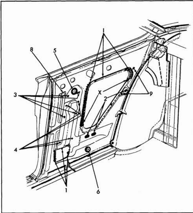
Fig. 4-8 Inner Panel Sealing - "47" Style
