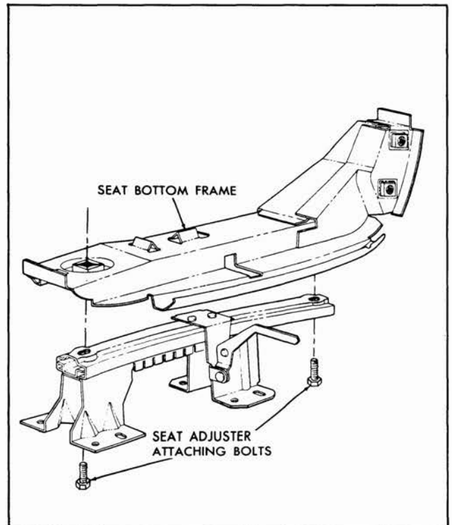
Fig. 8-1 Manual Seat Adjuster
