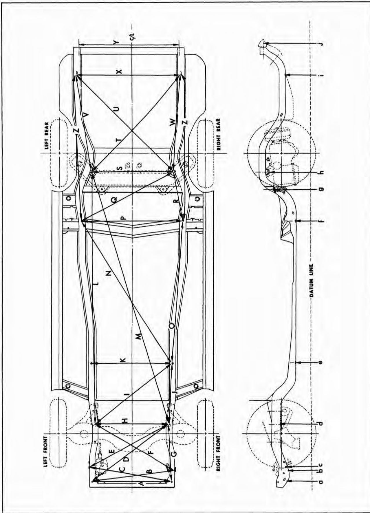
Fig. 12-8 Underbody Dimensions (*Not Symmetrical - See Note, Page 12-7)
