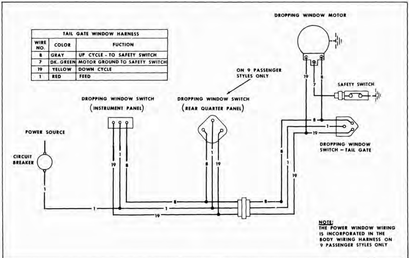
Fig. 9-10 Tail Gate Window Wiring - 9 Passenger
