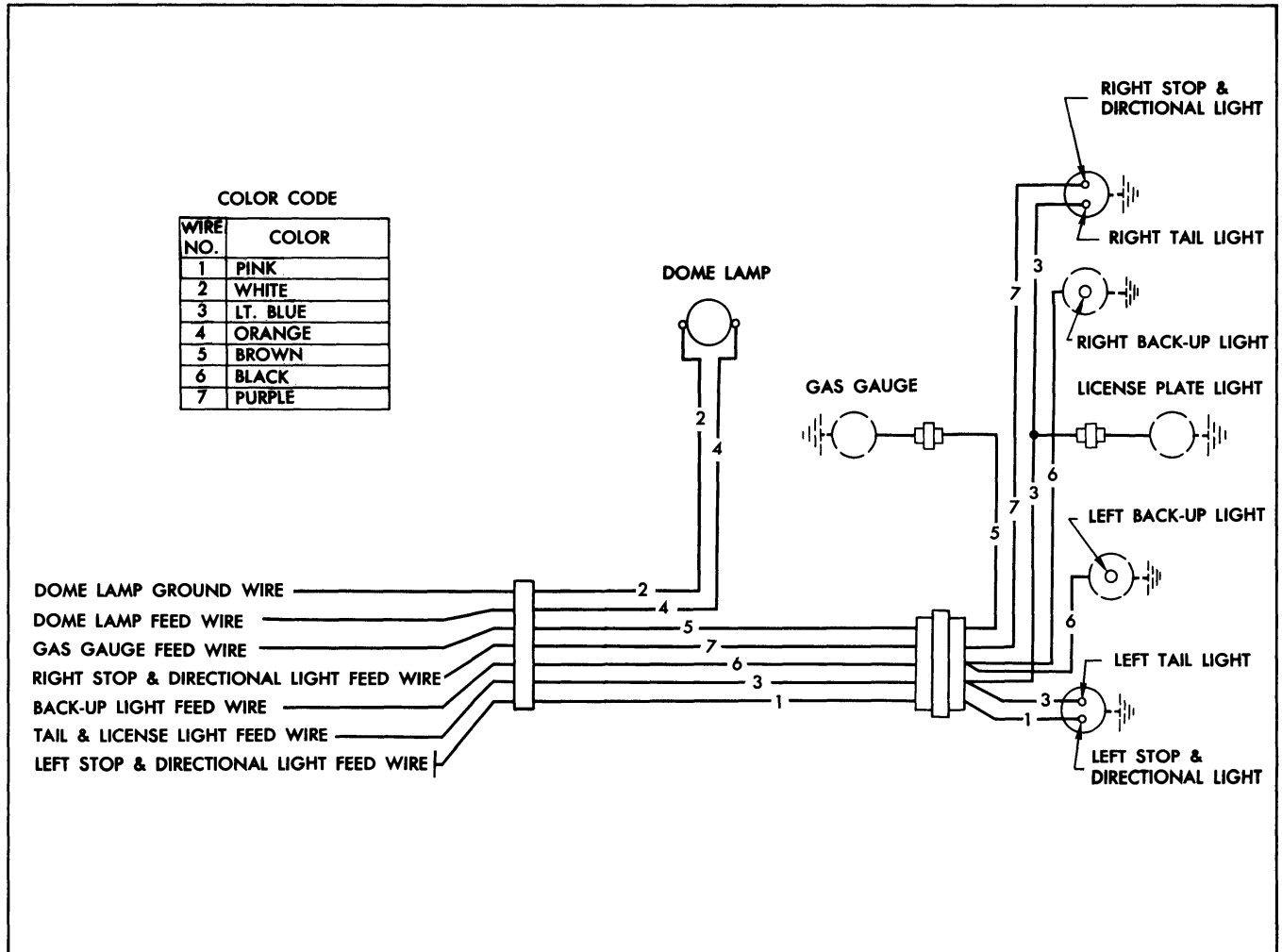
Fig. 19-6 Schematic Body Wiring Circuit Diagram
