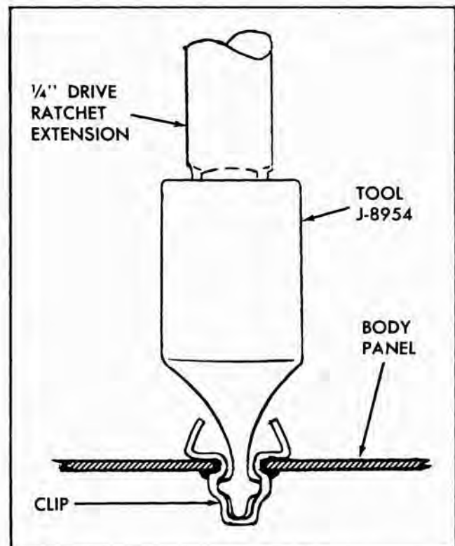
Fig. 6-7 Installing Narrow Bath-Tub Clip
