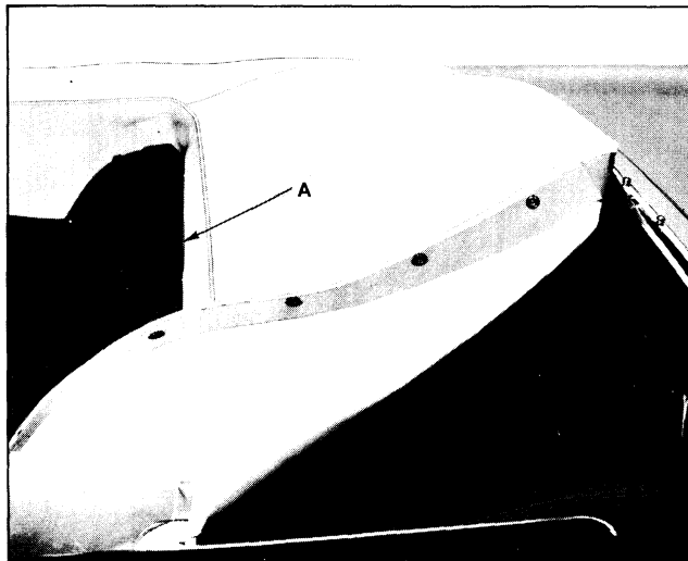
Fig. 22-14 Top Boot Partially Installed
