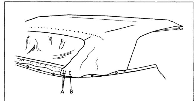
Fig. 22-49 Tacking Top Material
