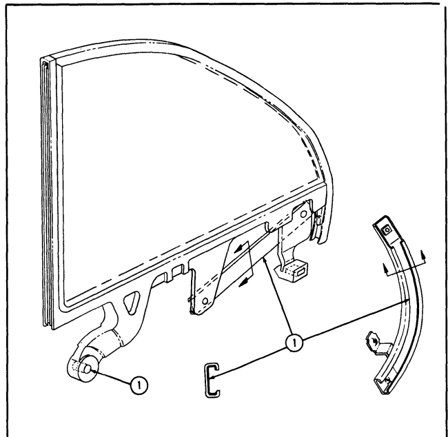
Fig. 20-12 Rear Quarter Window
