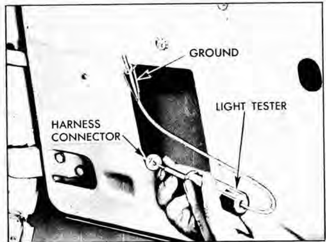
Fig. 9-5 Checking Circuit Between Switch and Motor
