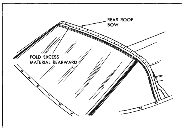
Fig. 22-43 Back Curtain Installation At Rear Roof Bow
