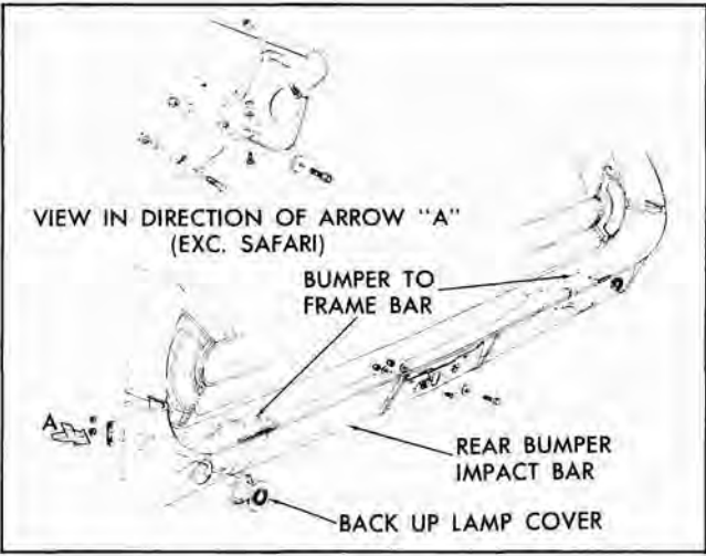
Fig. 1-2 Rear Bumper Assembly
