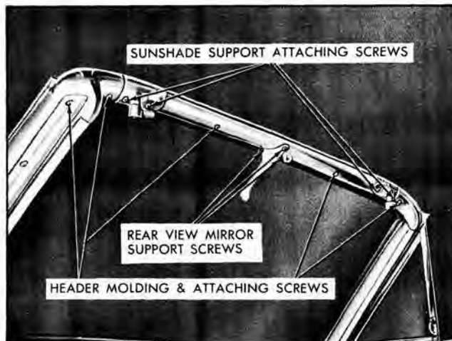
Fig. 12-11 Windshield Header - "67" Style
