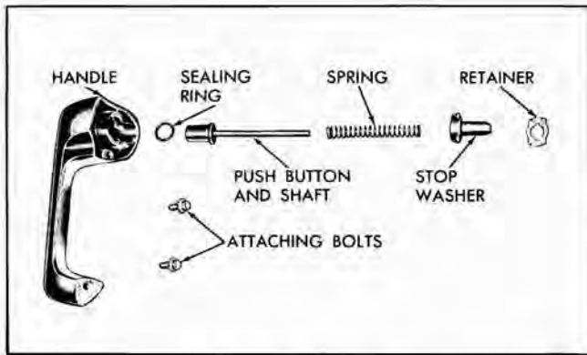
Fig. 13-10 Outside Handle
