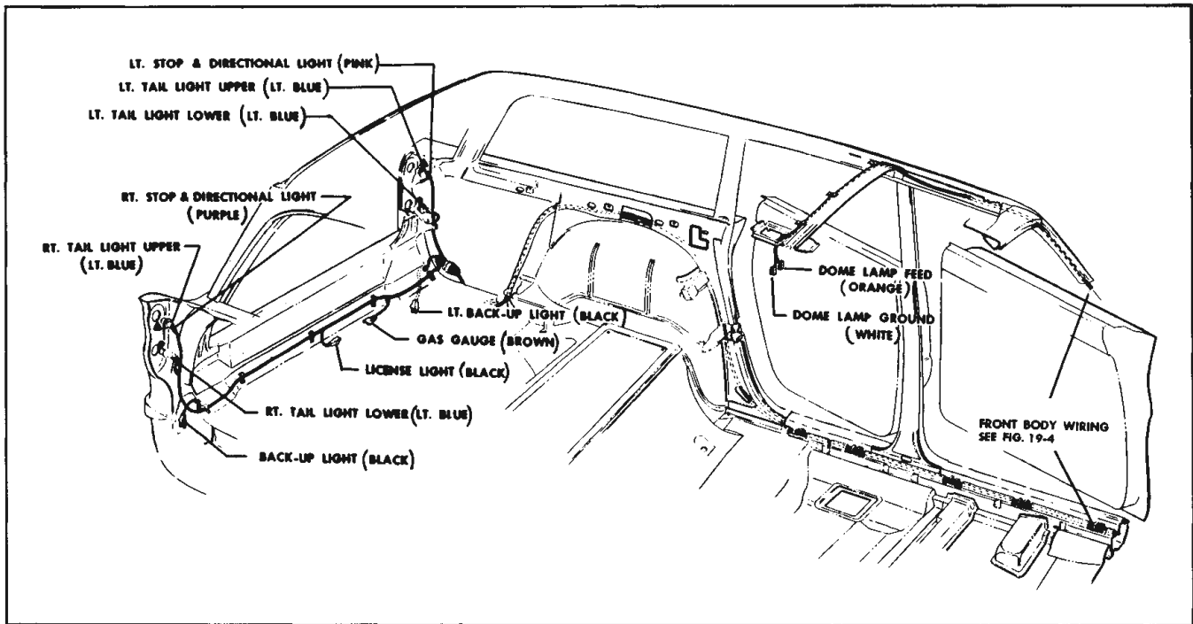
Fig. 19-2 Station Wagon Body Wire Installation
