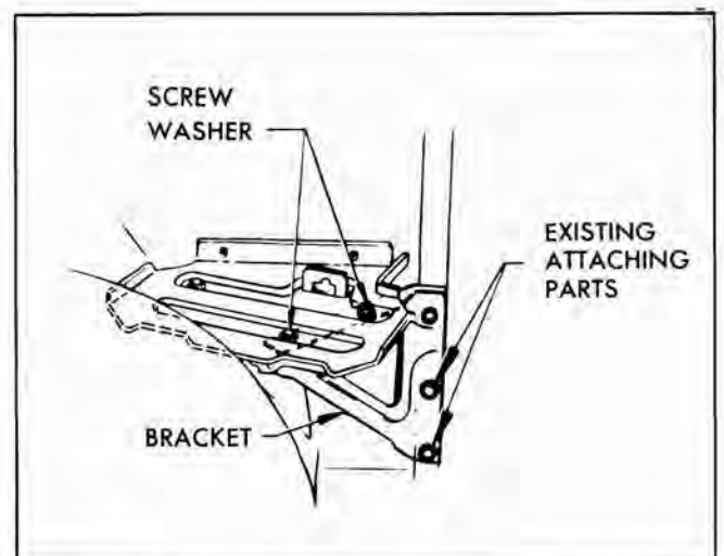
Fig. 1-6 Battery Tray Installation
