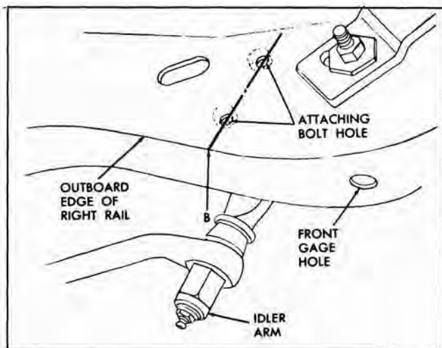
Fig. 12-5 Underbody Vertical Reference Point ("B")
