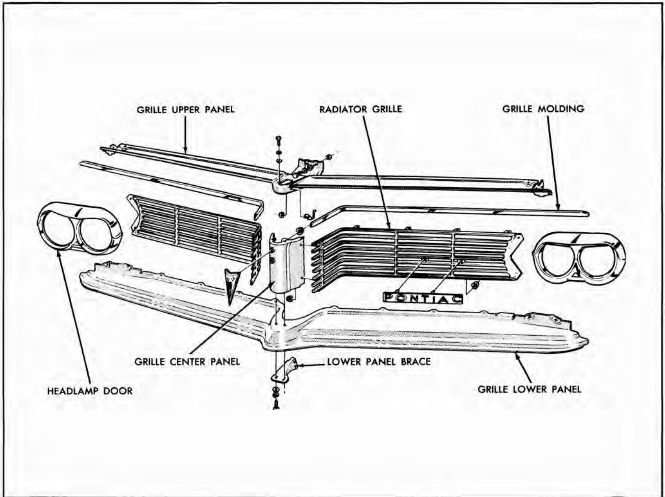
Fig. 1-12 Radiator Grille Assembly
