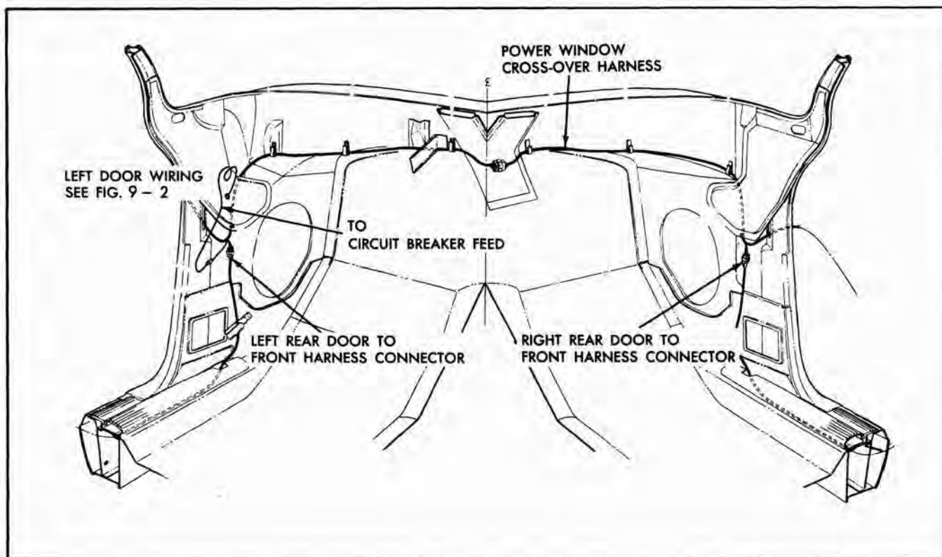
Fig. 9-1 Power Window Wiring Installation
