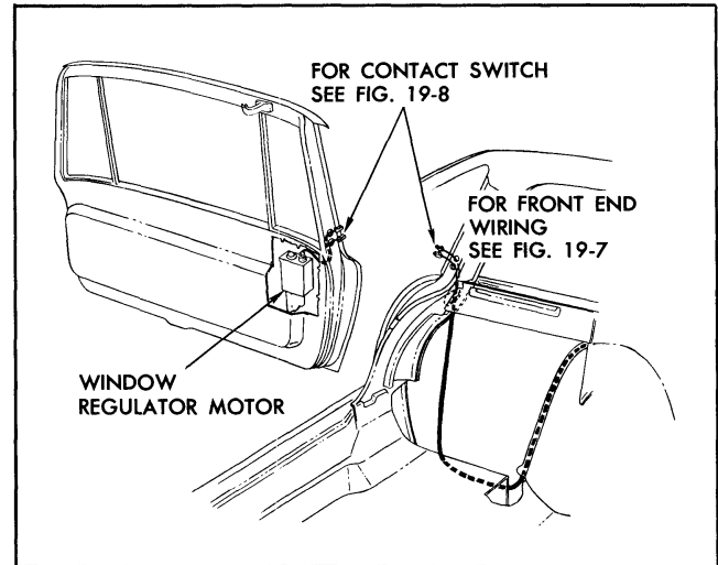
Fig. 19-9 Electric Window - Regulator Wiring
