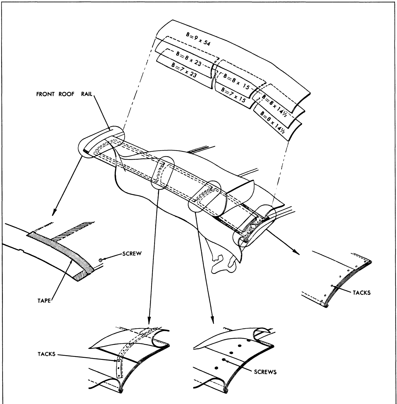
Fig. 22-36 Installation of Side Stay Pads ("B" Styles)
