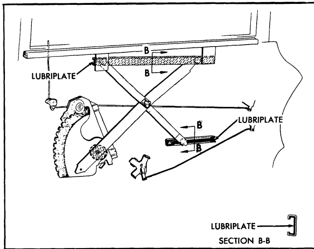
Fig. 20-10 Rear Door Window Regulator Cams
