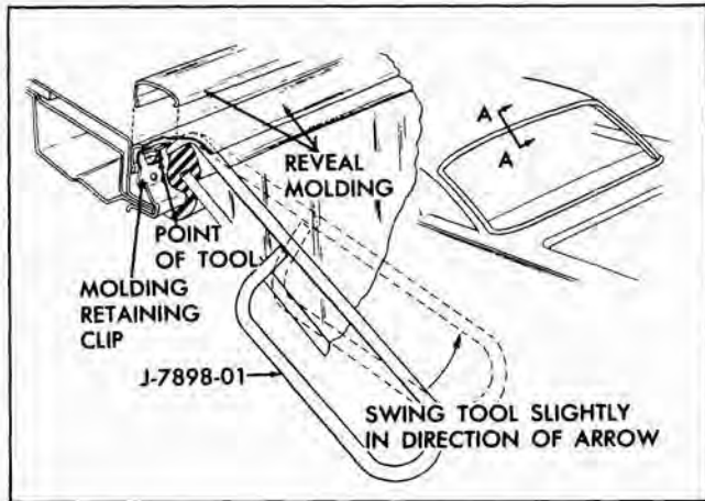
Fig. 5-3 Reveal Molding Removing Tool
