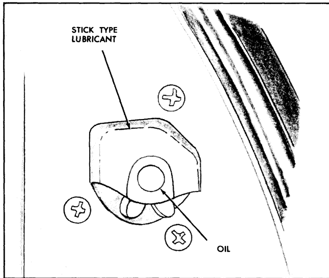
Fig. 20-3 Door Lock Rotary Bolt and Housing
