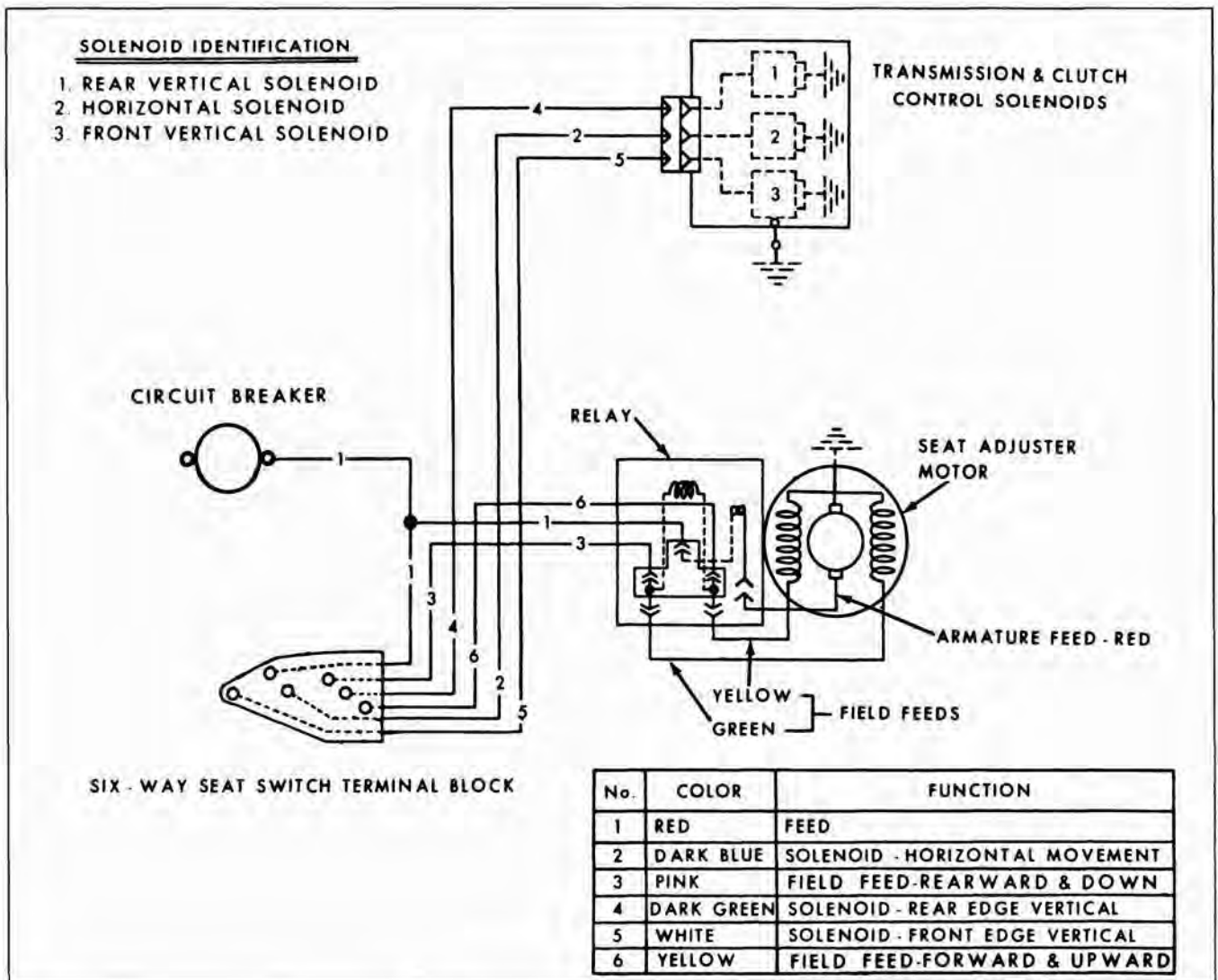
Fig. 9-12 Circuit Diagram - Six-Way Seat
