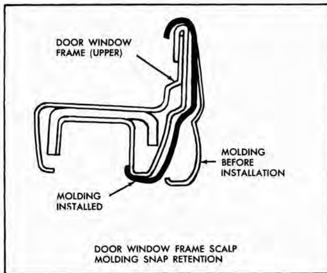
Fig. 6-1 Typical Methods of Molding Attachments
