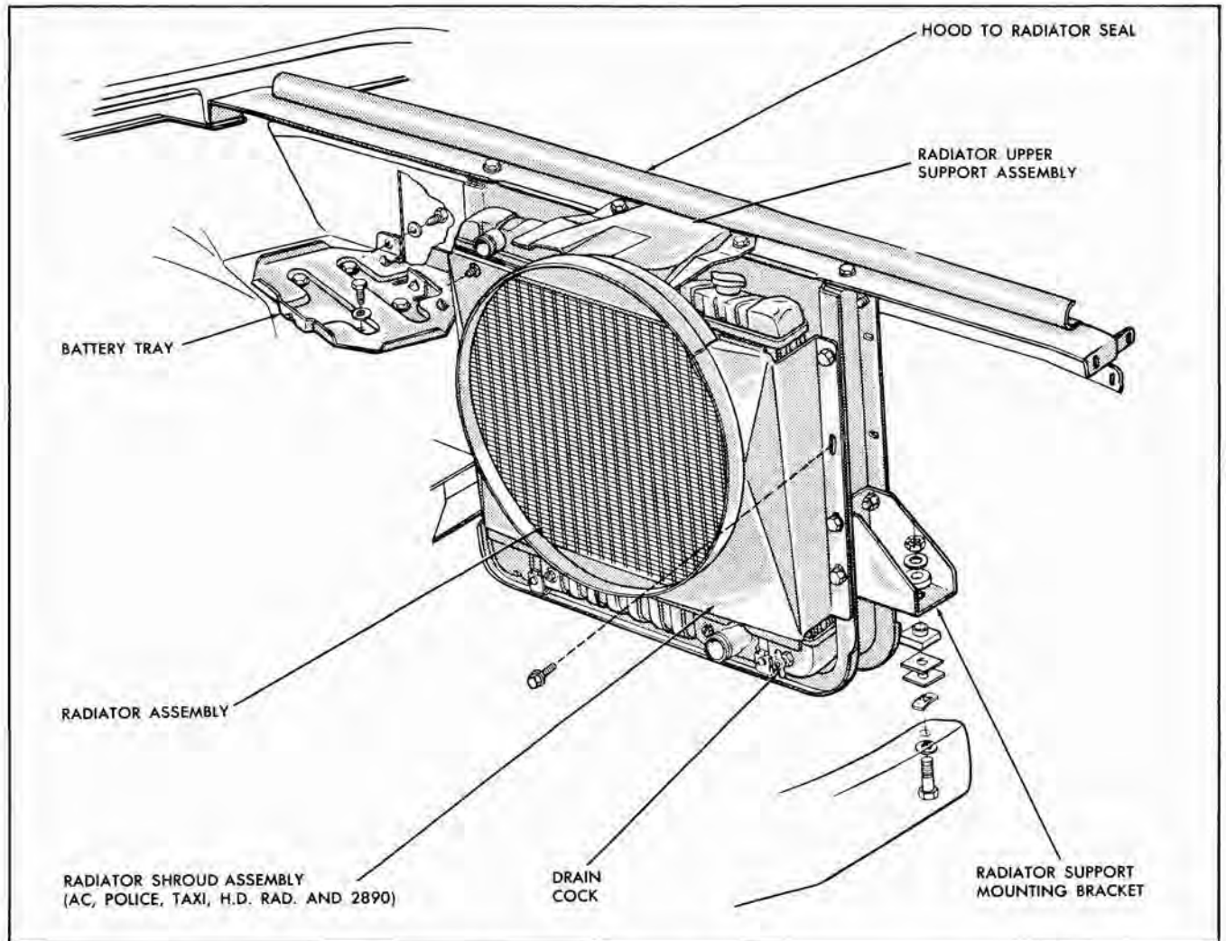
Fig. 1-5 Radiator Assembly Installation
