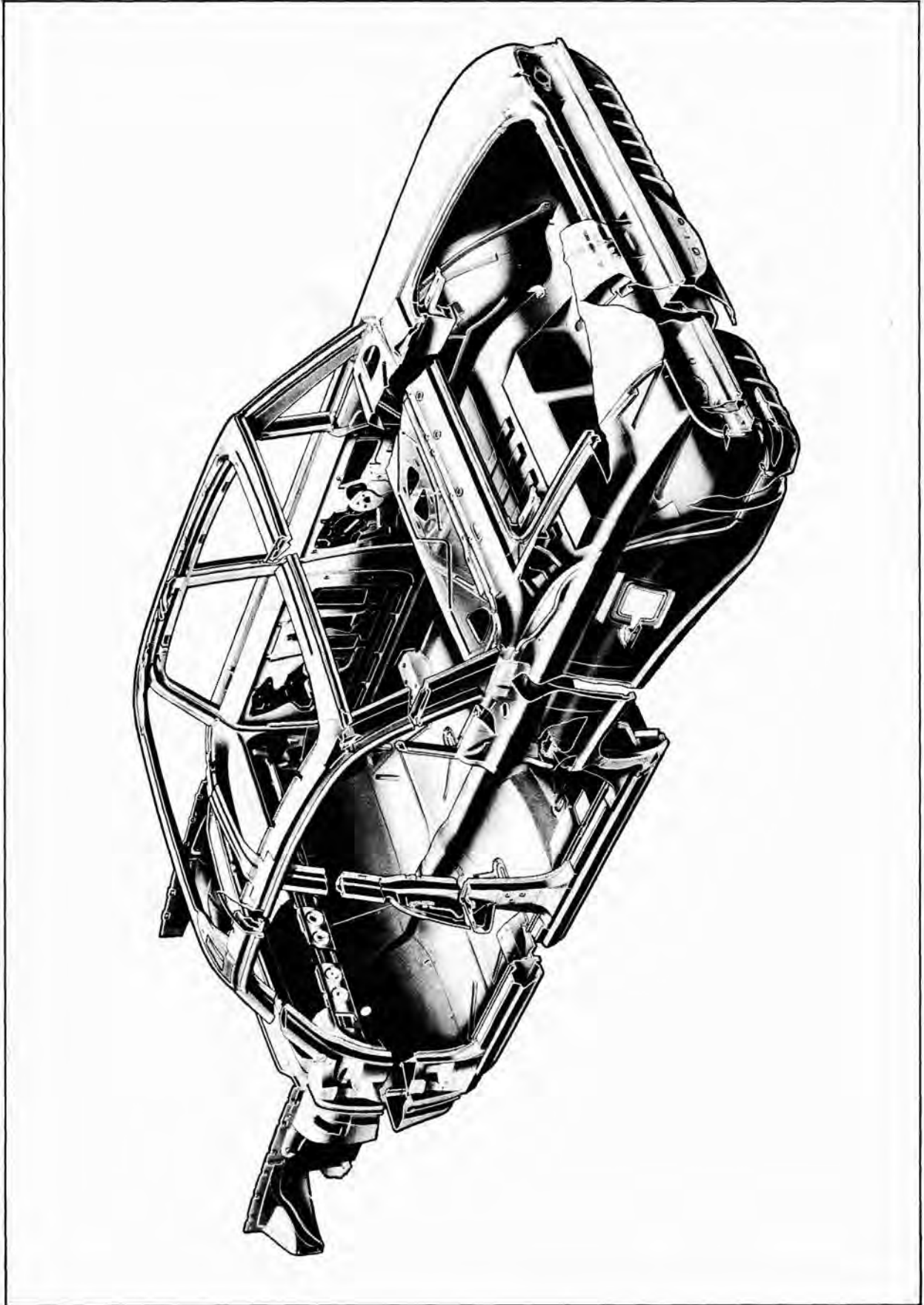
Fig. 12-2 2119 Body Shell Construction
