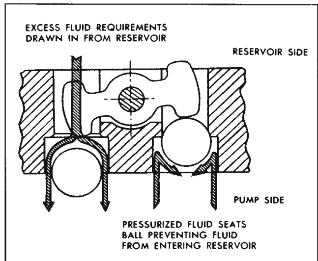
Fig. 22-64 Fluid Control Valve
