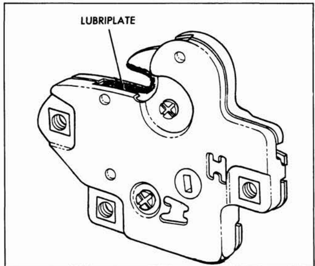
Fig. 10-5 Rear Compartment Lid Lock Bolt
