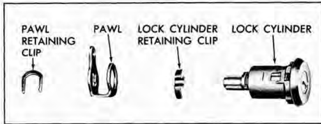
Fig. 3-21 Front Door Lock Cylinder
