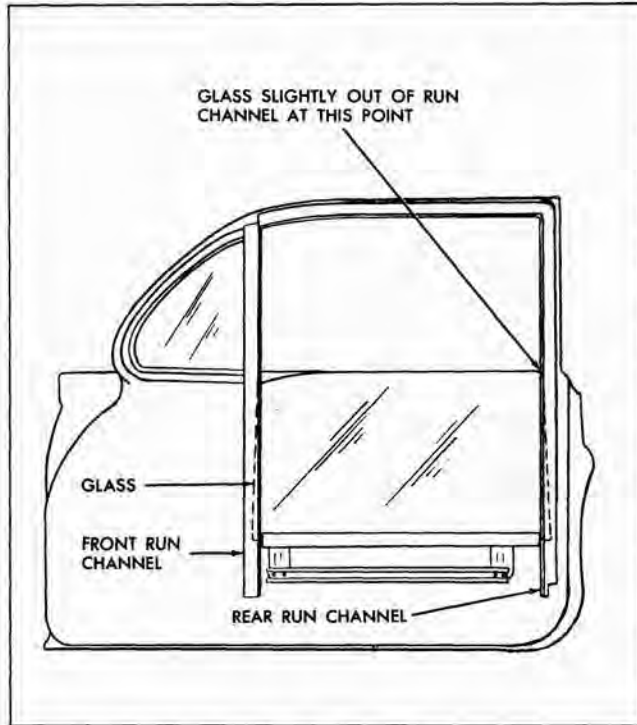
Fig. 3-17 Lowered Front Door Glass
