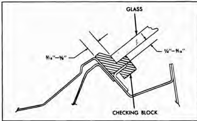
Fig. 12-14 Windshield Opening Check
