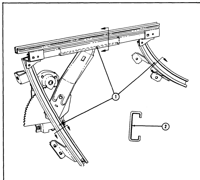
Fig. 20-11 Rear Quarter Window Regulator Cams
