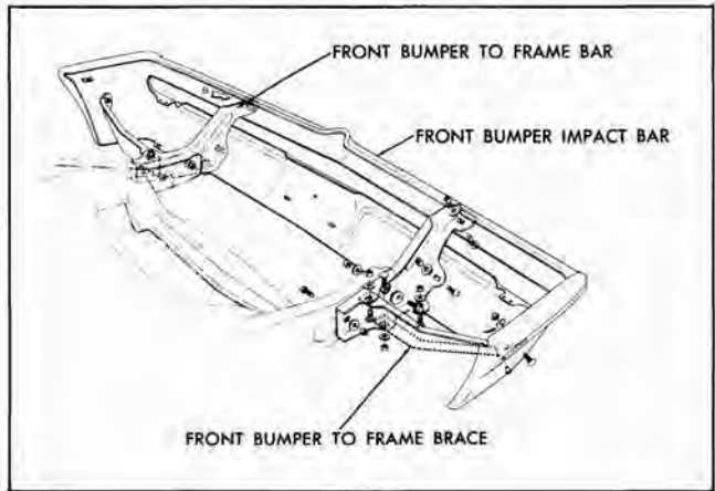
Fig. 1-1 Front Bumper Assembly
