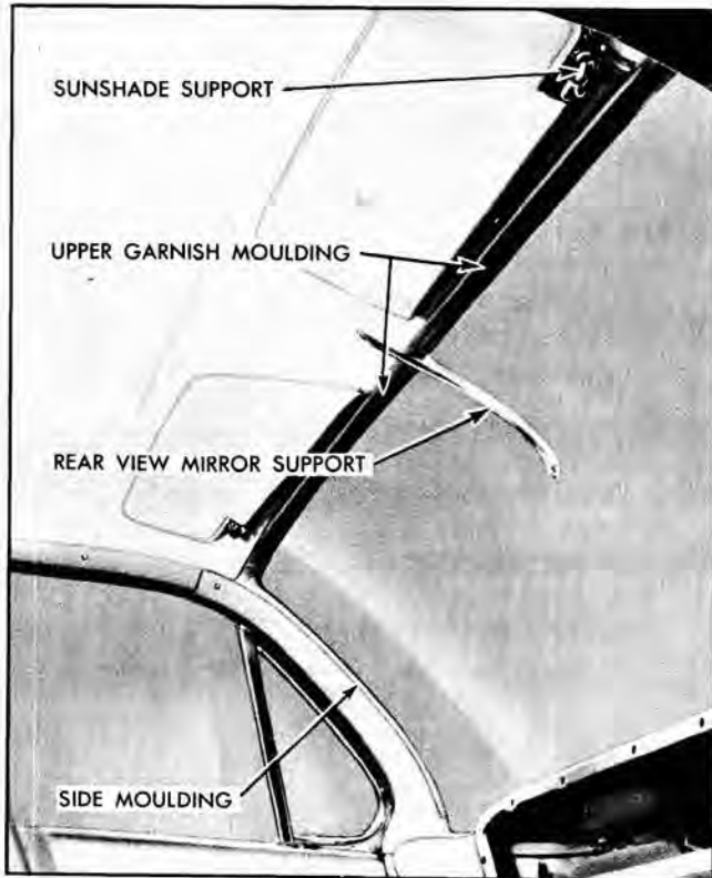
Fig. 2-2 Windshield Garnish Moldings
