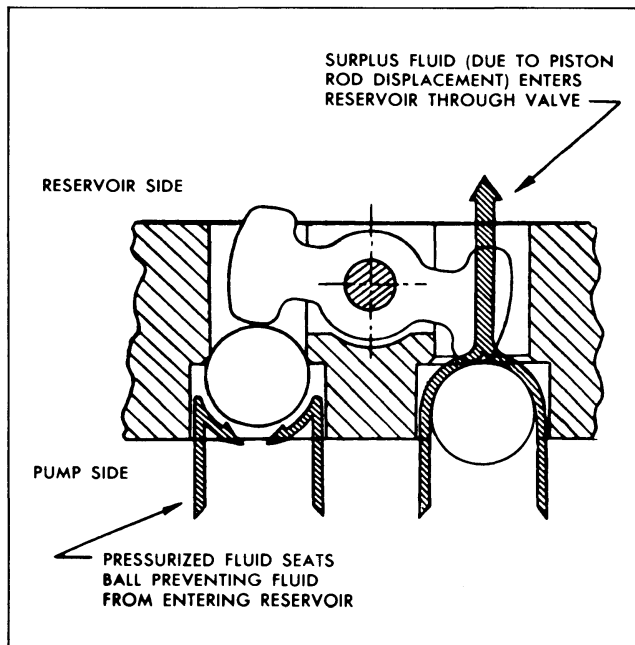
Fig. 22-65 Fluid Control Valve
