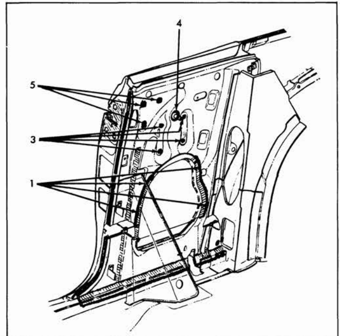
Fig. 14-8 Rear Quarter Sealing "67" Style
