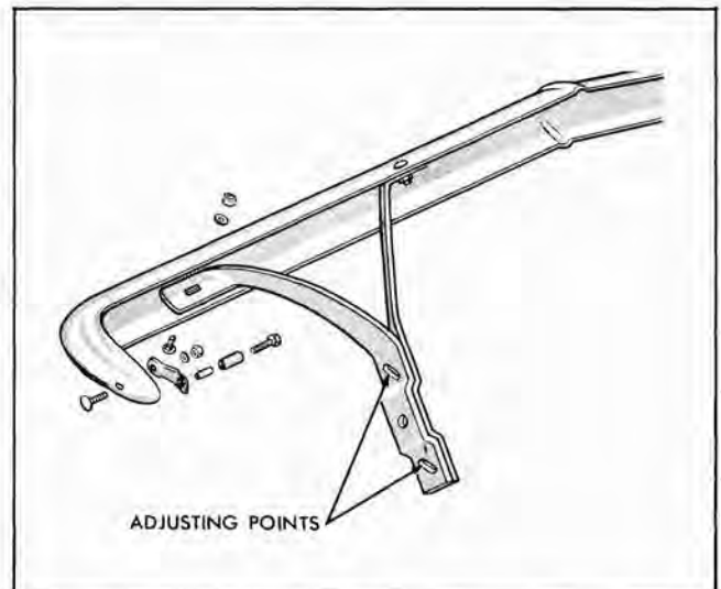
Fig. 11-8 Front Bumper
