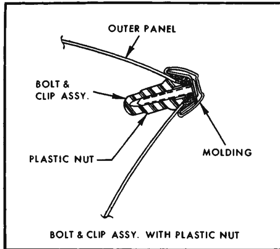
Fig. 16-1 Typical Method For Molding Attachment
