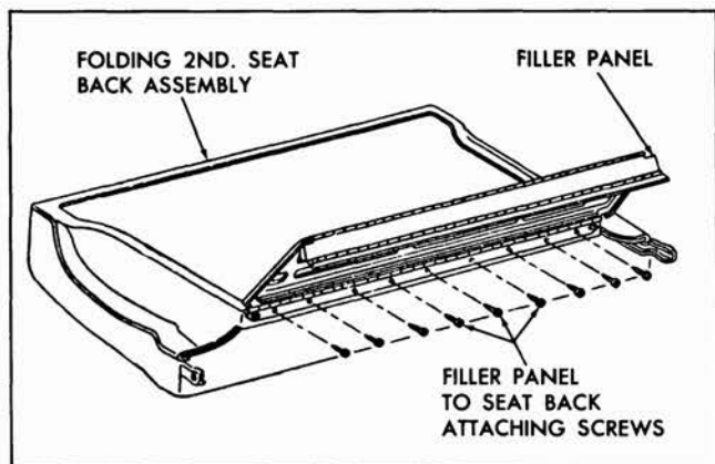
Fig. 8-5 Rear Door Filler Panel
