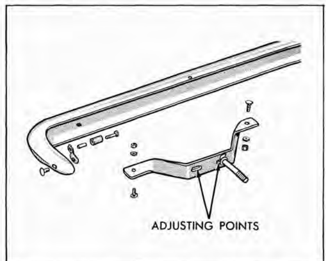
Fig. 11-9 Rear Bumper
