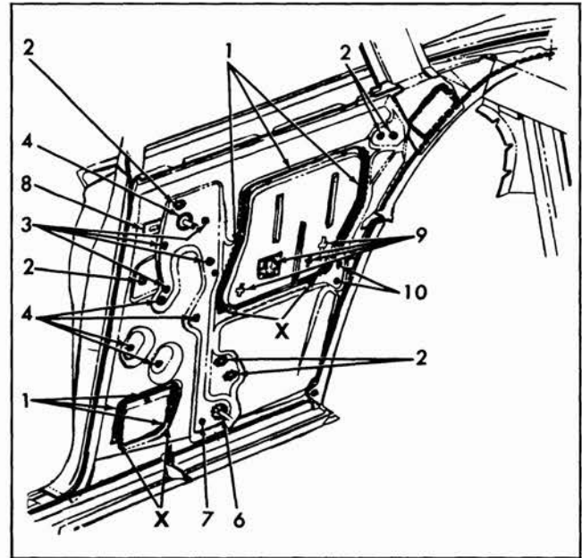
Fig. 4-7 Inner Panel Sealing - "11" Style
