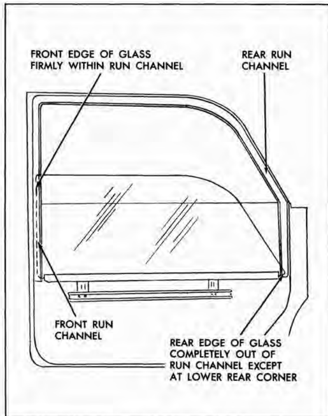
Fig. 3-32 Lowered Rear Door Glass
