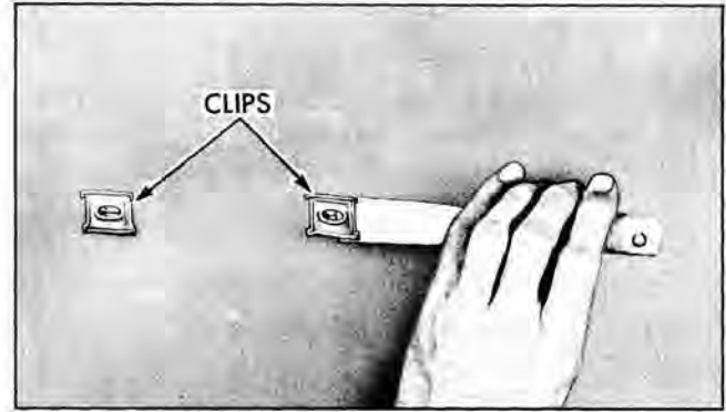
Fig. 6-6 Removing Bath-Tub Type Clip
