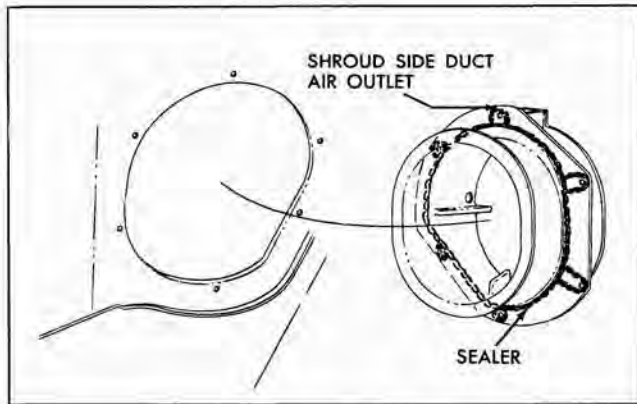
Fig. 2-14 Shroud Side Duct Air Outlet
