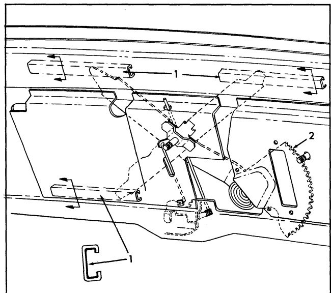
Fig. 20-13 Back Door Window Regulator Cams
