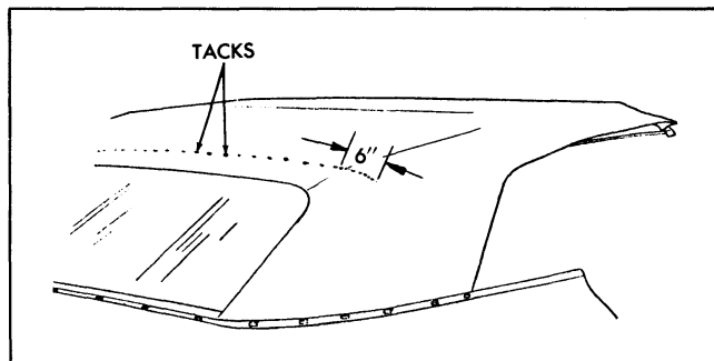
Fig. 22-51 Tacks Outboard of Seams
