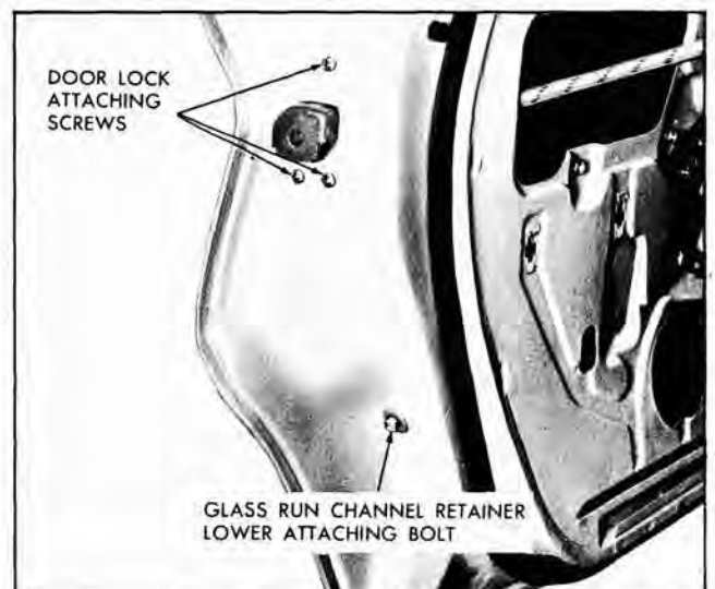
Fig. 13-27 Door Lock and Run Channel Attachments
