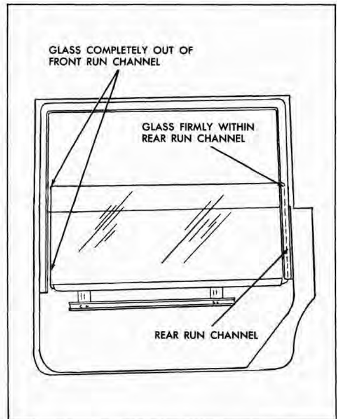
Fig. 3-33 Lowered Rear Door Glass (Sta. Wgn.)
