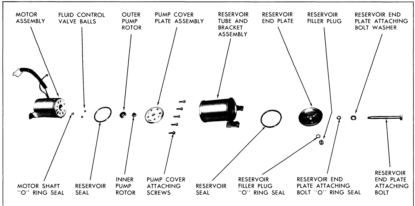
Fig. 22-59 Hydro-Lectric Motor and Pump Assembly-Exploded
