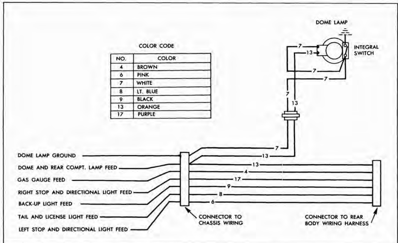
Fig. 9-14 Front Body Wiring Diagram - 2669, All 23 Series Except Wagons
