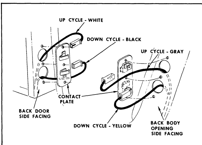
Fig. 19-8 Electric Window Connectors
