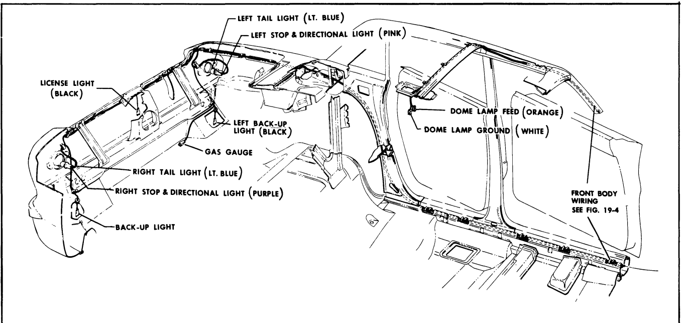
Fig. 19-1 Sedan Body Wire Installation
