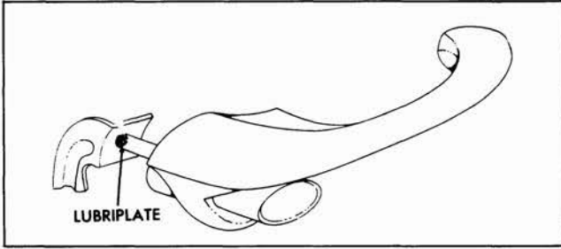
Fig. 10-8 Door Outside Handle
