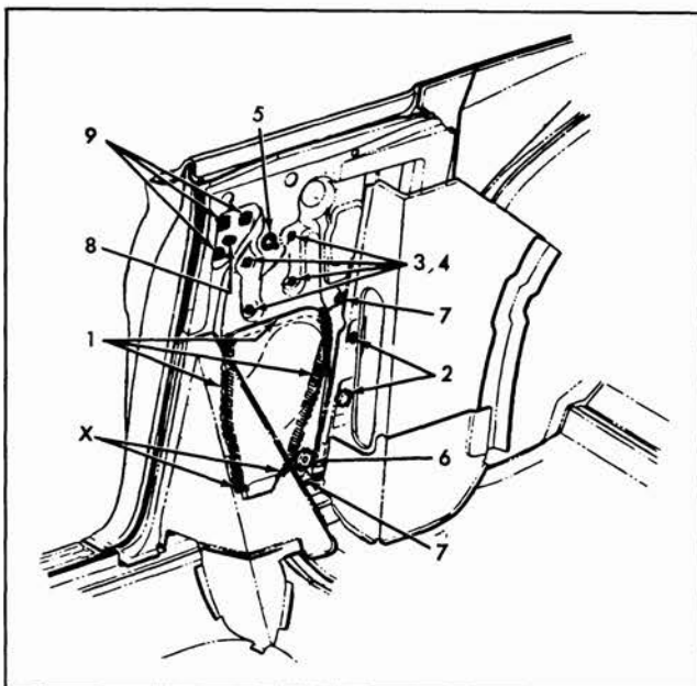
Fig. 4-9 Inner Panel Sealing - "67" Style
