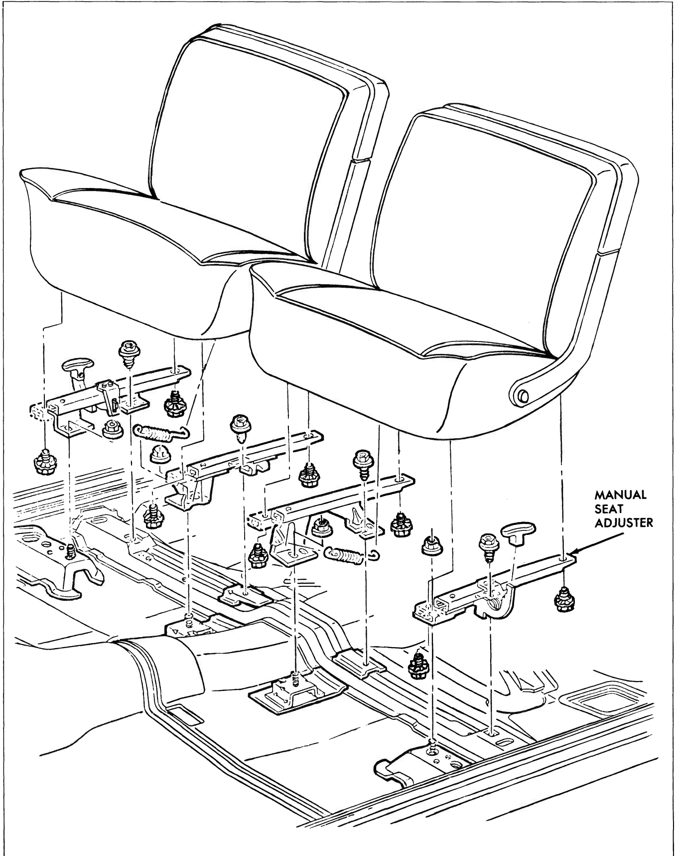
Fig. 23-2 Bucket Seat Assemblies - Typical all Adjustable Right Side
