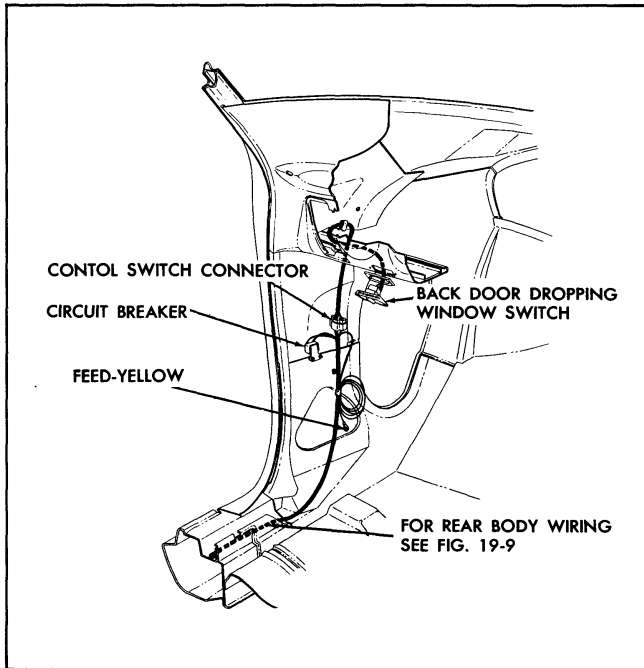
Fig. 19-7 Body Wiring - Electric Back Window
