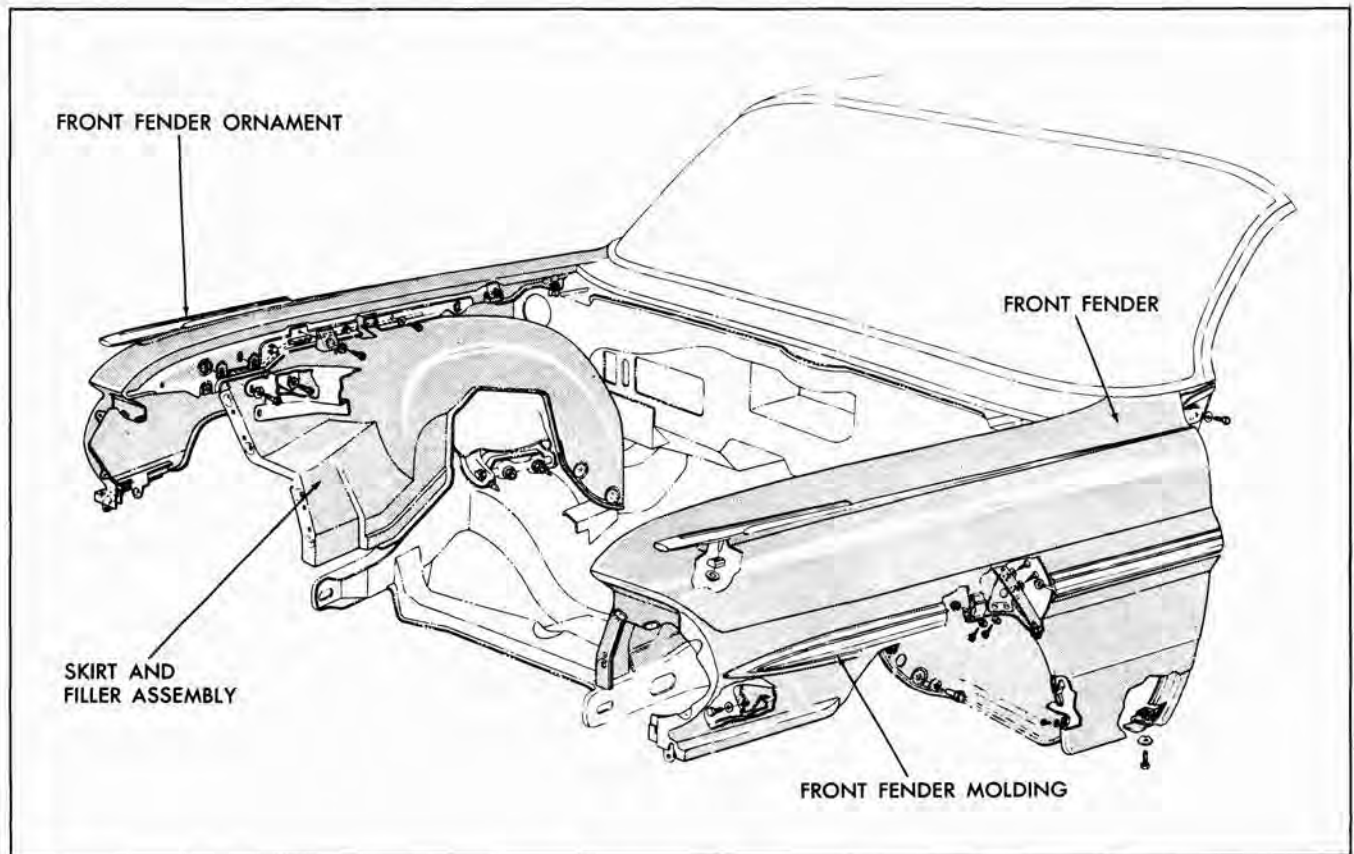
Fig. 1-8 Front Fenders Installation
