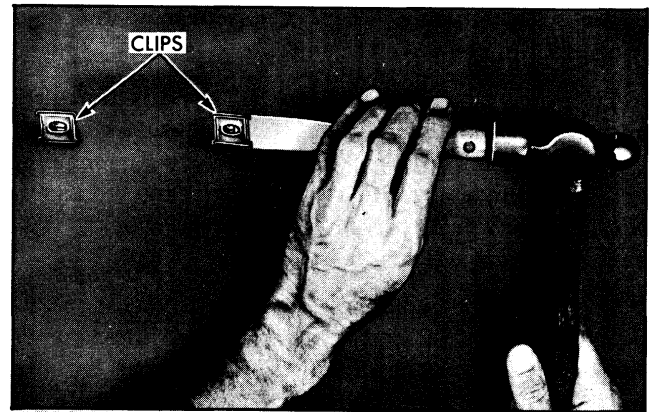
Fig. 16-4 Removing Clip
