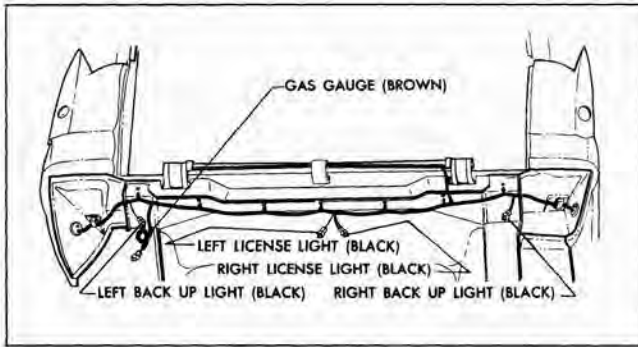
Fig. 9-9 Rear End Wiring (Sta. Wgn.)
