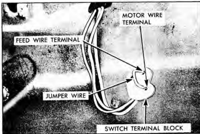
Fig. 9-4 Checking Window Control Switch
