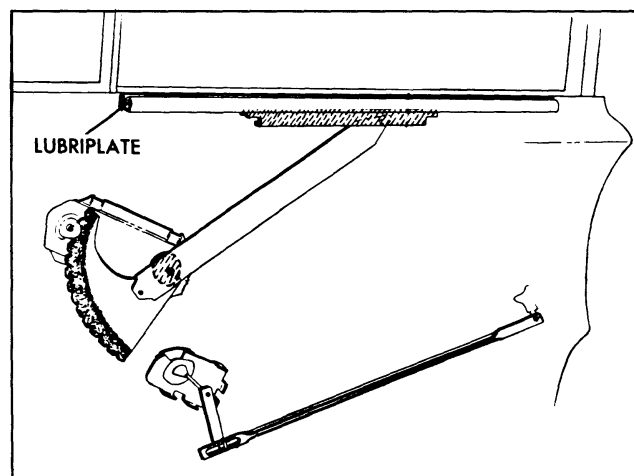
Fig. 20-9 Front Door Window Regulator Cams
