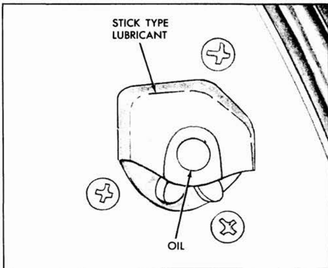
Fig. 10-3 Door Lock Rotary Bolt and Housing
