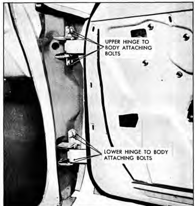
Fig. 13-13 Front Door Hinge Attachments
