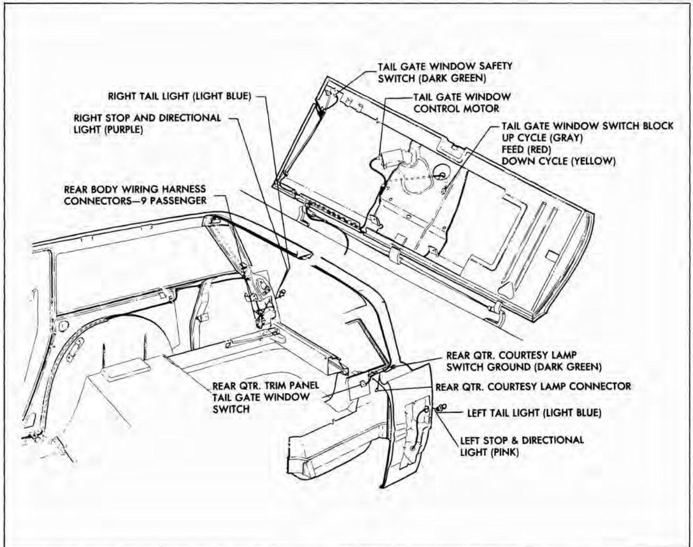
Fig. 9-8 Wiring For Tail Gate
