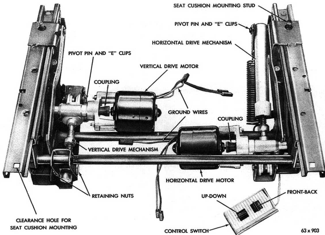
Fig. 20 - Seat Track and Rails Assembly
