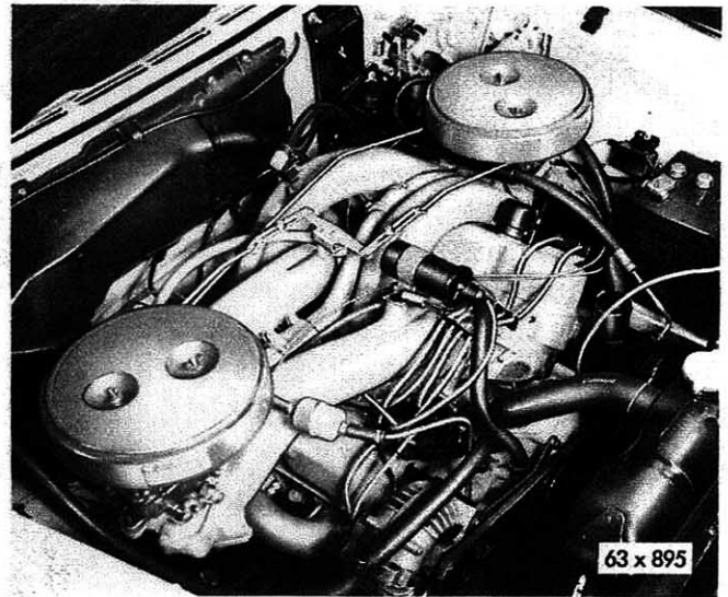
Fig. 8 - Carburetor Air Cleaner Installed
