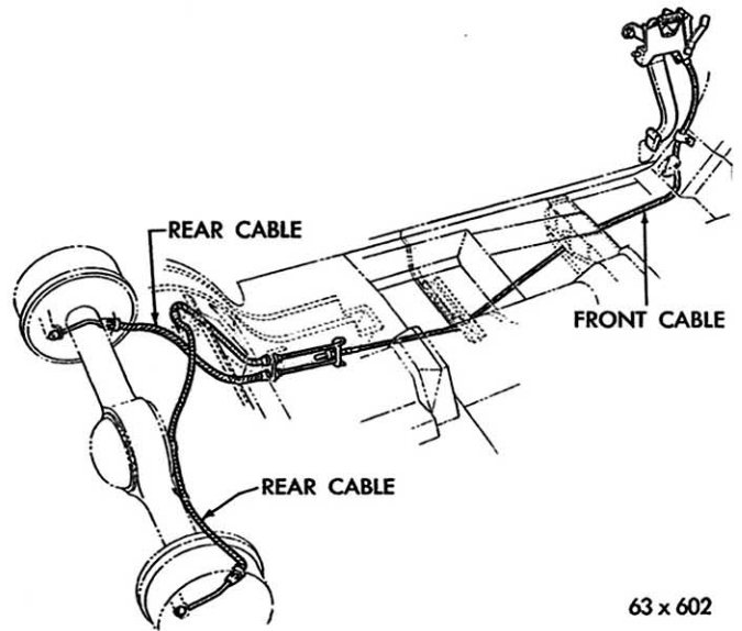
Fig. 3 - Rear Wheel Parking Brakes
