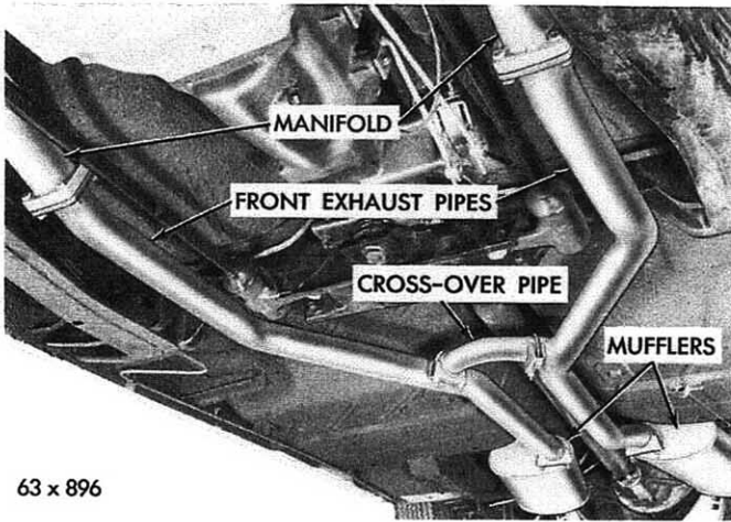
Fig. 9 - Exhaust System
