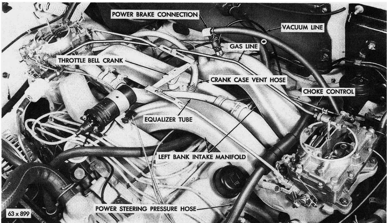
Fig. 15 - Fuel Induction Intake Manifolds
