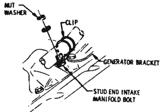
CLIP FASTENING WITHOUT AIR CONDITIONING
