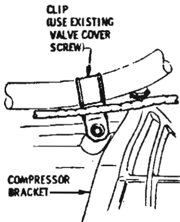
CLIP FASTENING WITH AIR CONDITIONING
