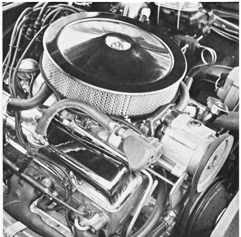
The high rev 302-cubic-inch Chevy features include a Holley four-barrel carburetor, high-winding mechanical lifters, special cam and aluminum inlet manifold.
