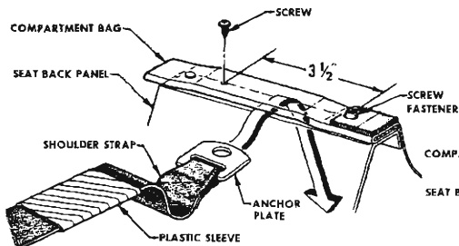
VIEW A
