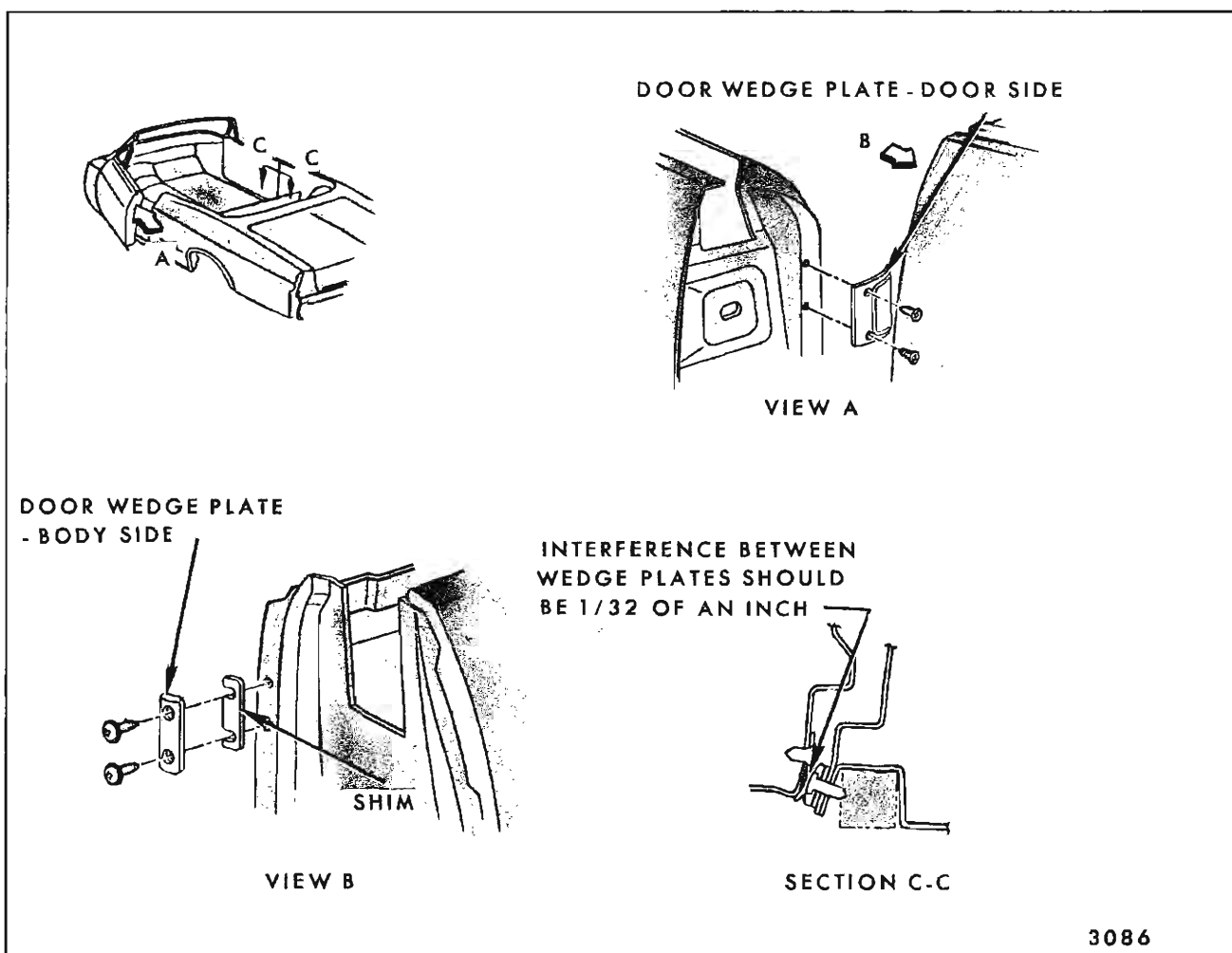
Fig. 6-104—Door Wedge Plates "67" Styles
