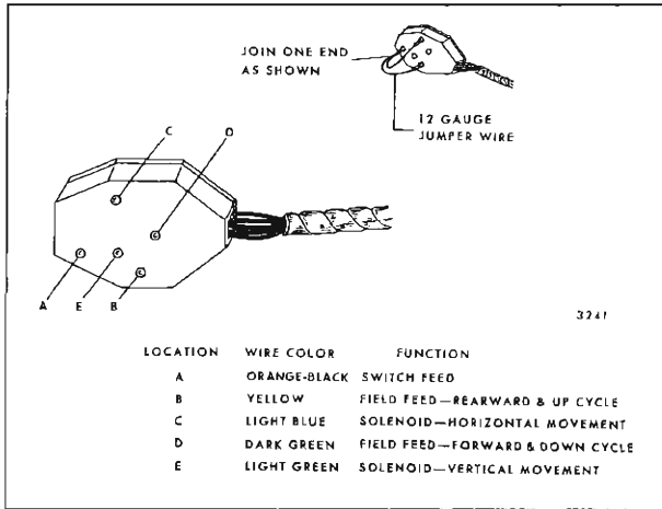
Fig. 16-33—Four-Way Seat Switch Block in Arm Rest
