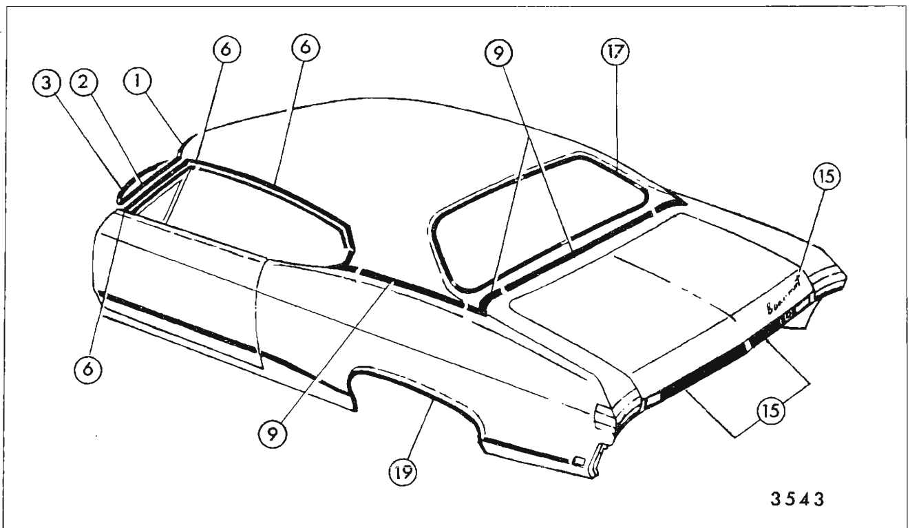
Fig. 17-104—Beaumont 73637 (Canadian)
