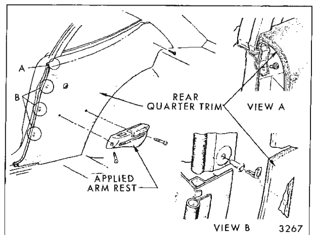
Fig. 14-18—Applied-Type Quarter Arm Rest and Trim Assembly
