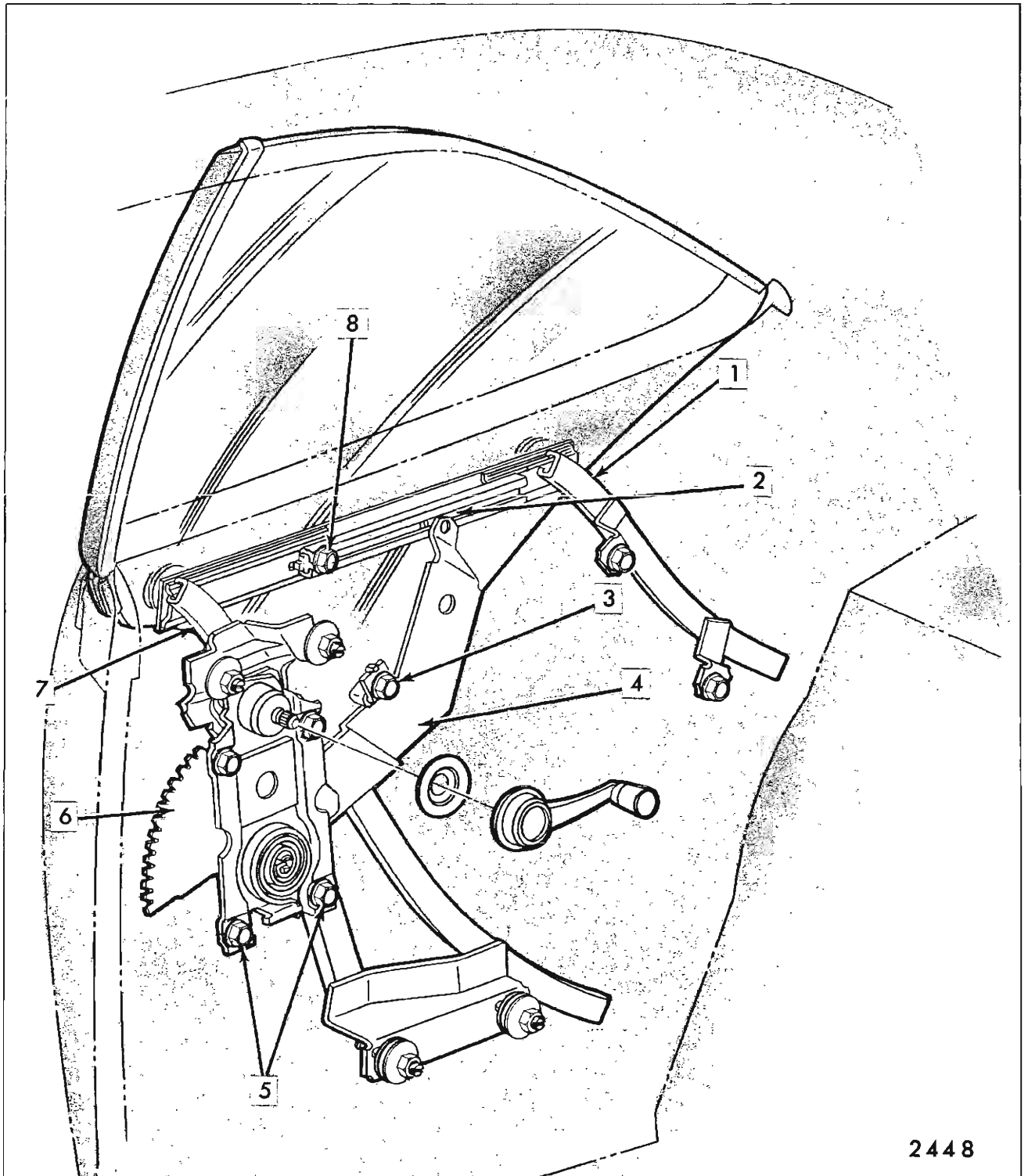
Fig. 7-37—Rear Quarter Hardware - "Z-37" Style
