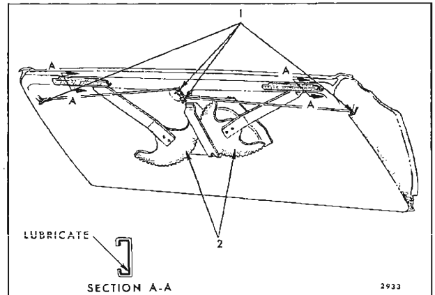
Fig. 2-14—Tailgate Window Regulator, Cams, etc. - All Tailgates
