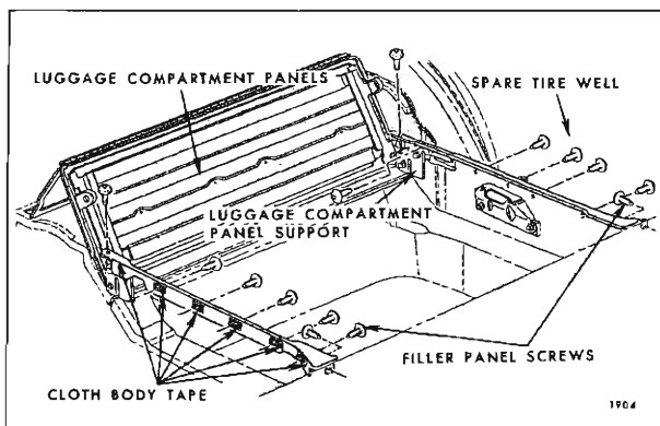
Fig. 15-70—Rear Compartment Pan Side Filler Panels
