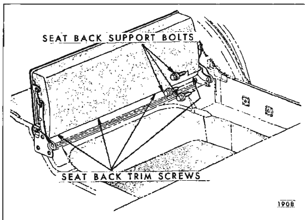
Fig. 15-74—Folding Third Seat Back
