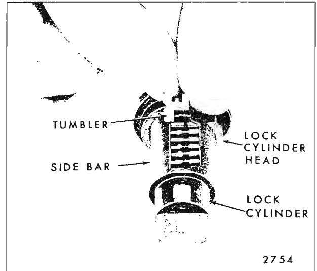
Fig. 1-5—Installing Tumblers
