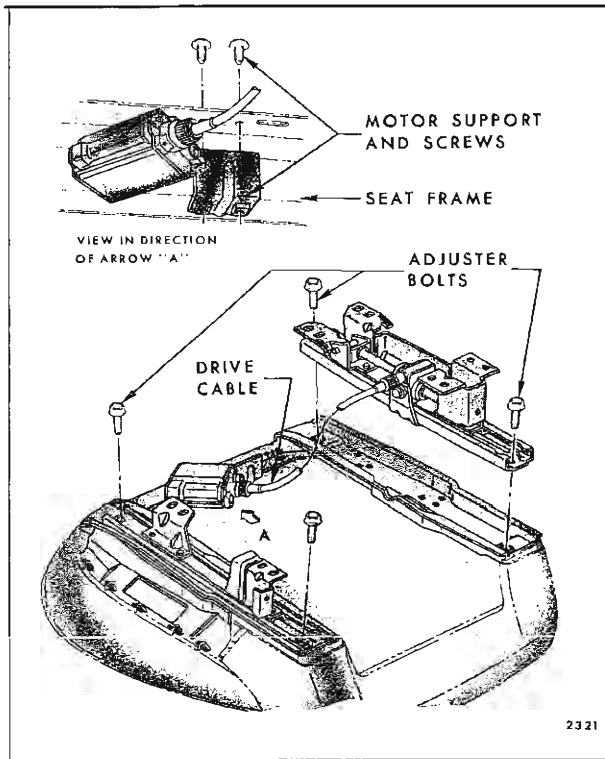
Fig. 15-44—Power Horizontal Bucket Seat Adjuster Removal
