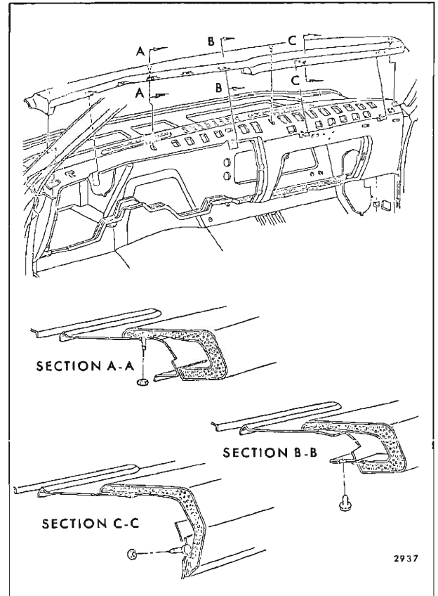
Fig. 5-20—Instrument Panel Cover - Chevrolet "A" Styles
