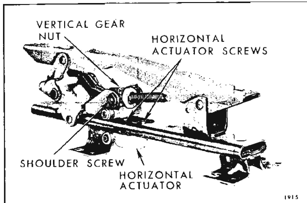
Fig. 15-12—Four-Way Seat Adjuster - "A" Styles
