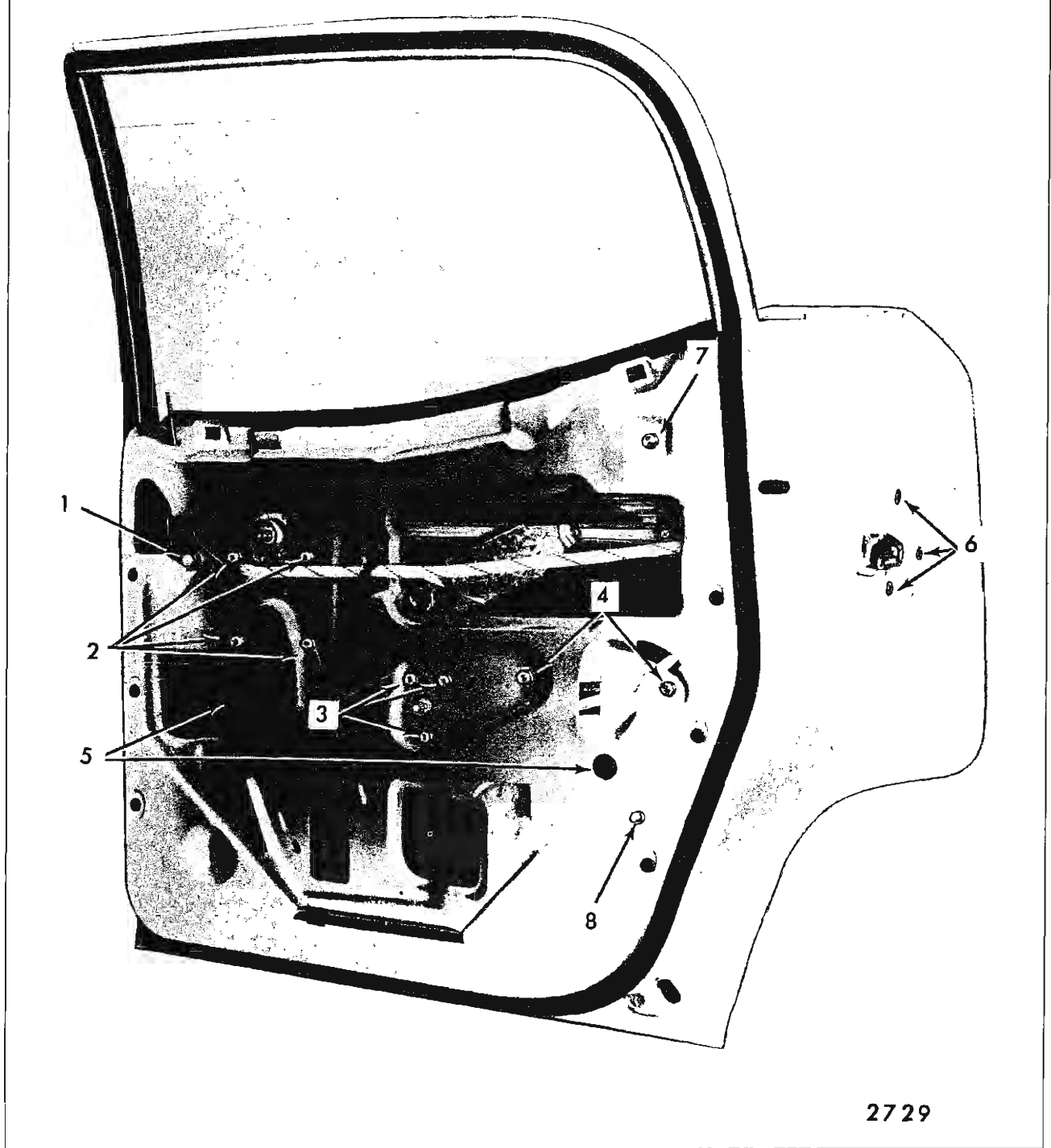
Fig. 6-106—Rear Door Hardware - "A" Closed Styles
