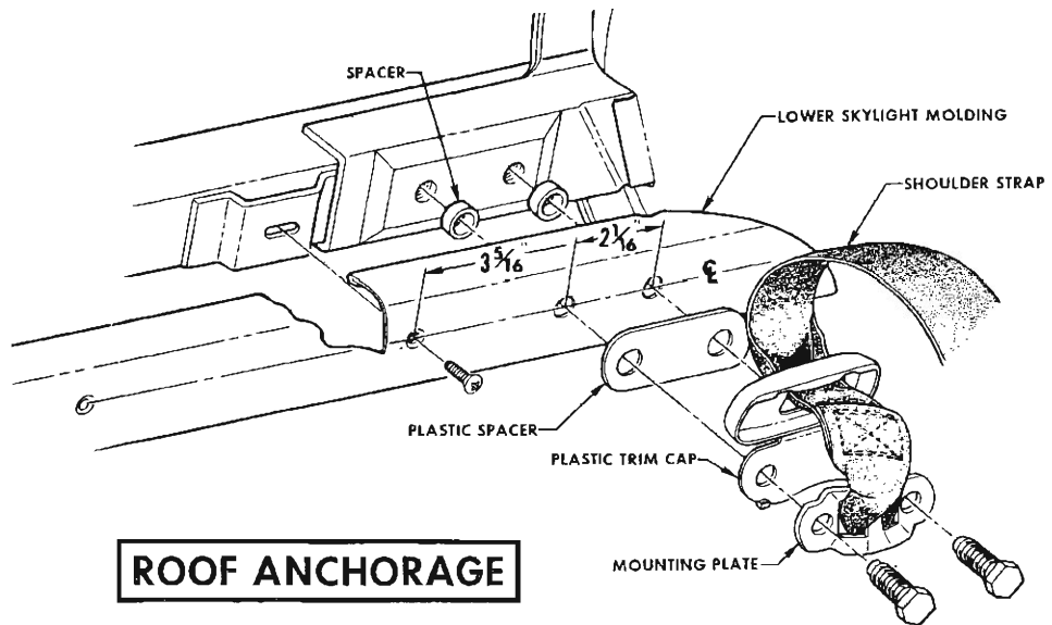
VIEW A
