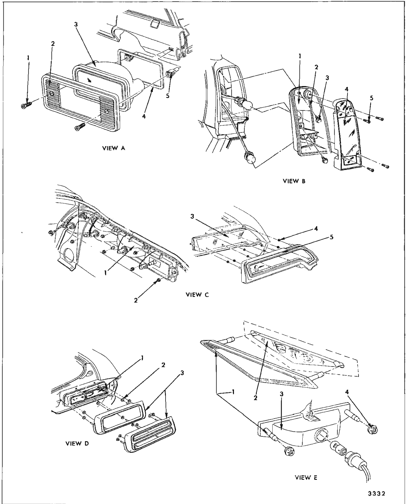
Fig. 16-42—Tail Lamp - Pontiac (U.S. and Canadian) Styles
