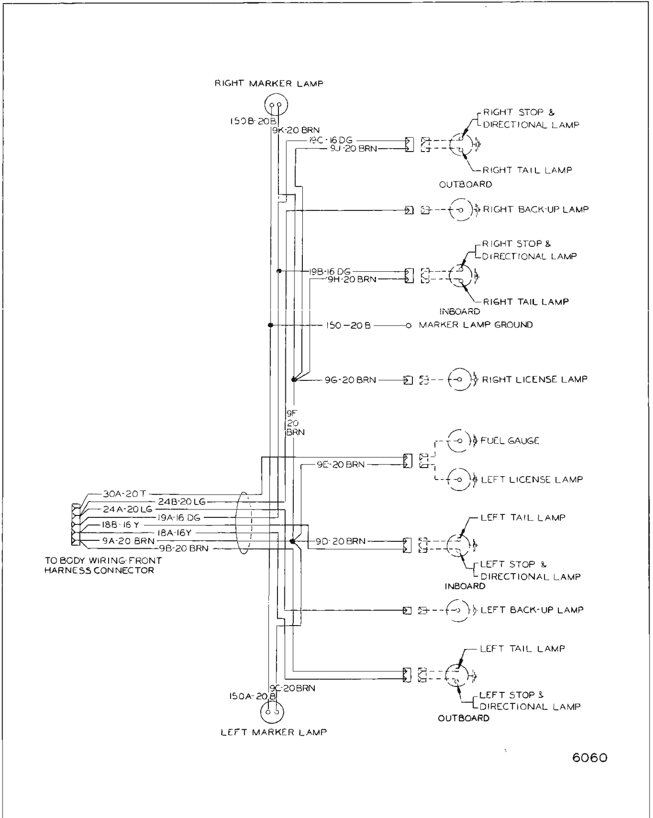
Fig. 16-56—Wiring Diagram Rear - Chevrolet "B" Styles
