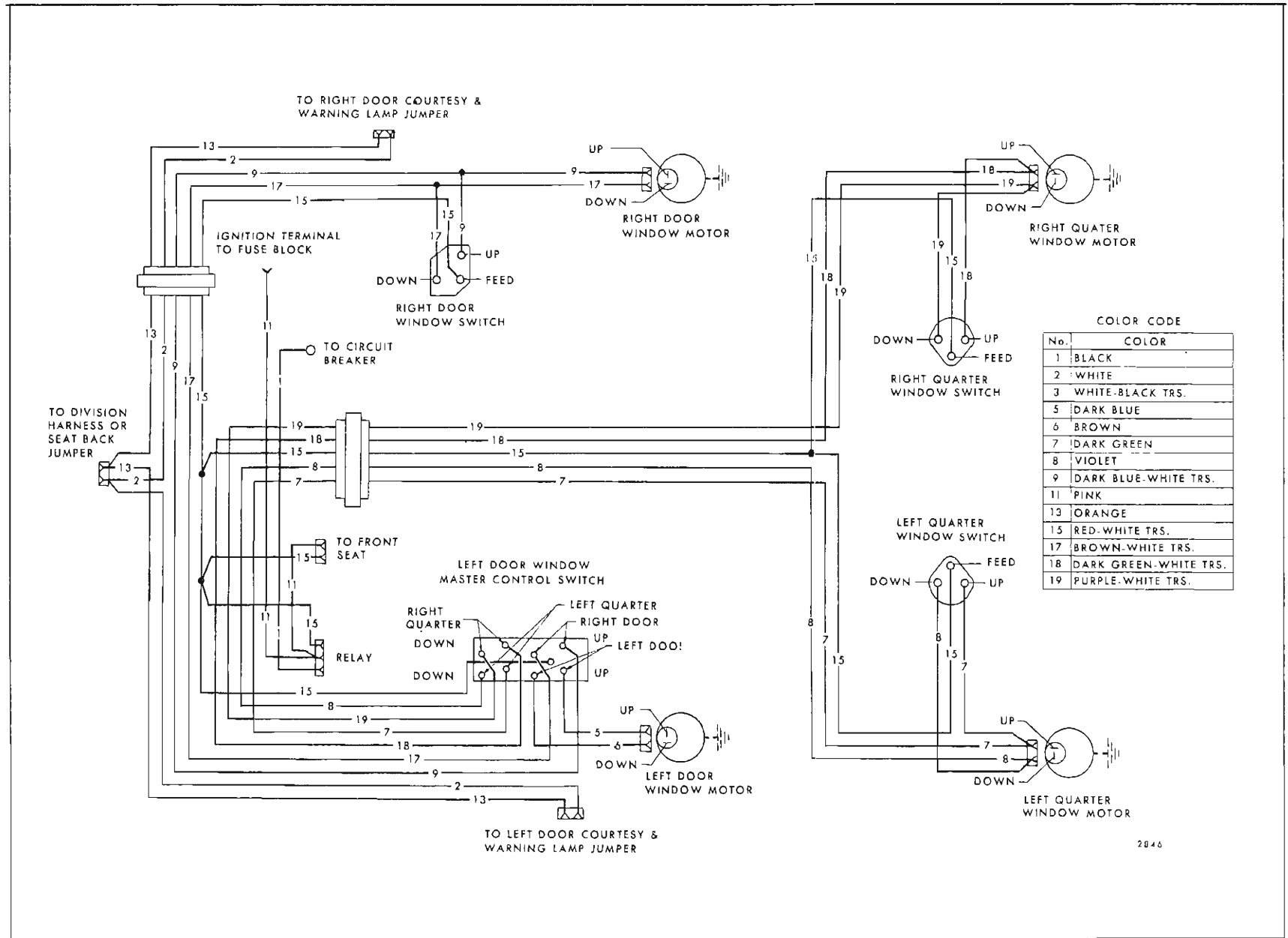
Fig. 16-5—Power Window Circuit - Oldsmobile "E" Styles
