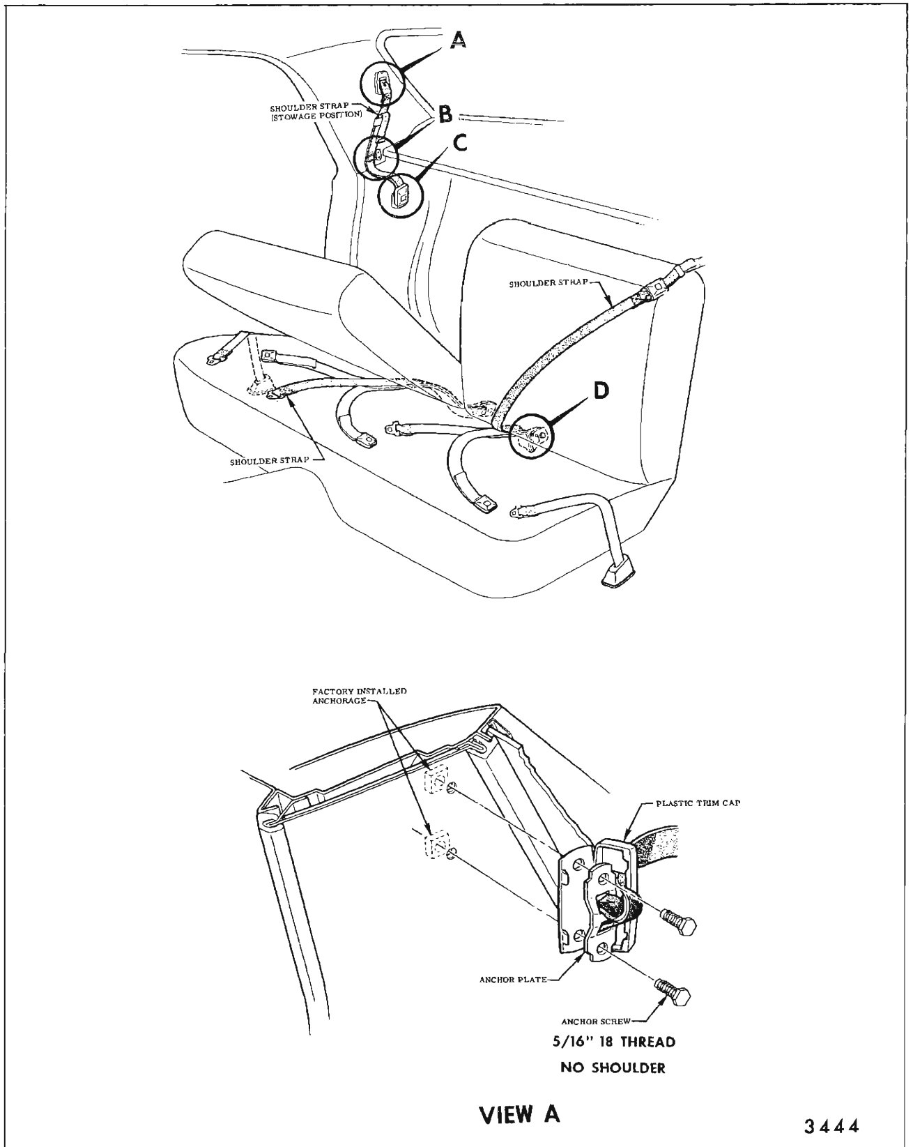
Fig. 15-104—Front Seat Shoulder Strap - "A-80" Styles
