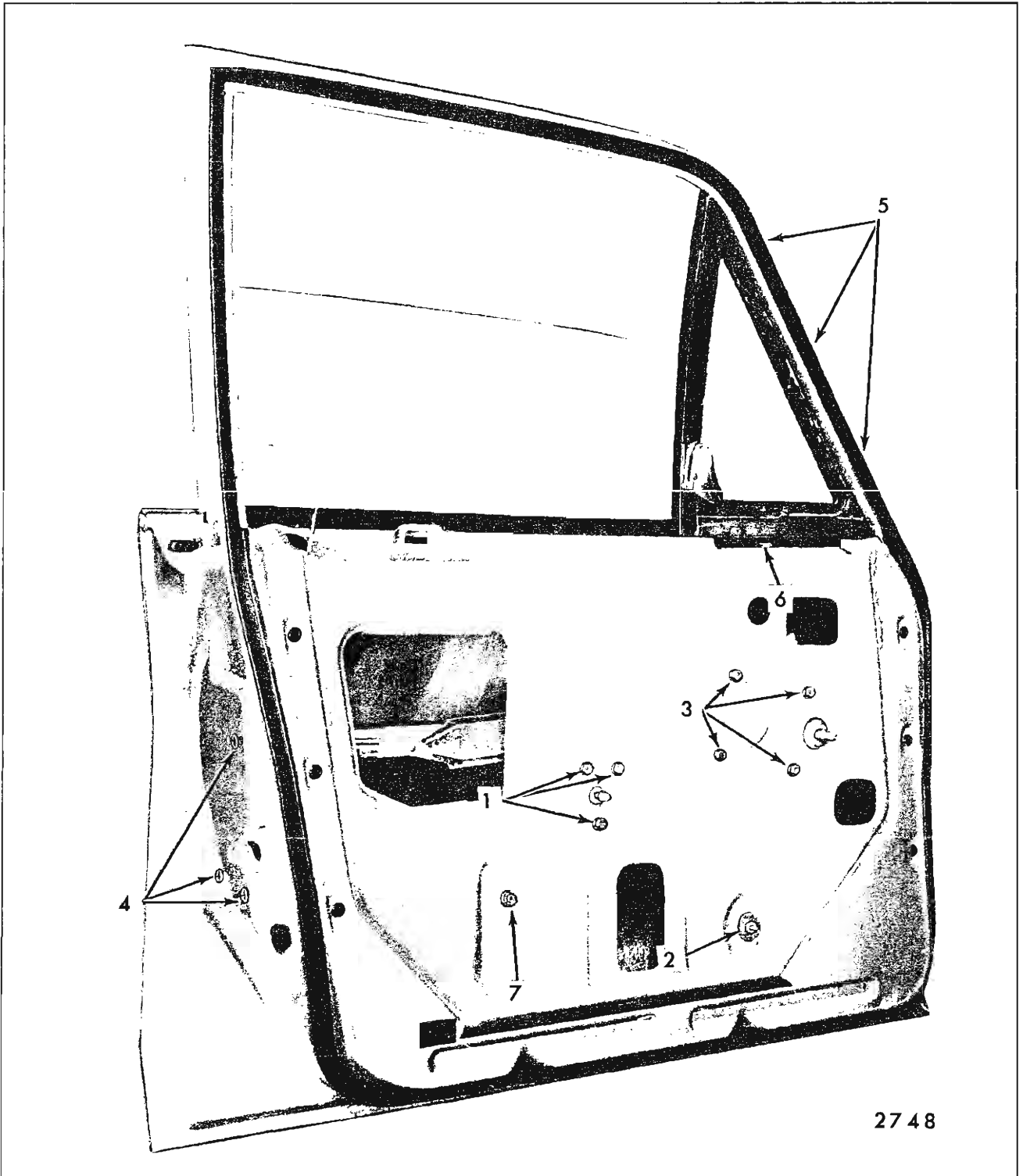
Fig. 6-56—Front Door Hardware - "X-69" Style Shown, "X-27" Style Similar
