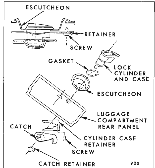
Fig. 15-80—Luggage Compartment Lock - Chevrolet "B" Styles
