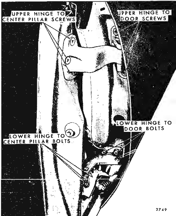
Fig. 6-115—Typical Rear Door Hinge Installation
