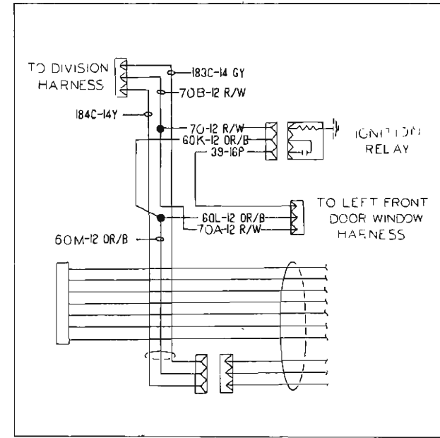
POWER TAILGATE + SIDE WINDOW INSTRUMENT WIRING
