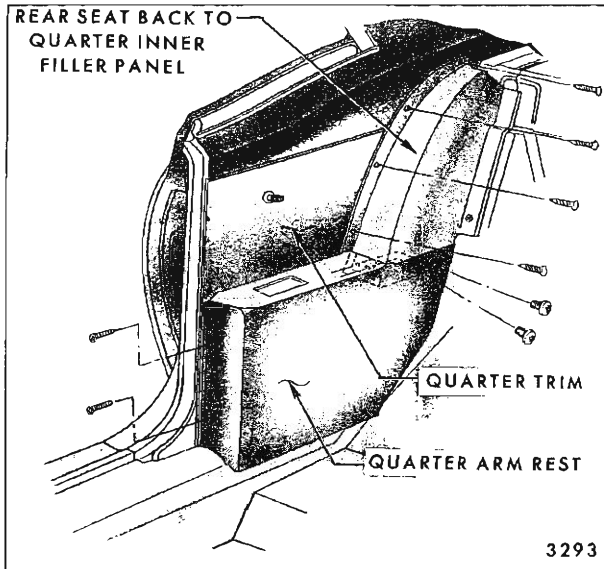
Fig. 14-23—Rear Quarter Trim - "F-37" Styles
