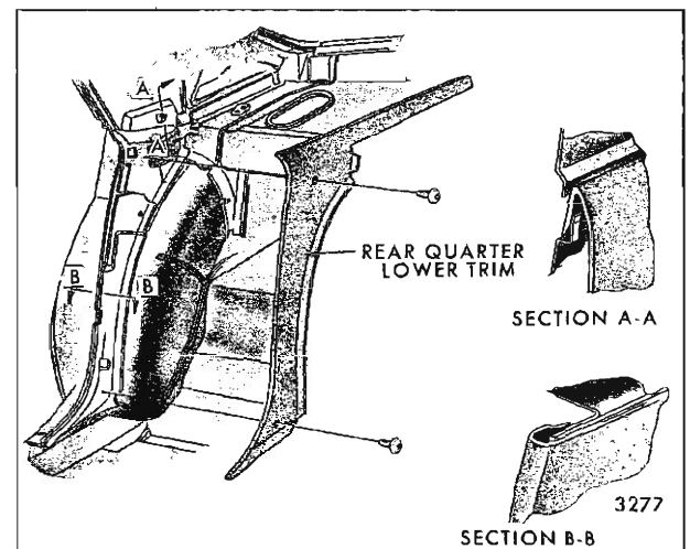
Fig. 14-30—Rear Quarter Trim Assembly - "A, B and X" Four-Door Styles and "A-80" style, Less Station Wagon
