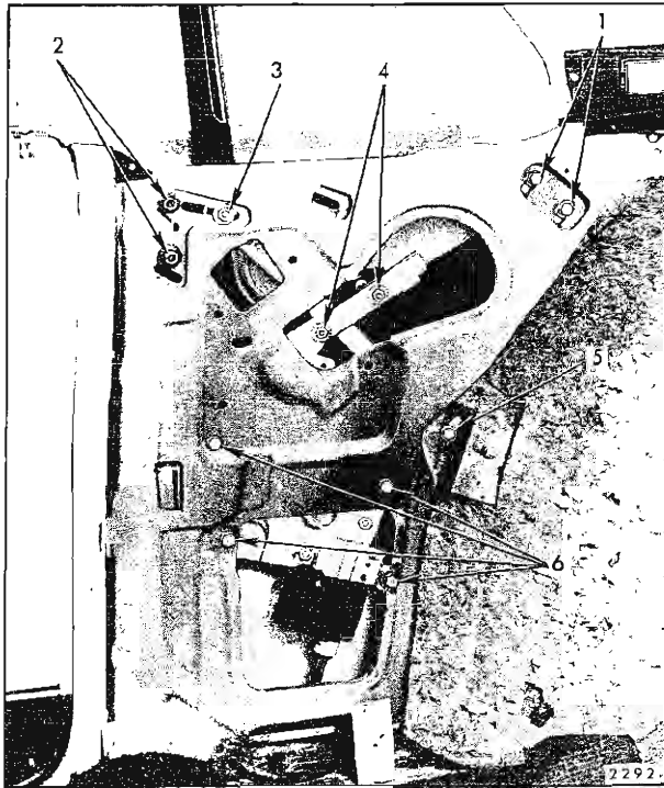
Fig. 7-24—Rear Quarter Hardware - "E" Body
