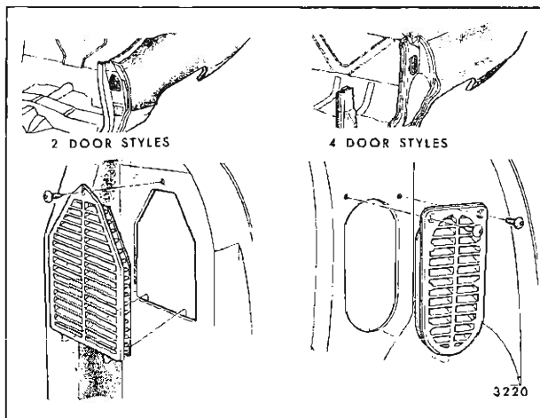
Fig. 5-16—Pressure Relief Valve - "A" Styles Shown
