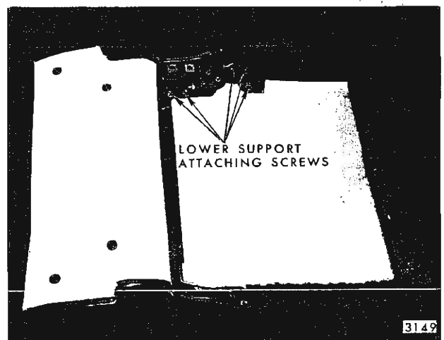
Fig. 15-64—Auxiliary Seat Lower Support - Cadillac Limousine Styles
