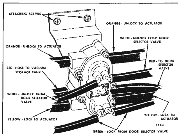
Fig. 6-29—Vacuum Lock Remote Control Valve
