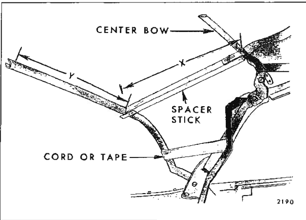
Fig. 13-4—Spacer Stick Installation
