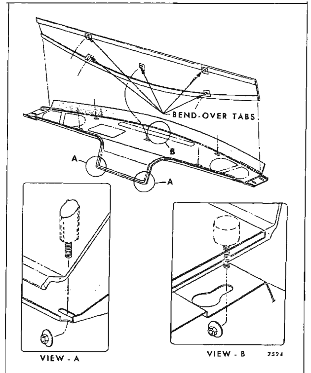
Fig. 14-44—Compartment Shelf Center Trim Panel - Cod. "E" Styles
