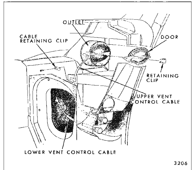
Fig. 5-5—Shroud Center Duct Upper Air Outlet Door - "A & G" Styles
