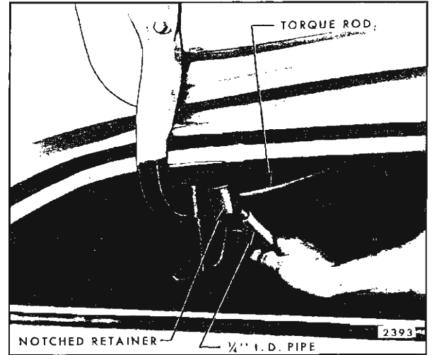
Fig. 8-8—Rear Compartment Lid Attachments - All "F" Styles
