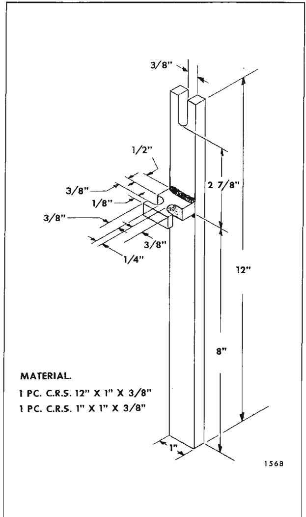
Fig. 8-5—Torque Rod Adjusting Tool
