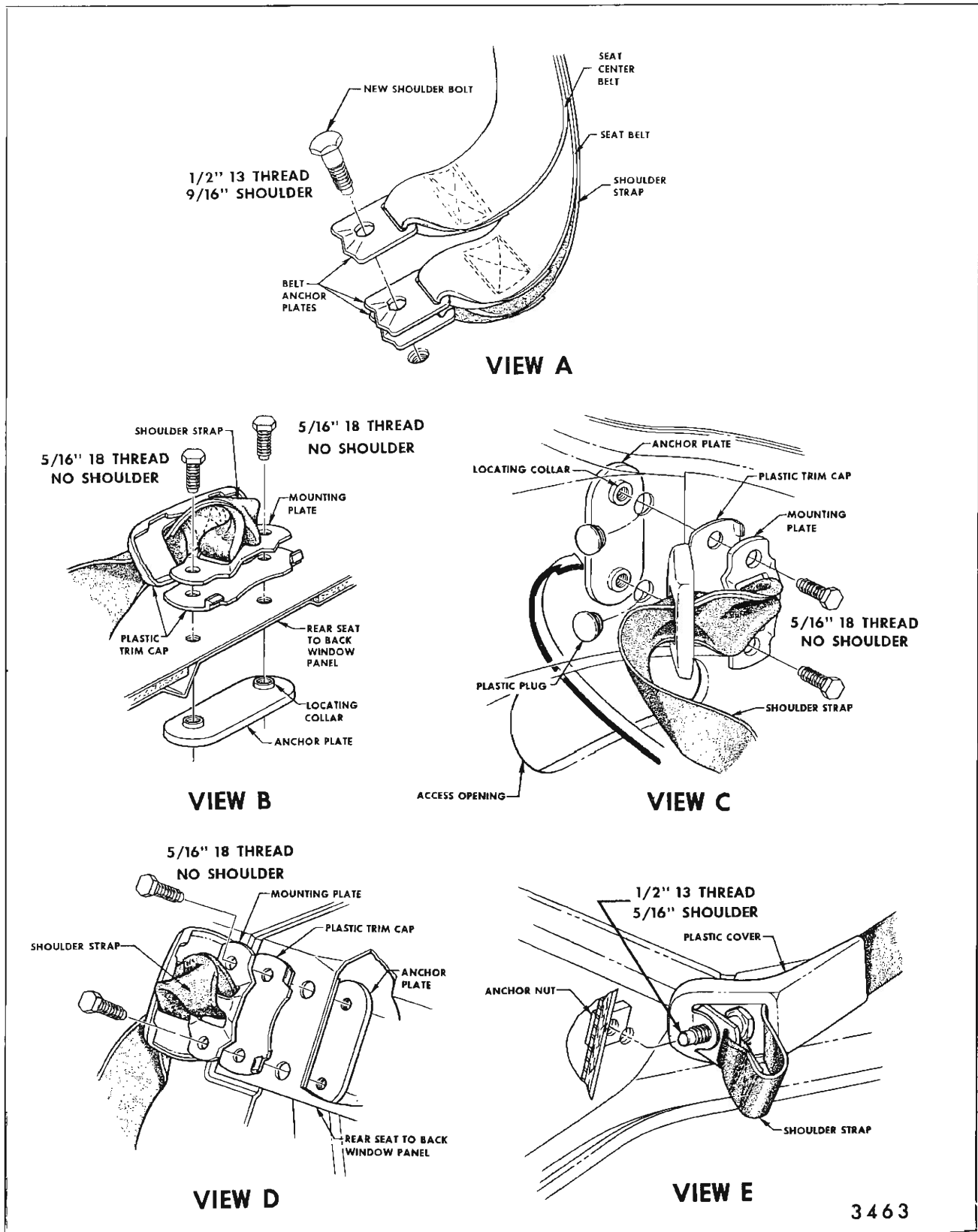
Fig. 15-108—Rear Seat Shoulder Straps - All Styles Except Station Wagons and Convertibles (Refer to Fig. 15-107)
