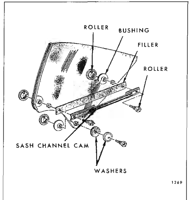
Fig. 7-40—Rear Quarter Window Assembly - "Z-37" Styles
