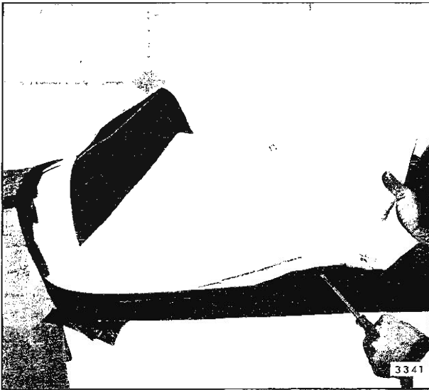
Fig. 13-32—Raising End of Trimstick "A" Styles cover to new one as follows: Place new top cover on a suitable clean surface, such as on clean roof of a car to provide proper contour and fullness, with inner surface of cover down.
