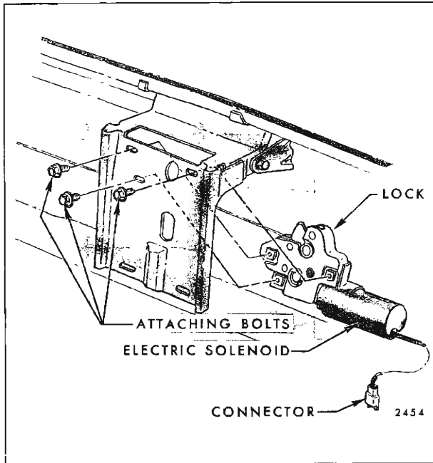
Fig. 8-28—Rear Compartment Lid Lock Electric Release Unit
