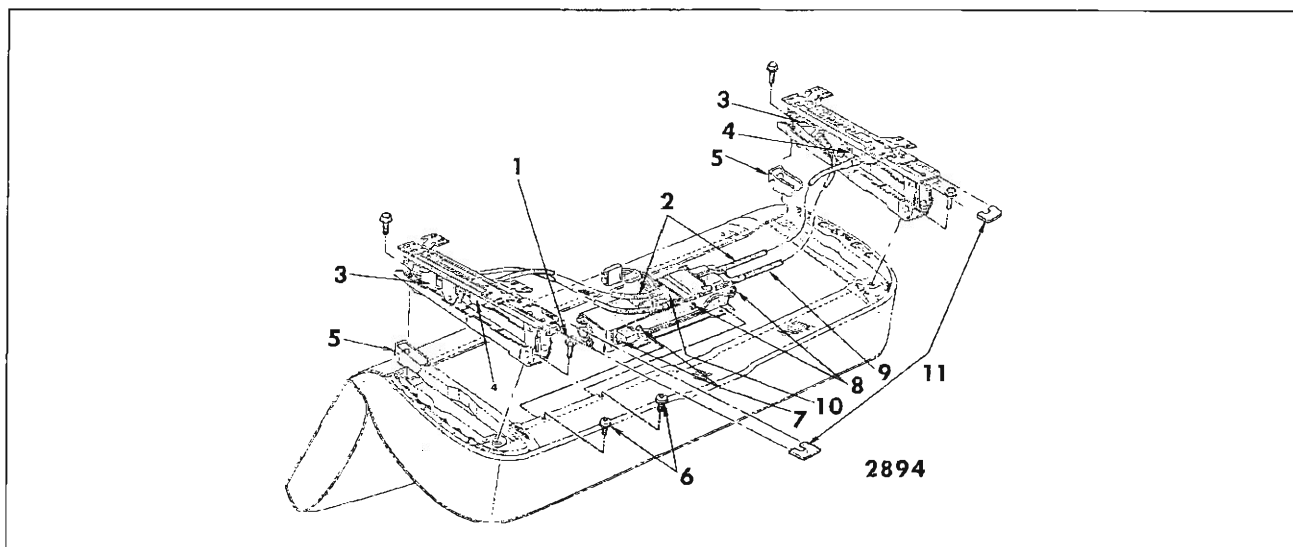
Fig. 15-8—Front Seat Assembly - Four-Way Tilt - Buick "B, C & E" Styles
