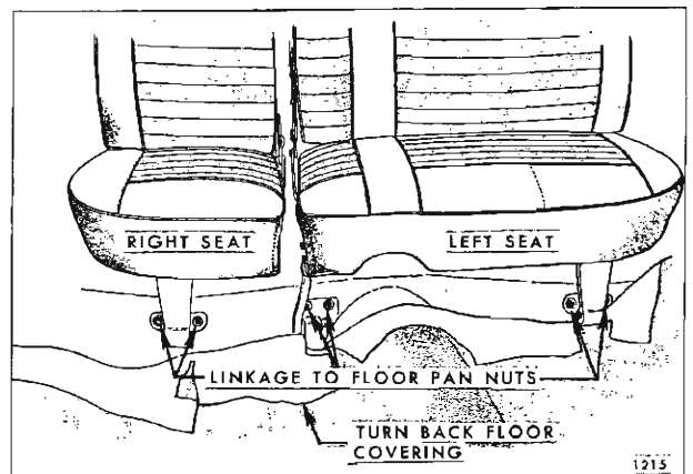
Fig. 15-86—Folding Second Seat Front Linkage (Vista Cruiser and Sport Wagon Styles)
