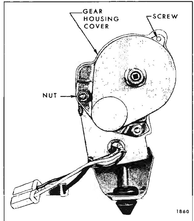
Fig. 13-74—Folding Top Lift Assembly
