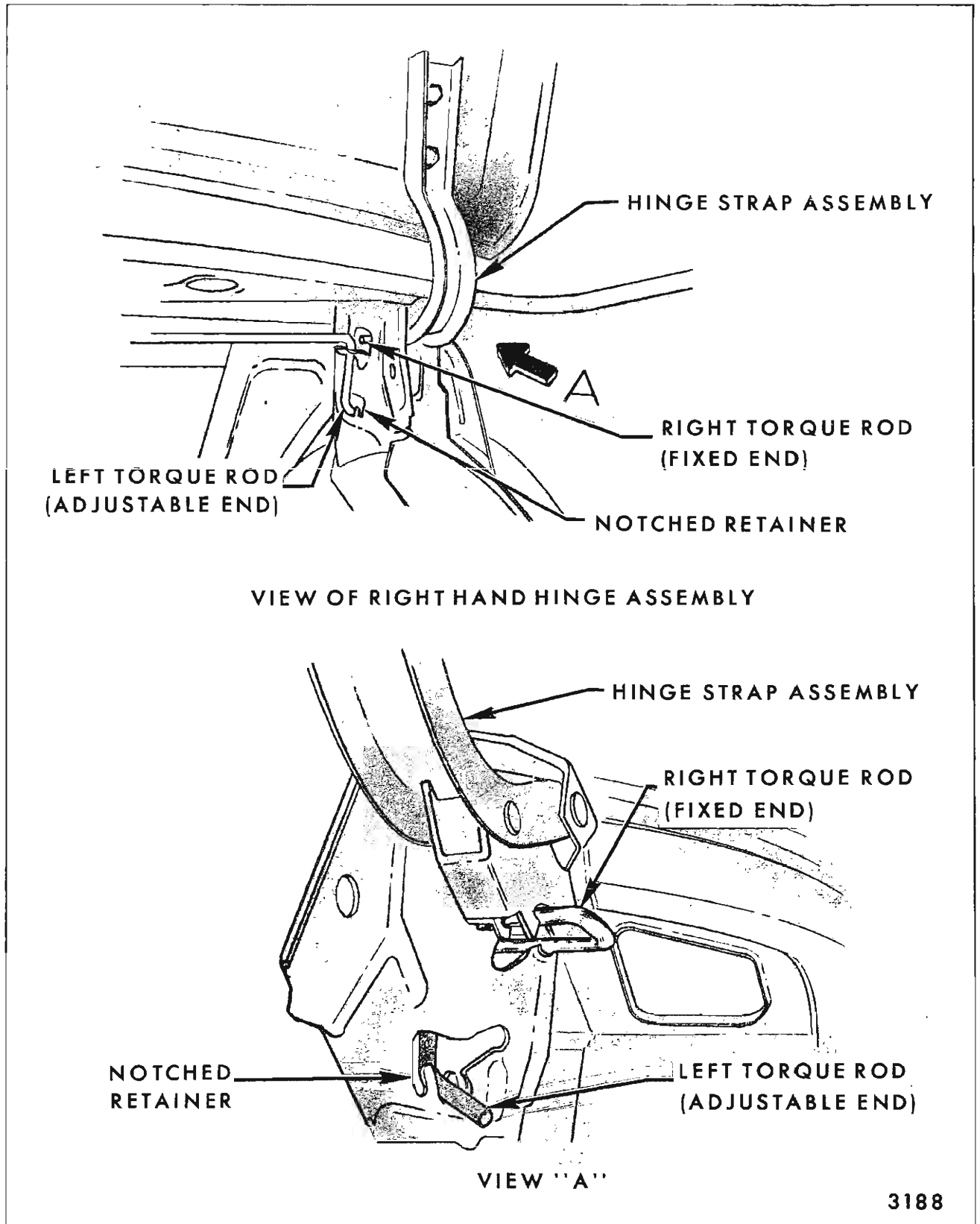
Fig. 8-10—Typical Torque Rod Adjustment
