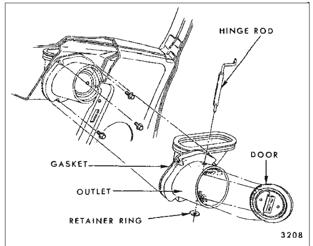
Fig. 5-6—Shroud Center Duct Upper Air Outlet and Door - "F" Styles
