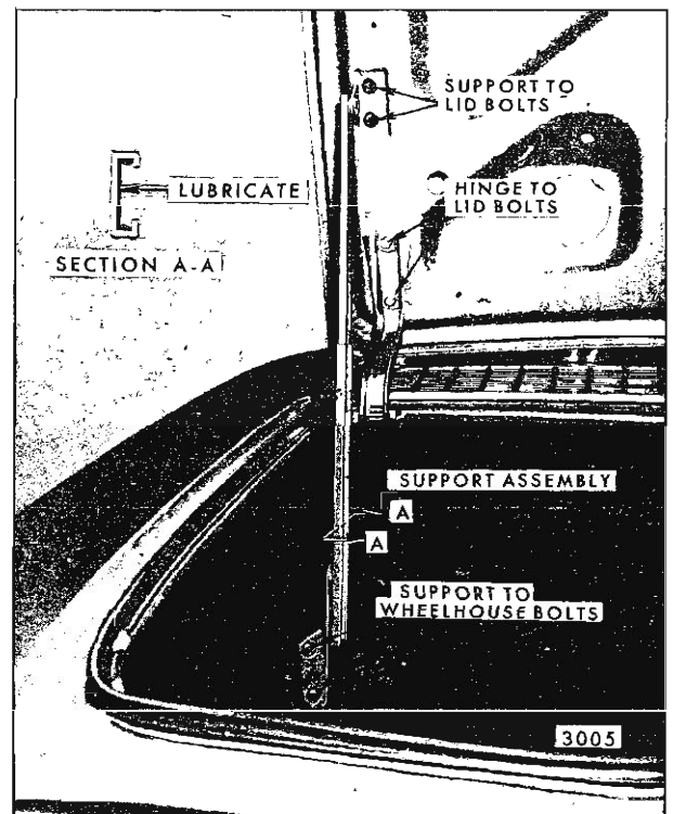
Fig. 2-19—Engine Compartment Lid Lubrication
