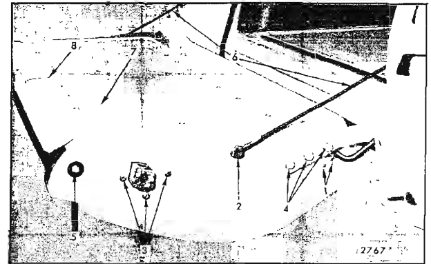
Fig. 9-39—Tail Gate Hardware - Right Side
