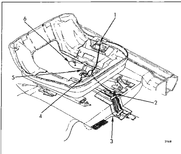
Fig. 16-24—Horizontal Bucket Seat Wiring
