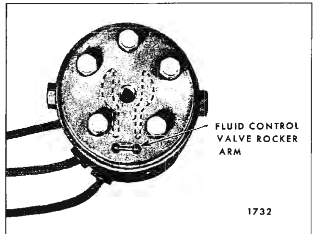
Fig. 13-63—Pump Cover Plate
