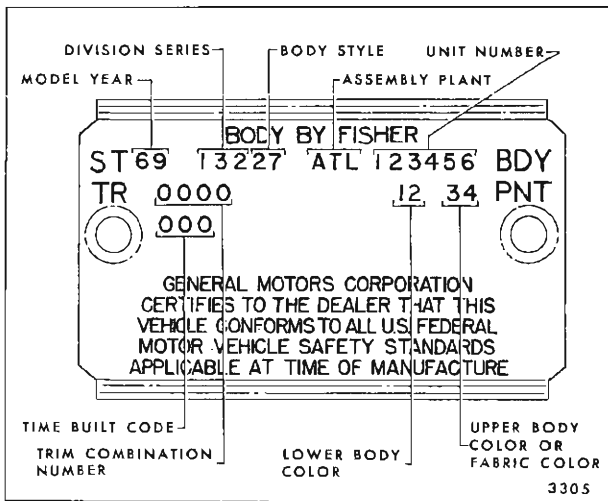
Fig. 1-1—Body Number Plate - U.S. Models
