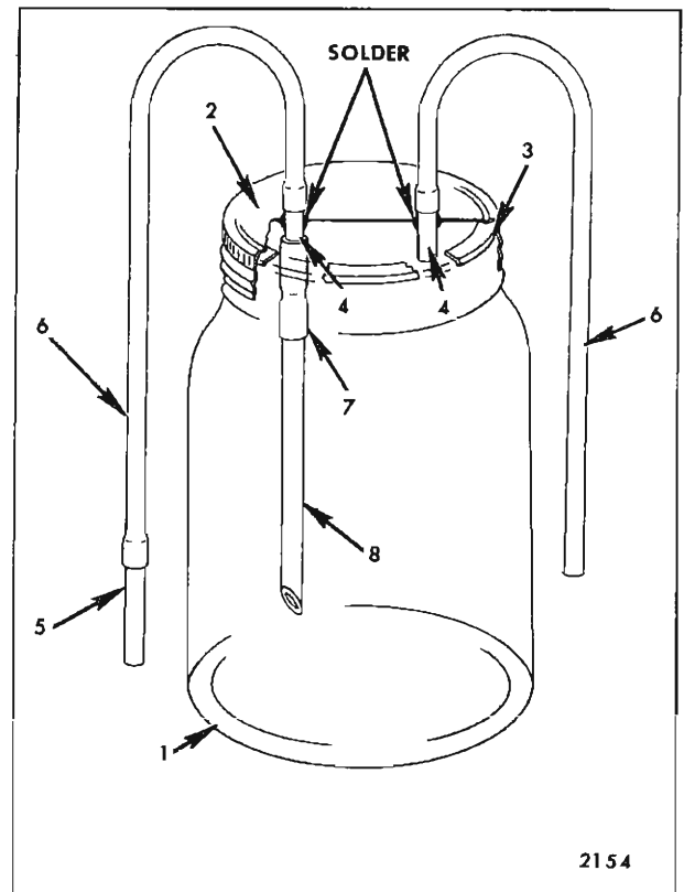
Fig. 6-30—Leak-Down Testing Device (See Text for Specifications of Components)
