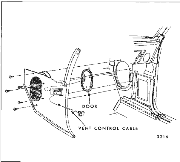
Fig. 5-10—Shroud Side Finishing Panel - "F" Styles
