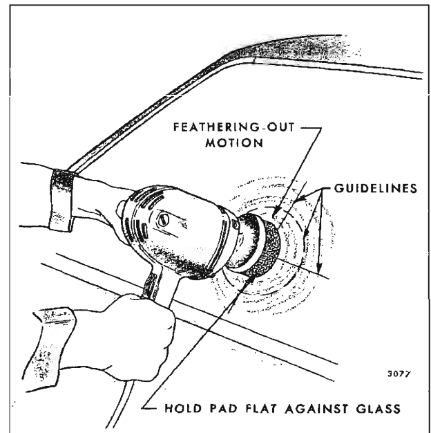
Fig. 1-9—Minor Glass Scratch Removal
