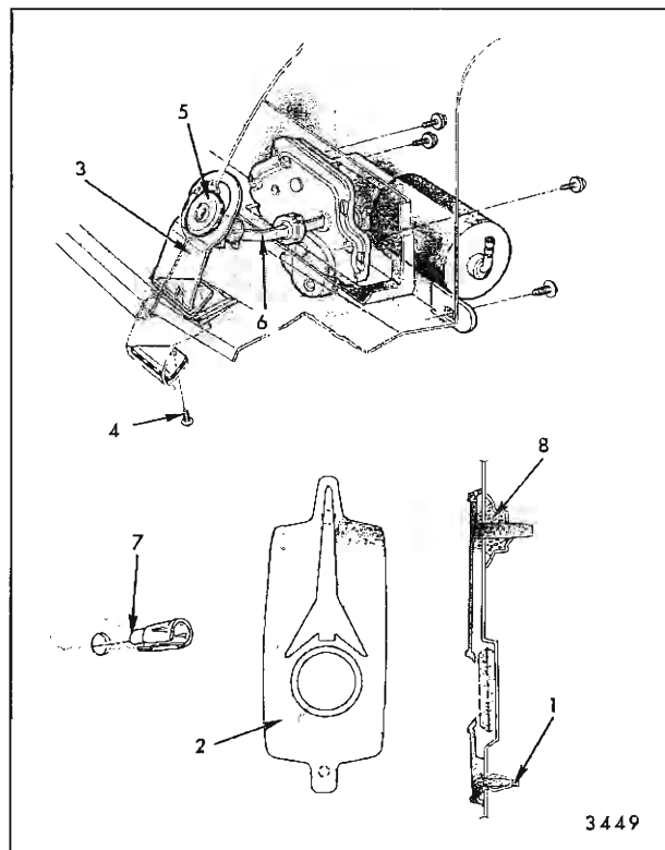
Fig. 8-20—Rear Compartment Lock Cylinder and Emblem Assembly - Oldsmobile "B" Styles
