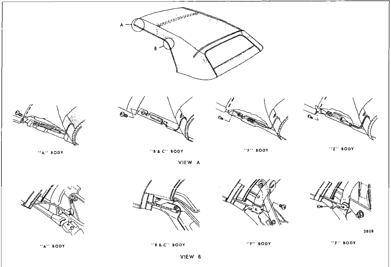
Fig. 13-25—Hold Down Cable Attachment
