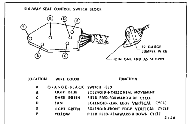
Fig. 16-38—Six-Way Seat Switch Block in Arm Rest
