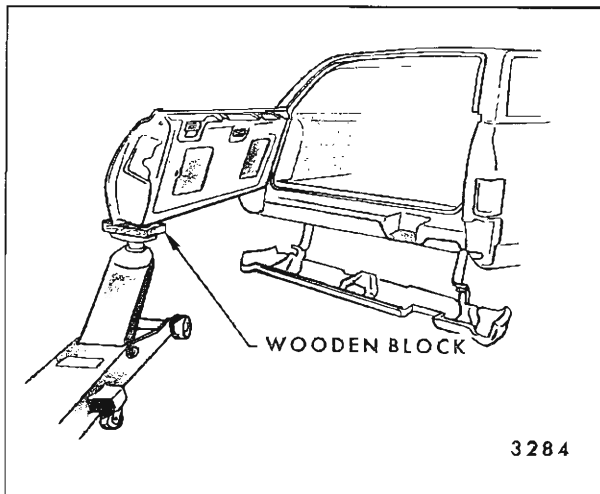
Fig. 9-10—Tail Gate Removal
