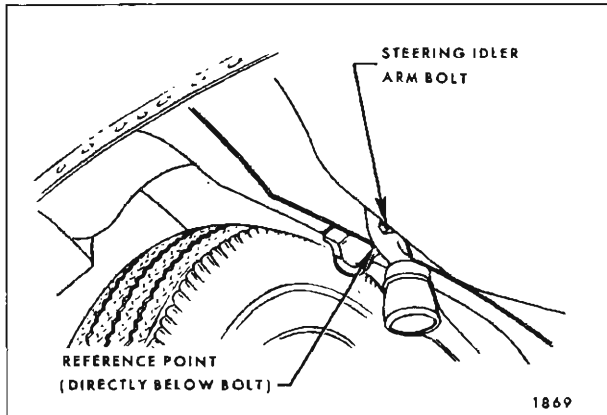
Fig. 3-5—Reference Point at Steering Idler Arm
