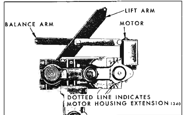
Fig. 6-36—Door Window Regulator and Electric Motor Assembly
