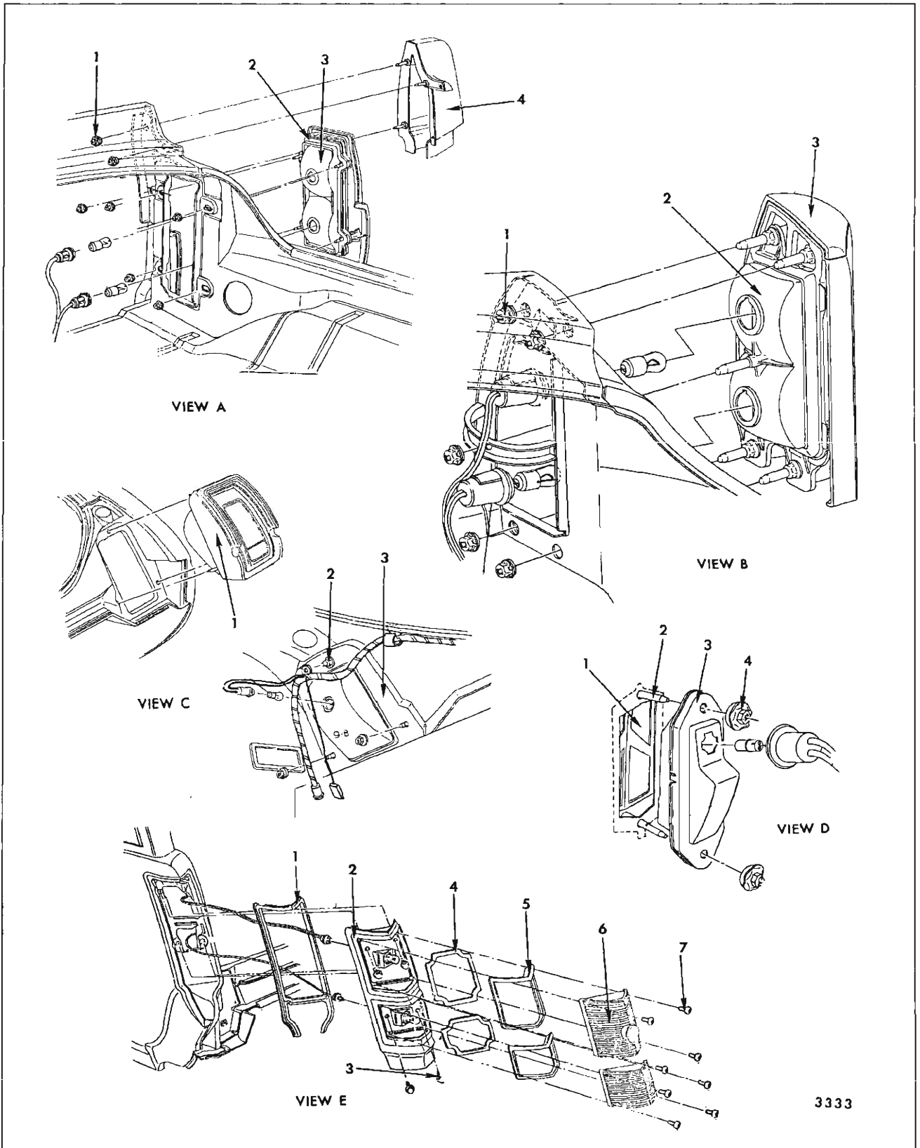
Fig. 16-43—Tail Lamp - Oldsmobile Styles
