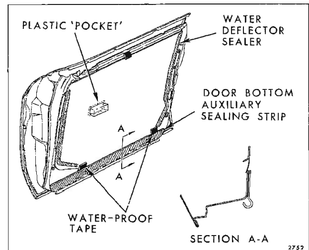
Fig. 6-6—Door Inner Panel Sealing
