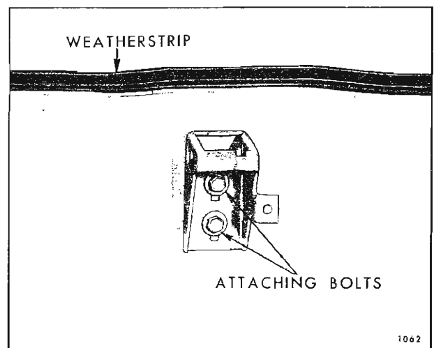
Fig. 8-13—Engine Compartment Lid Latch Striker - "Z" Styles
