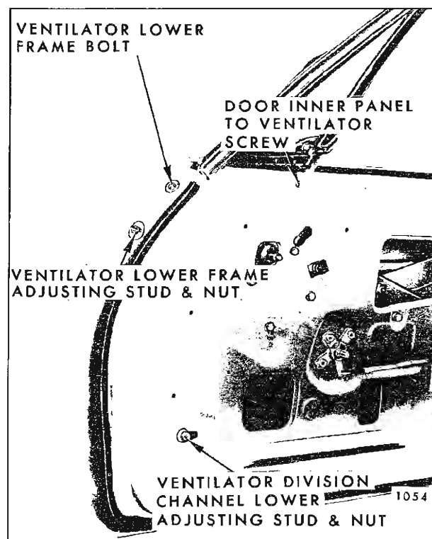
Fig. 6-75—Front Door Ventilator Attachments - “Z” Styles
