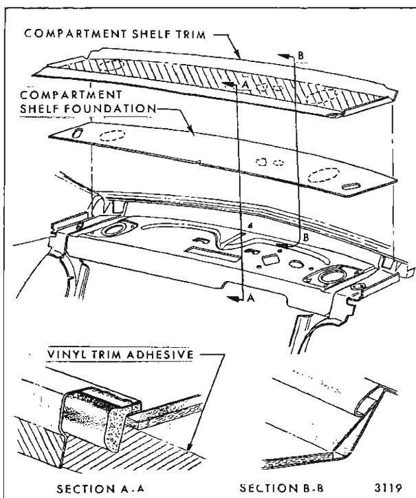
Fig. 14-40—Compartment Shelf Trim Panel - Typical All Less "E and Z" Styles
