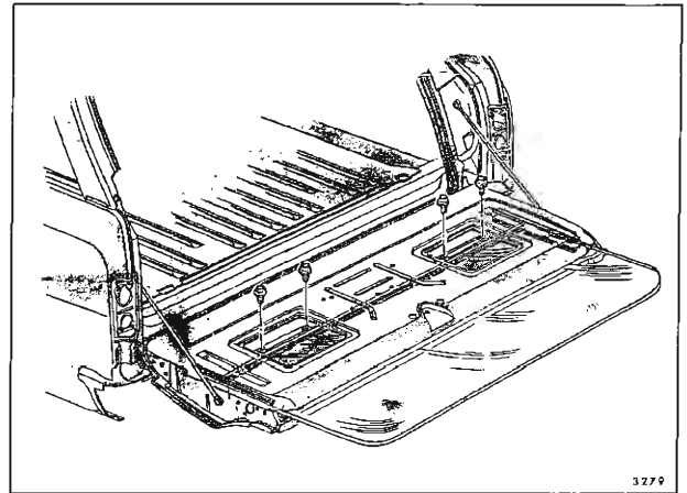
Fig. 9-41—Tail Gate Inner Cam Attachments
