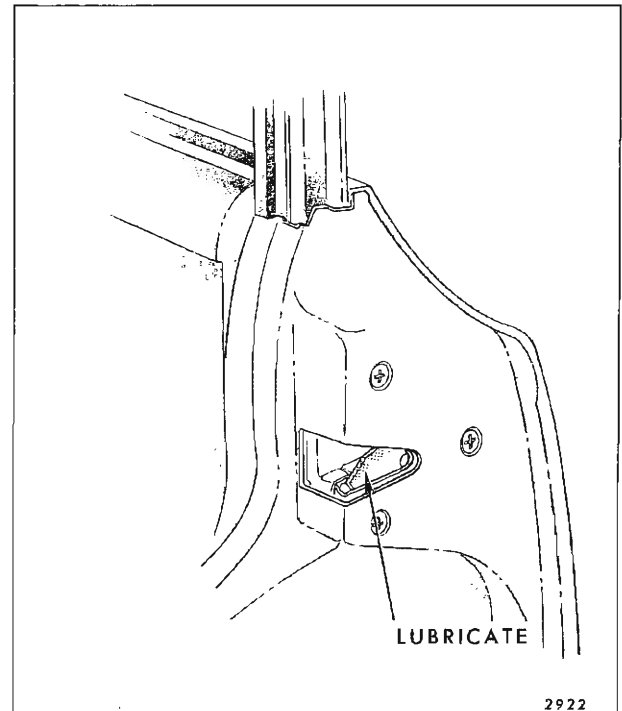
Fig. 2-6—Door Lock Fork Bolt Lubrication
