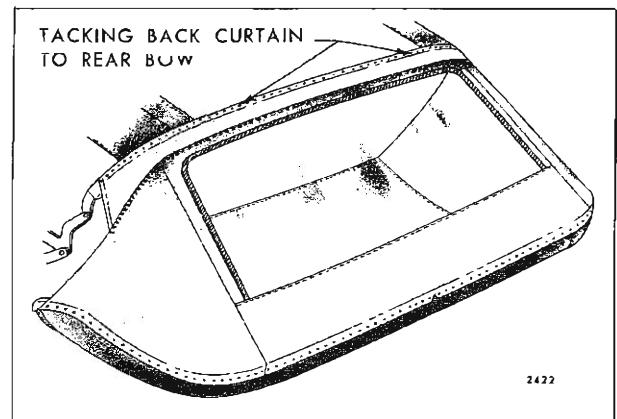
Fig. 13-21—Tacking Back Curtain
