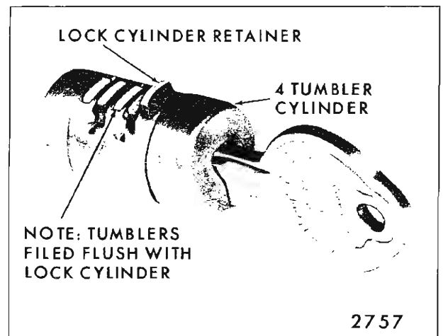
Fig. 1-8—Coded Glove Compartment Cylinder
