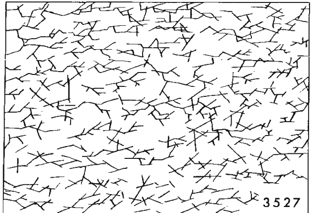
Fig. 1-15—Crazing
