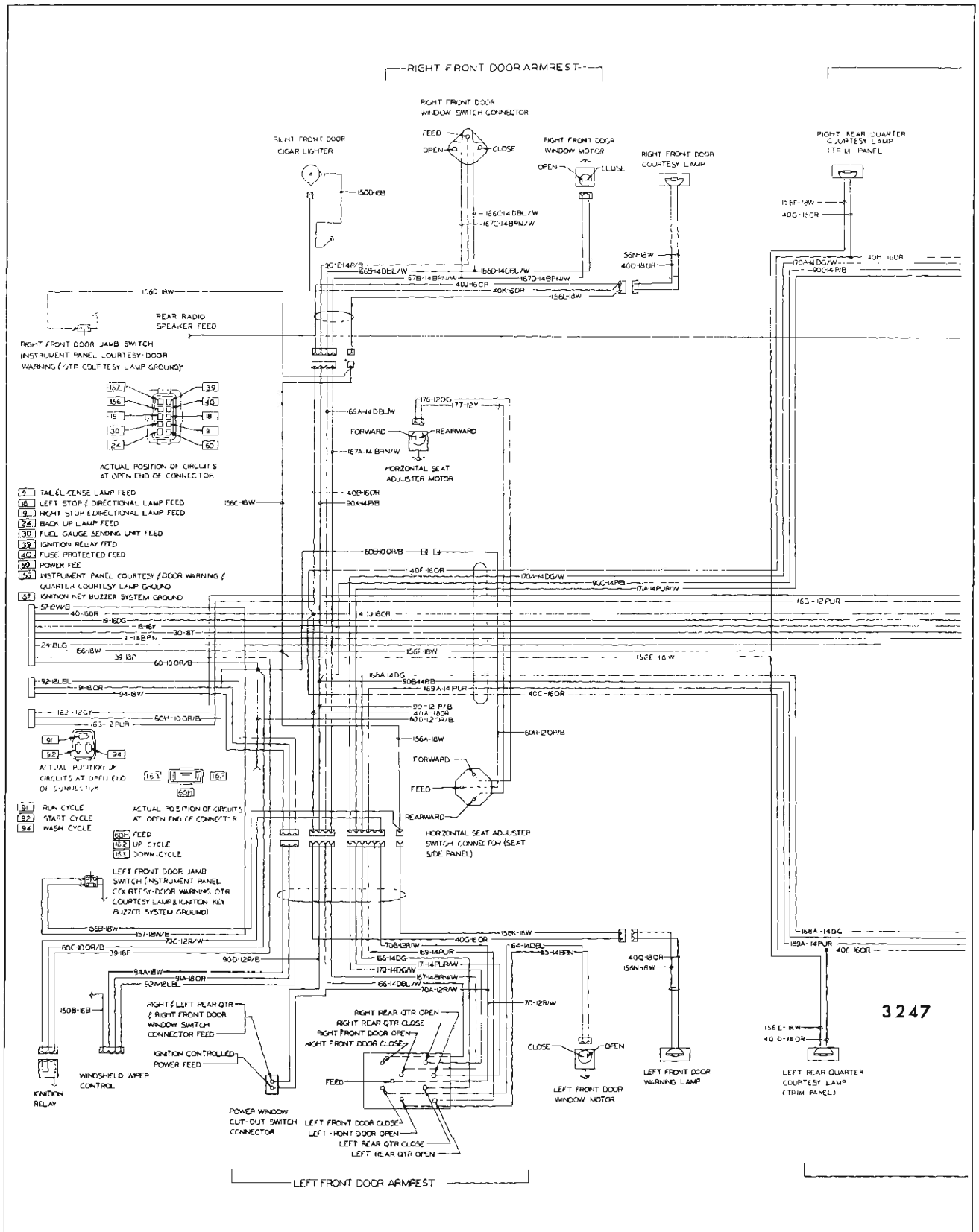
Fig. 16-68—Wiring Diagram - Cadillac "C-67" Styles
