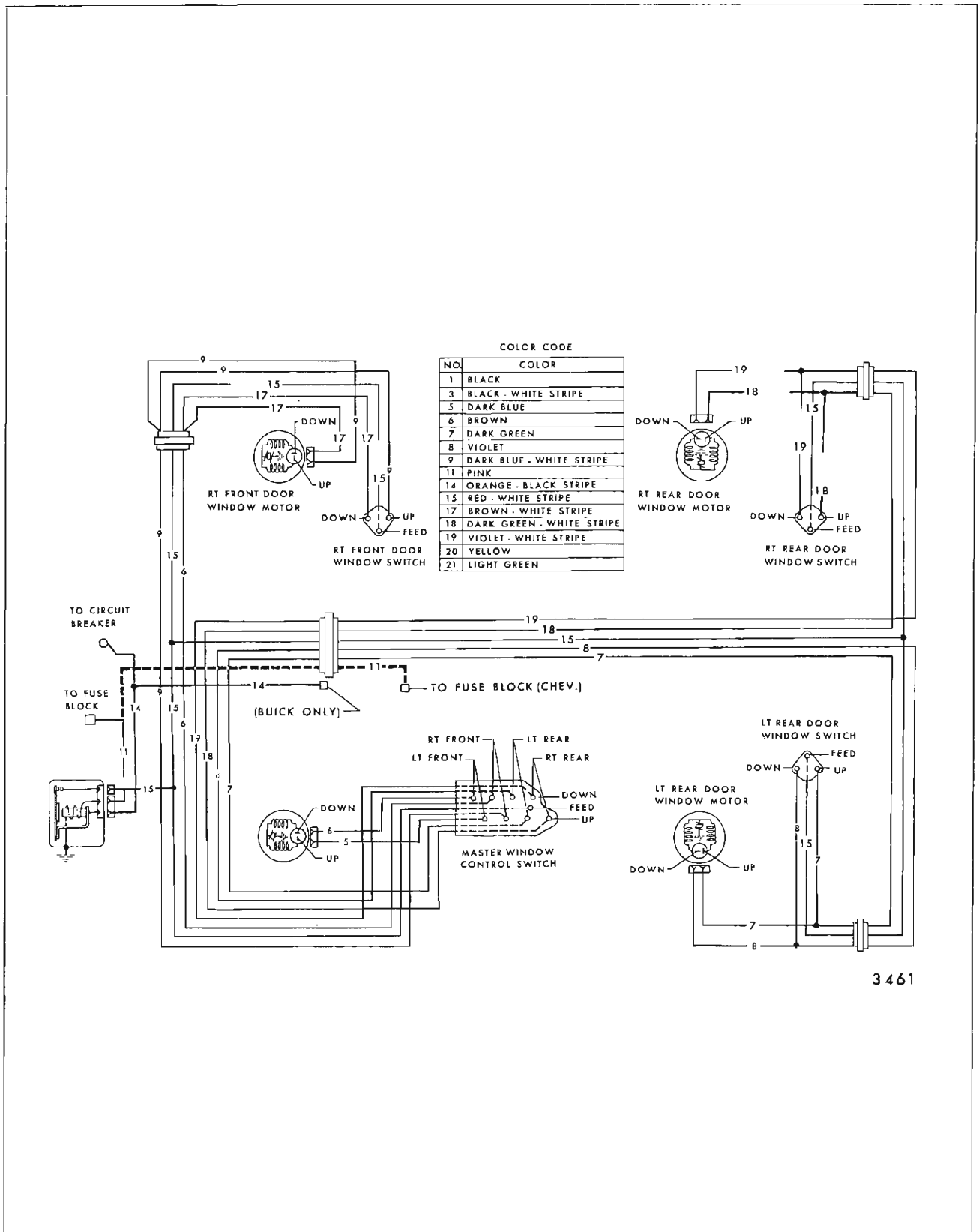
Fig. 16-2—Power Window Circuit - Typical "B" Styles
