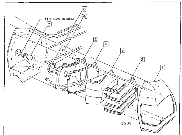
Fig. 16-41—Tail Lamp - Beaumont (Canadian) Styles
