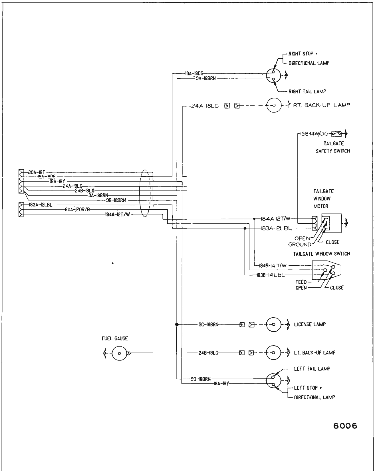
Fig. 16-16—Power Tail Gate Window Rear Wiring Circuit - Oldsmobile "A" Styles
