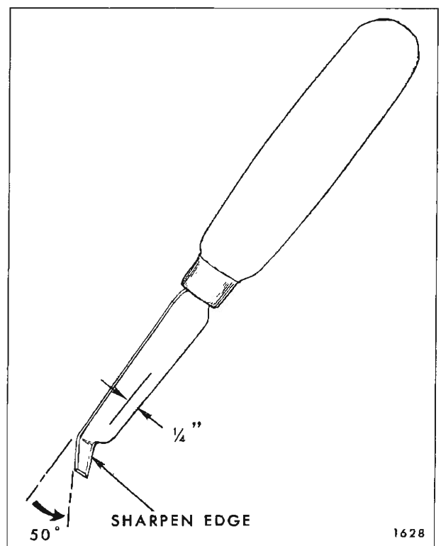
Fig. 12-4—Fabric Cover Trimming Tool
