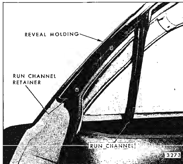
Fig. 9-33—Tail Gate Upper Glass Run Channel Retention
