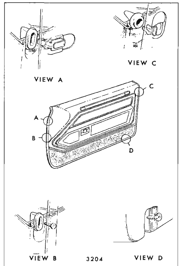
Fig. 14-11—Various Types of Door Trim Retention
