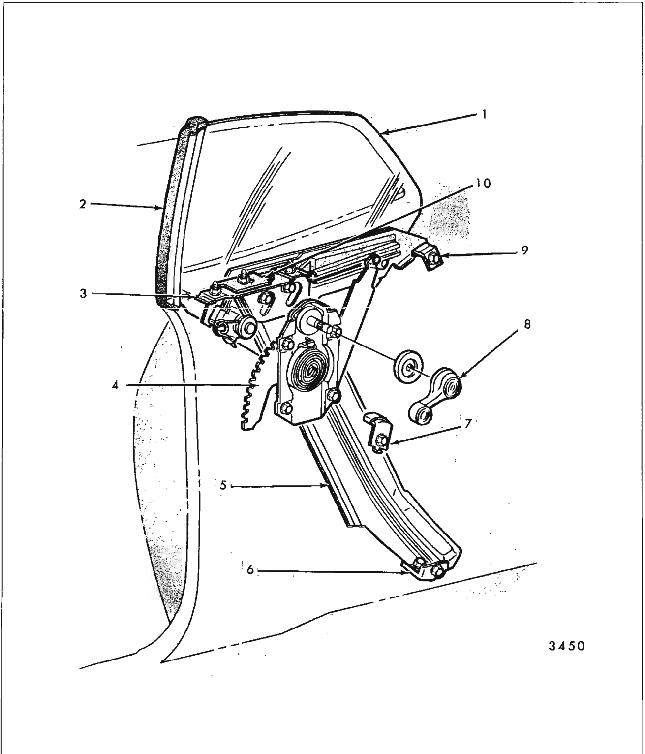
Fig. 7-16—Quarter Window Hardware - "B & C" Body 1. Quarter Window Glass 5. Guide 8. Handle 2. Sash Channel 6. Lower Guide Support Assembly 9. Upper Rear Stop Assembly 3. Support Assembly 7. Lower Stop Assembly 10. Upper Front Stop Assembly 4. Regulator Assembly
