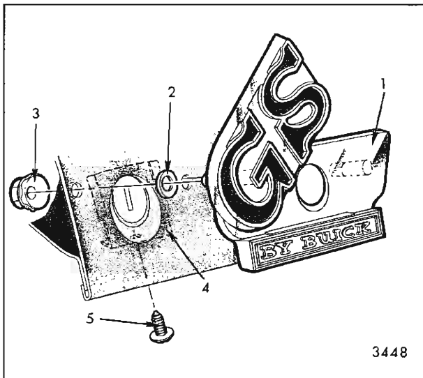
Fig. 8-18—Lock Cylinder Emblem - Buick 43437, 44637 and 44667 Styles
