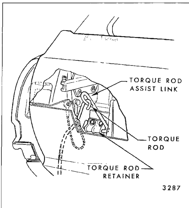
Fig. 9-7—Dual Gate - Torque Rod to Body Attachment
