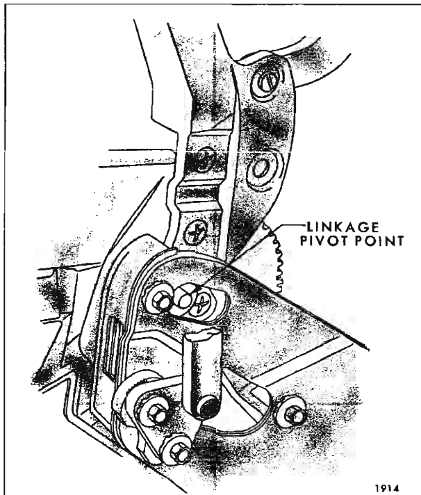
Fig. 13-88—Folding Top Linkage Pivot Point "Z" Styles
