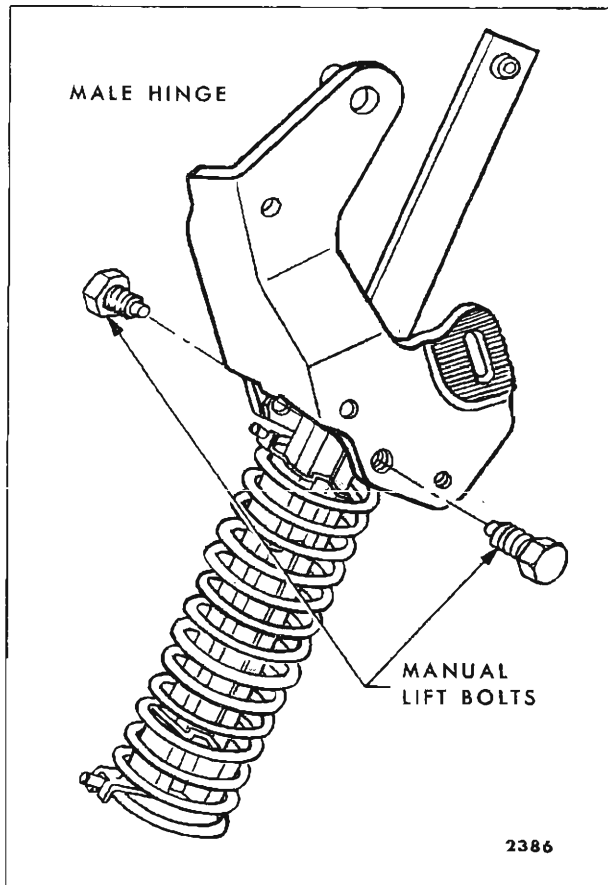
Fig. 13-77—Folding Top Manual Lift Attachment - "F" Styles
