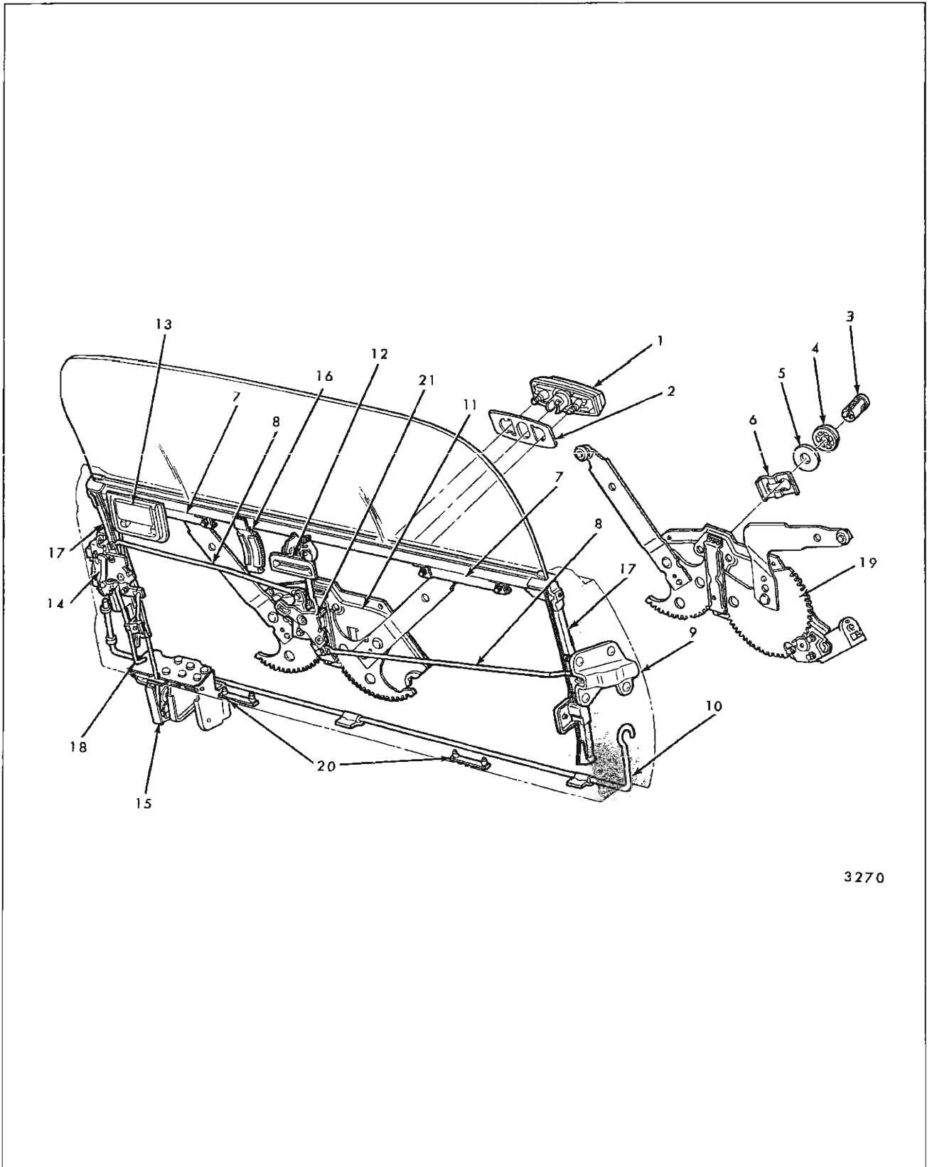
Fig. 9-1—Dual Acting Tail Gate
