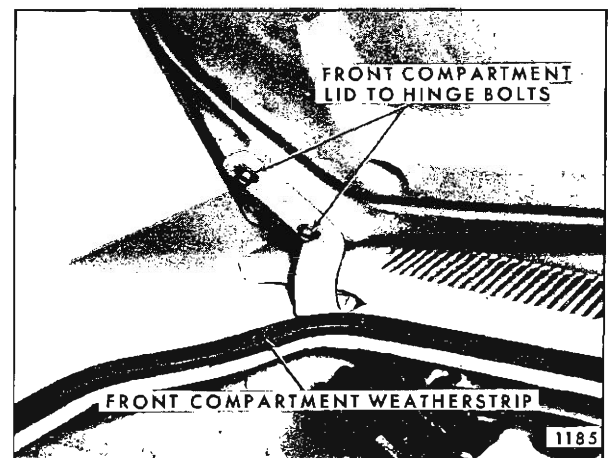
Fig. 5-24—Front Compartment Weather Strip and Lid to Hinge Bolts
