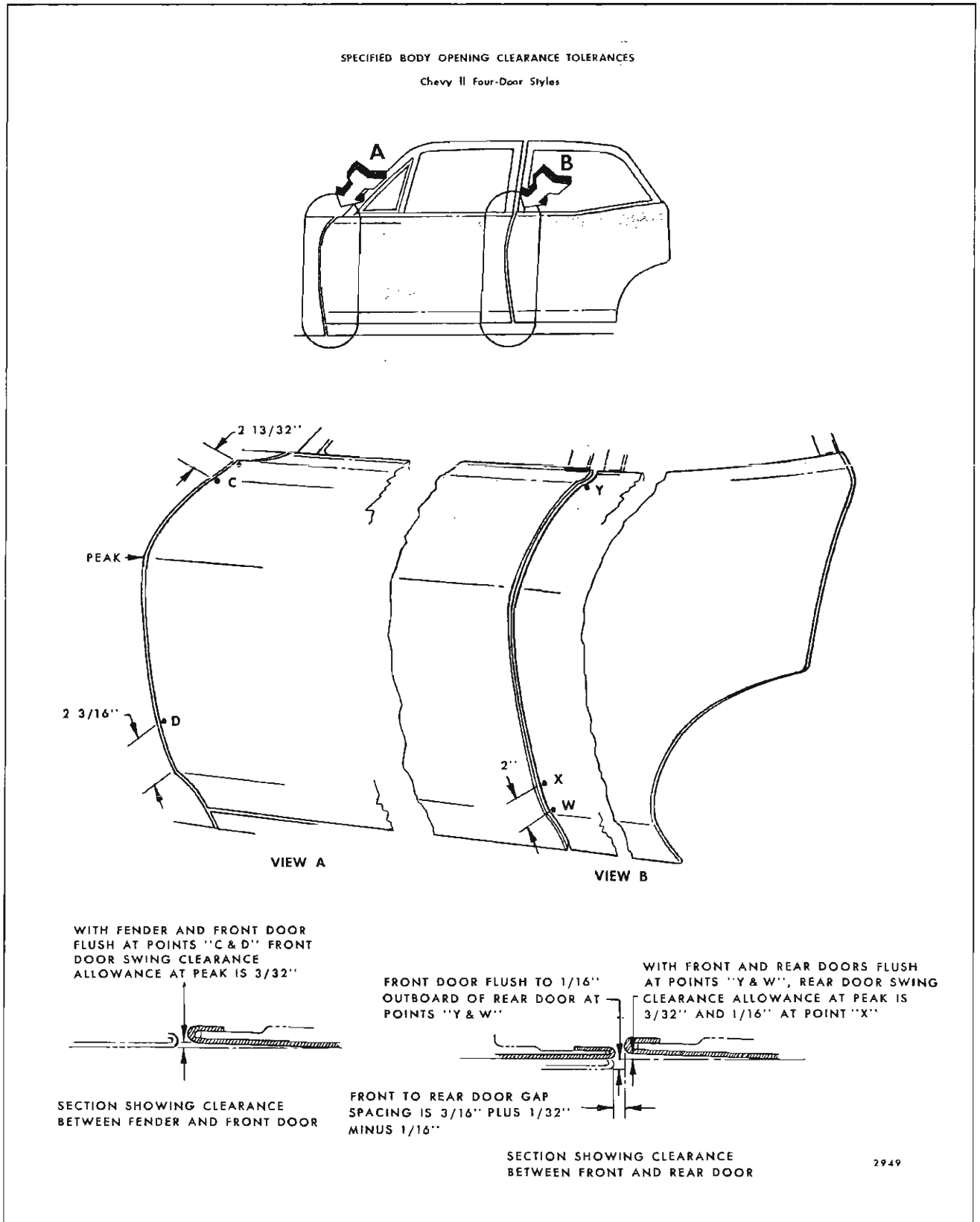
Fig. 6-17—Specified Body Opening Clearance Tolerances - "X" Styles
