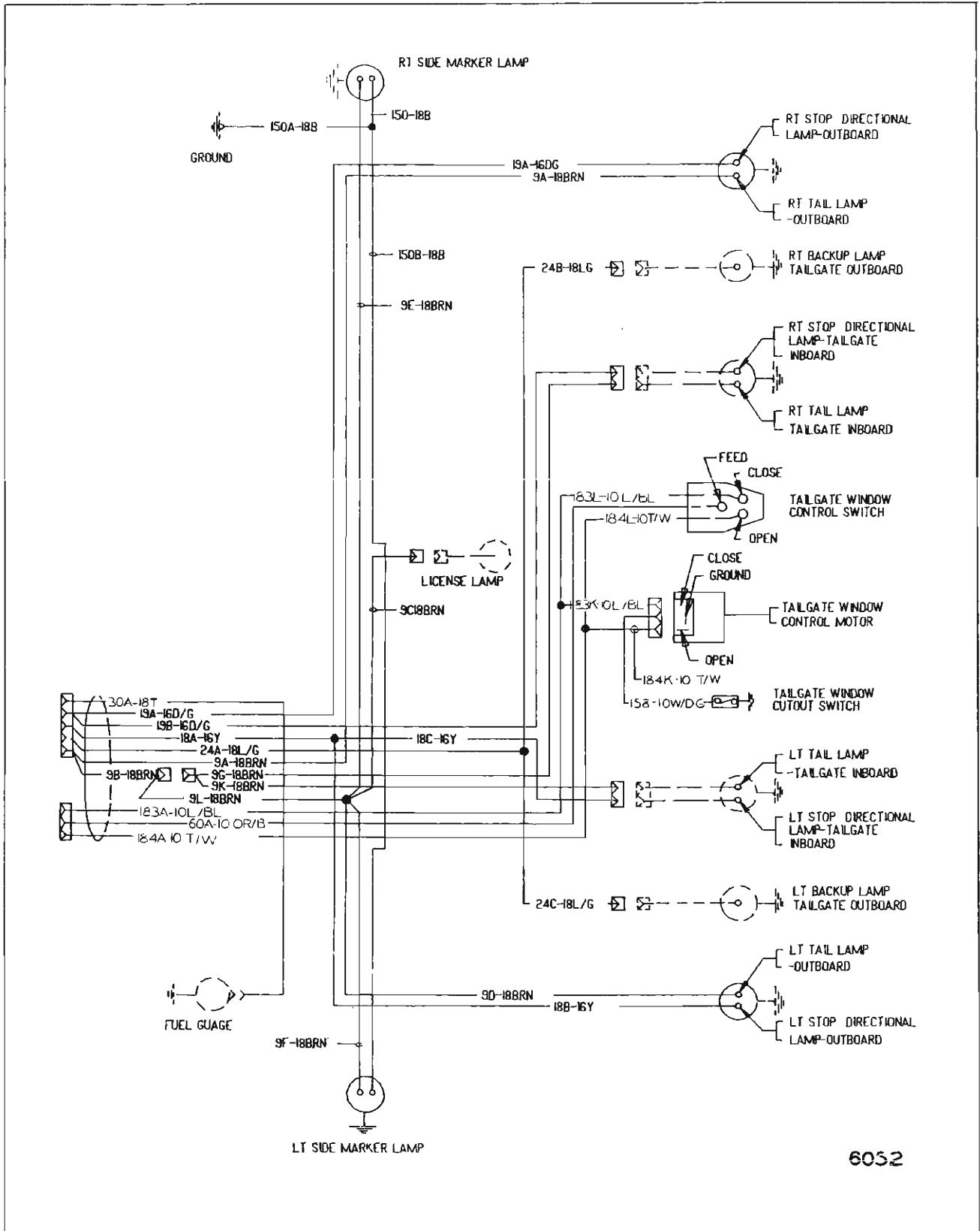
Fig. 16-20—Power Tail Gate Window Rear Wiring Circuit - Chevrolet "B" Styles
