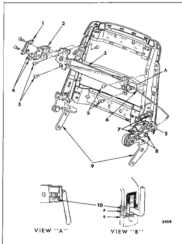
Fig. 15-57—Strato Reclining Seat Back Lock
