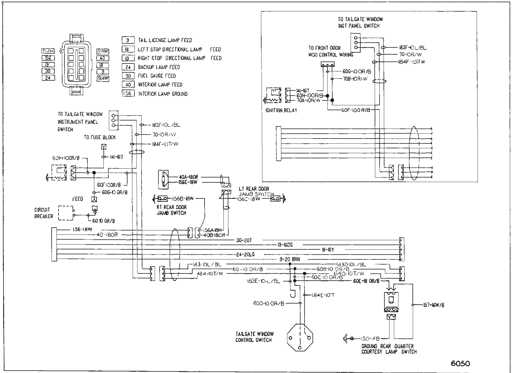
Fig. 16-19—Power Tail Gate Window Front Wiring Circuit - Chevrolet "B" Styles
