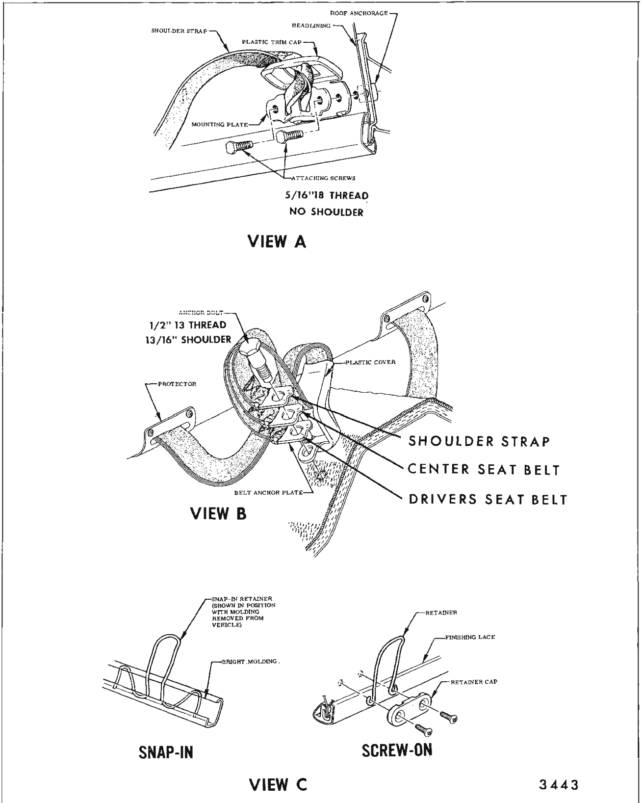
Fig. 15-103—Front Seat Shoulder Strap - All Styles Except Convertibles, "A-80" and "D" Styles (Refer to Fig. 15-102)
