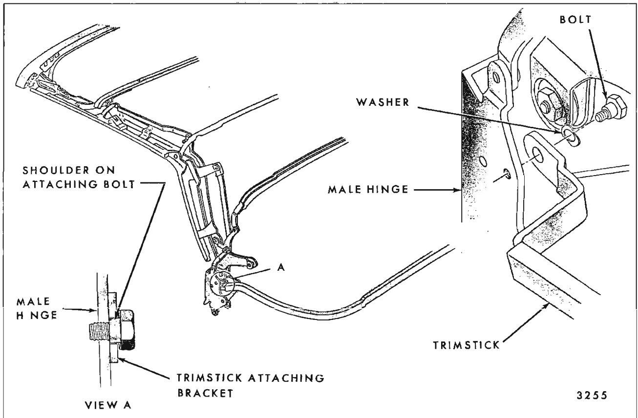
Fig. 13-45—Trimstick Attachment "B & C" Styles
