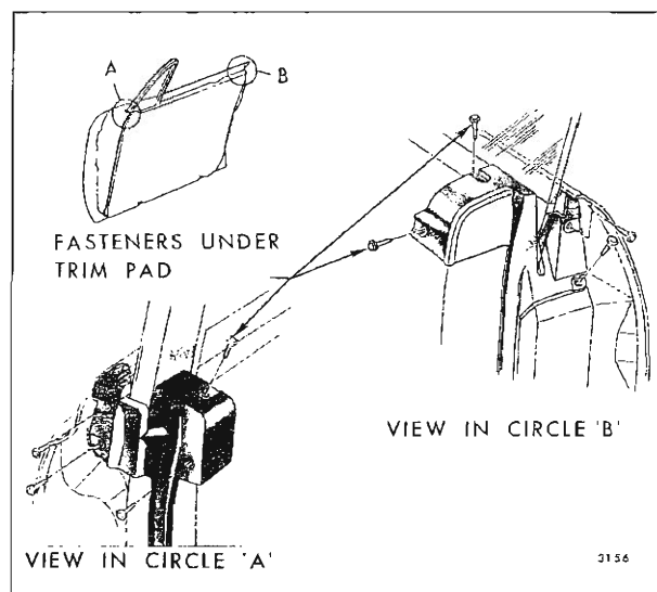
Fig. 6-3—Door Weatherstrip - Hardtop Styles
