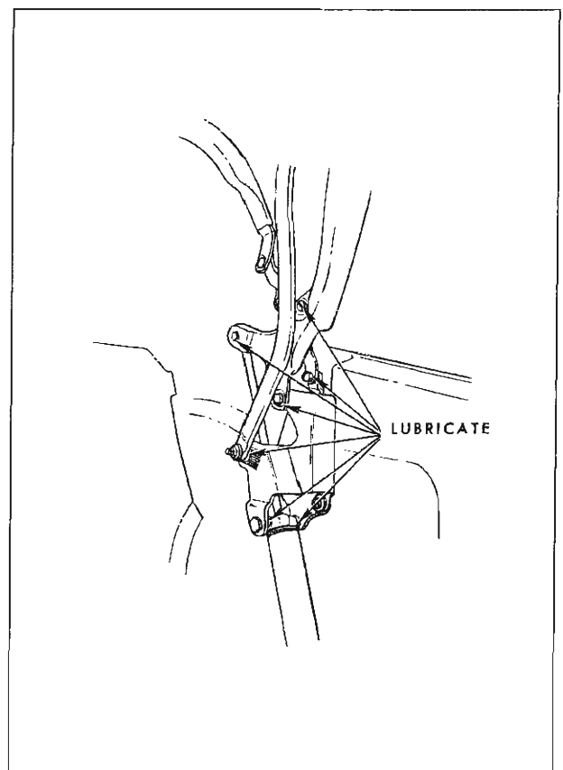
Fig. 2-16—"B" Convertible Hinge Lubrication
