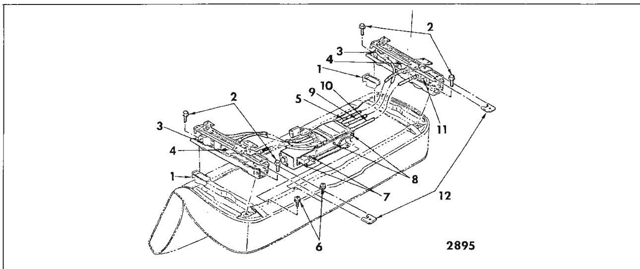
Fig. 15-9—Front Seat Assembly-Six-Way - "B & C" Full Width Seat
