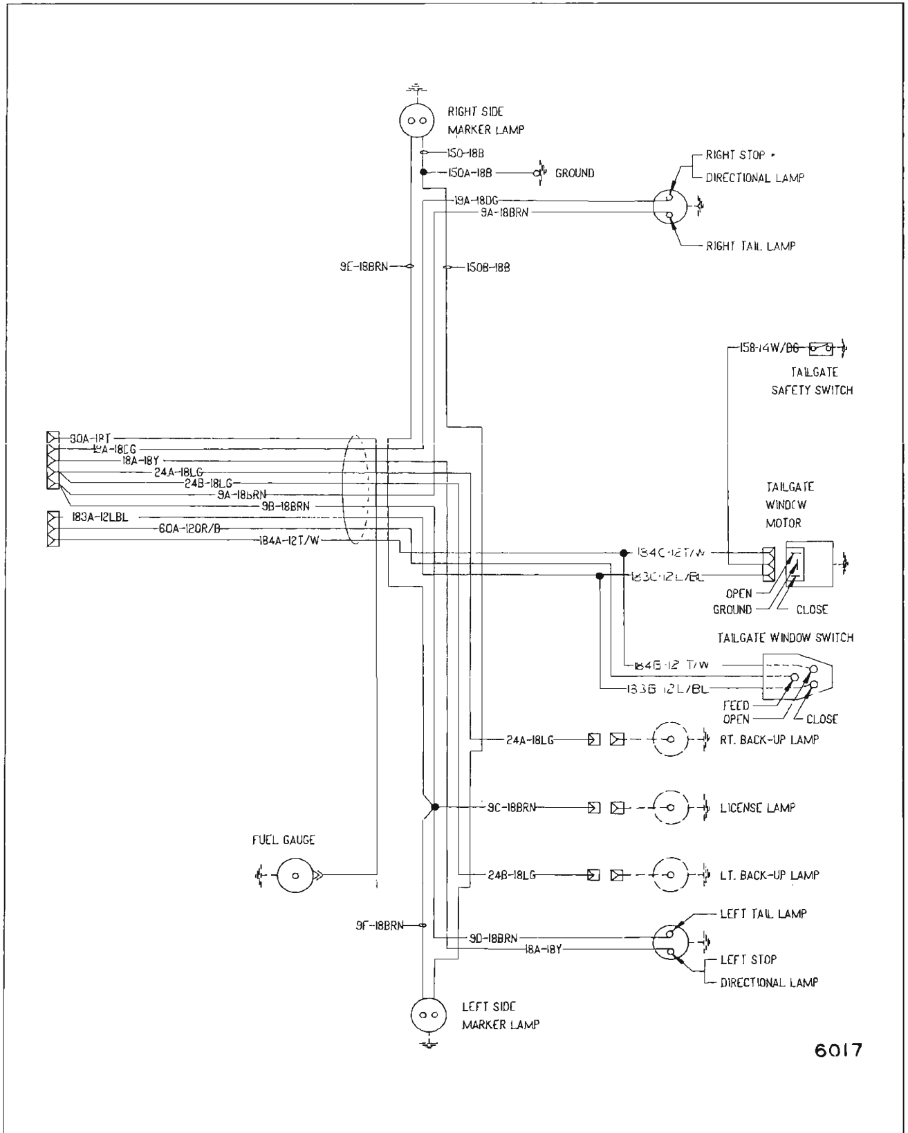
Fig. 16-14—Power Tail Gate Window Rear Wiring Circuit - Pontiac "A" Styles
