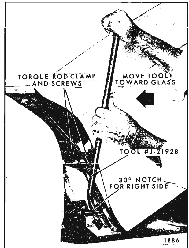
Fig. 5-26—Torque Rod Removal - Right Side
