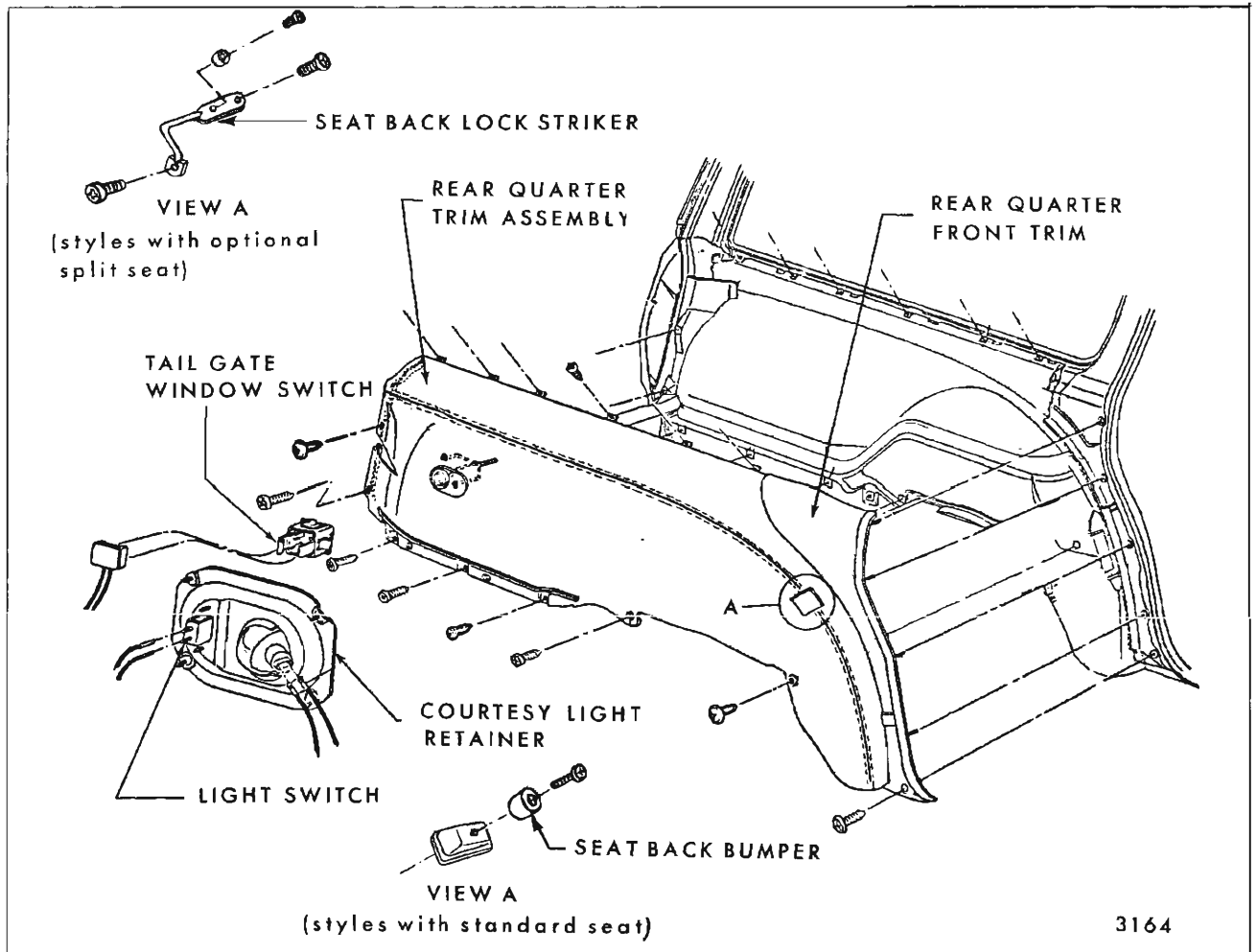
Fig. 14-32—Rear Quarter Trim Panel (Left Side) - "B" Station Wagon
