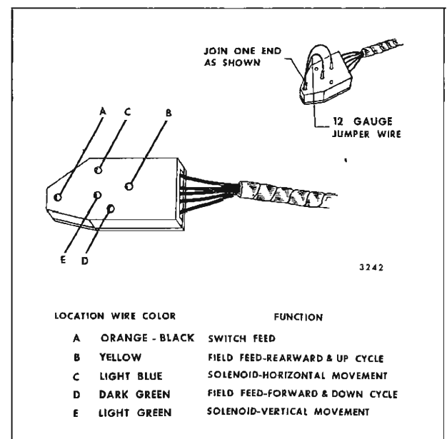
Fig. 16-32—Four-Way Seat Switch Block in Trim Panel
