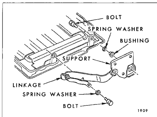
Fig. 15-75—Third Seat Back Panel and Linkage
