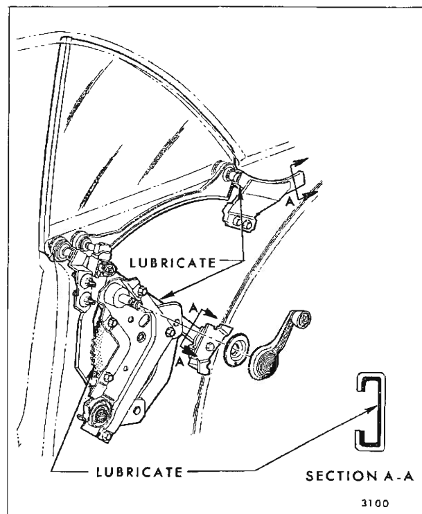
Fig. 2-10—"E" Styles - Quarter Window Regulator Lubrication
