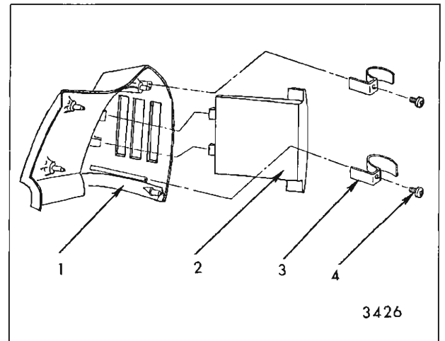
Fig. 16-39—Pontiac "G" Style Side Marker
