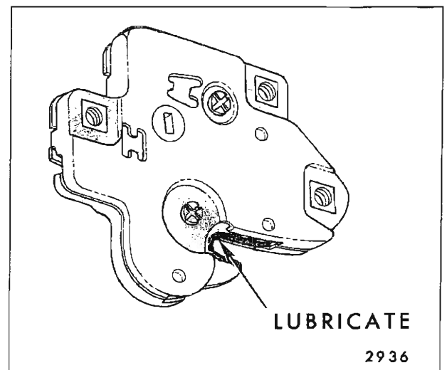
Fig. 2-20—Rear Compartment Lid Lock Lubrication
