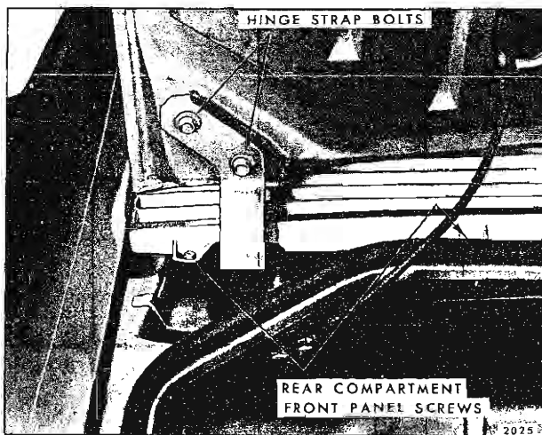
Fig. 8-2—Rear Compartment Lid Attachments - Oldsmobile and Buick "E" Styles
