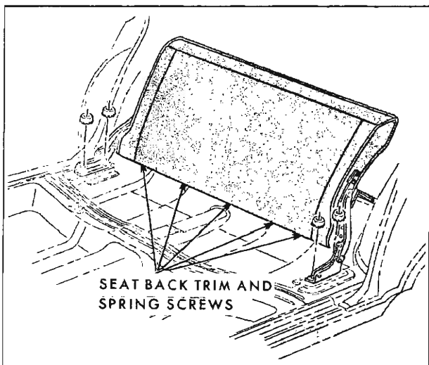
Fig. 15-77—Second Seat Back Trim and Spring Assembly
