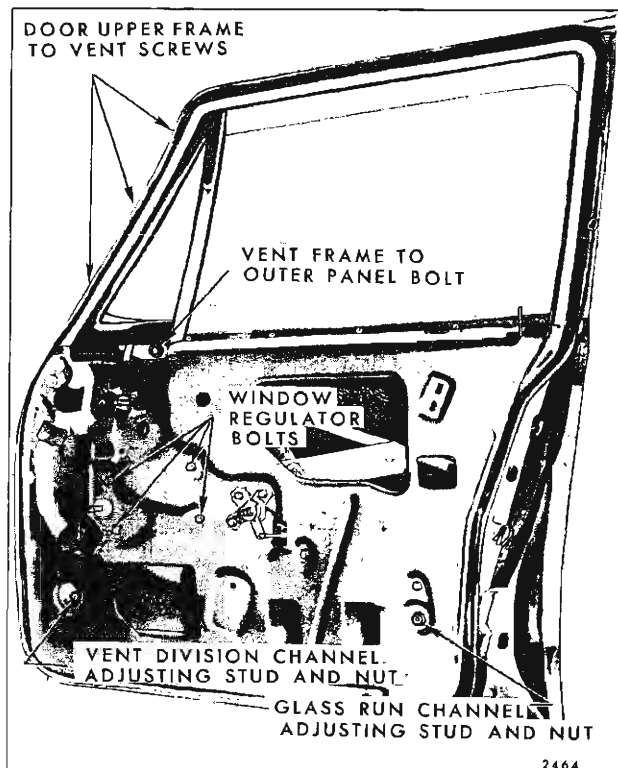
Fig. 6-100—Door Ventilator and Regulator Attachment - "A" Styles
