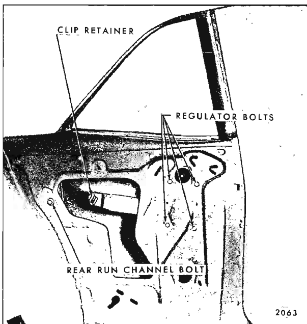
Fig. 7-42—Rear Quarter Hardware Attachment - "A, B, & X" Closed Styles
