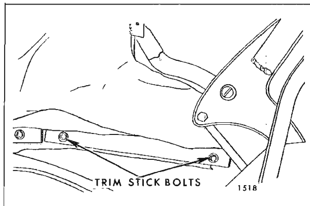
Fig. 13-10—Quarter Trimstick "F & Z" Styles
