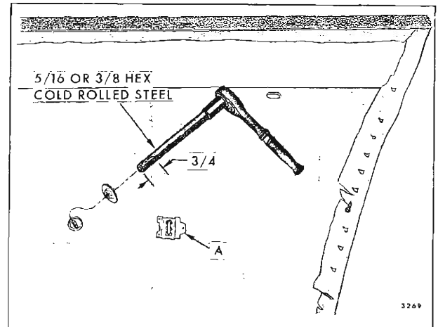
Fig. 14-16—Door Trim Pad Molding and Applique Removal
