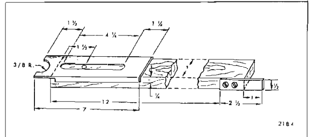
Fig. 13-5—Spacer Stick Fabrication
