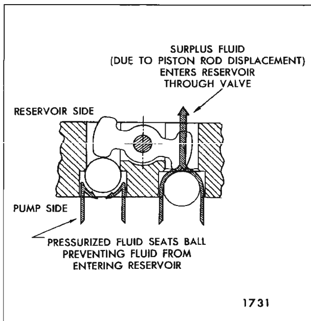
Fig. 13-65—Fluid Control Valve
