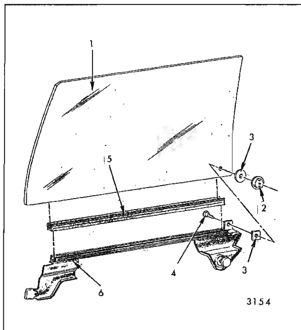
Fig. 6-79—Front Door Window Assembly - "A-39" Styles
