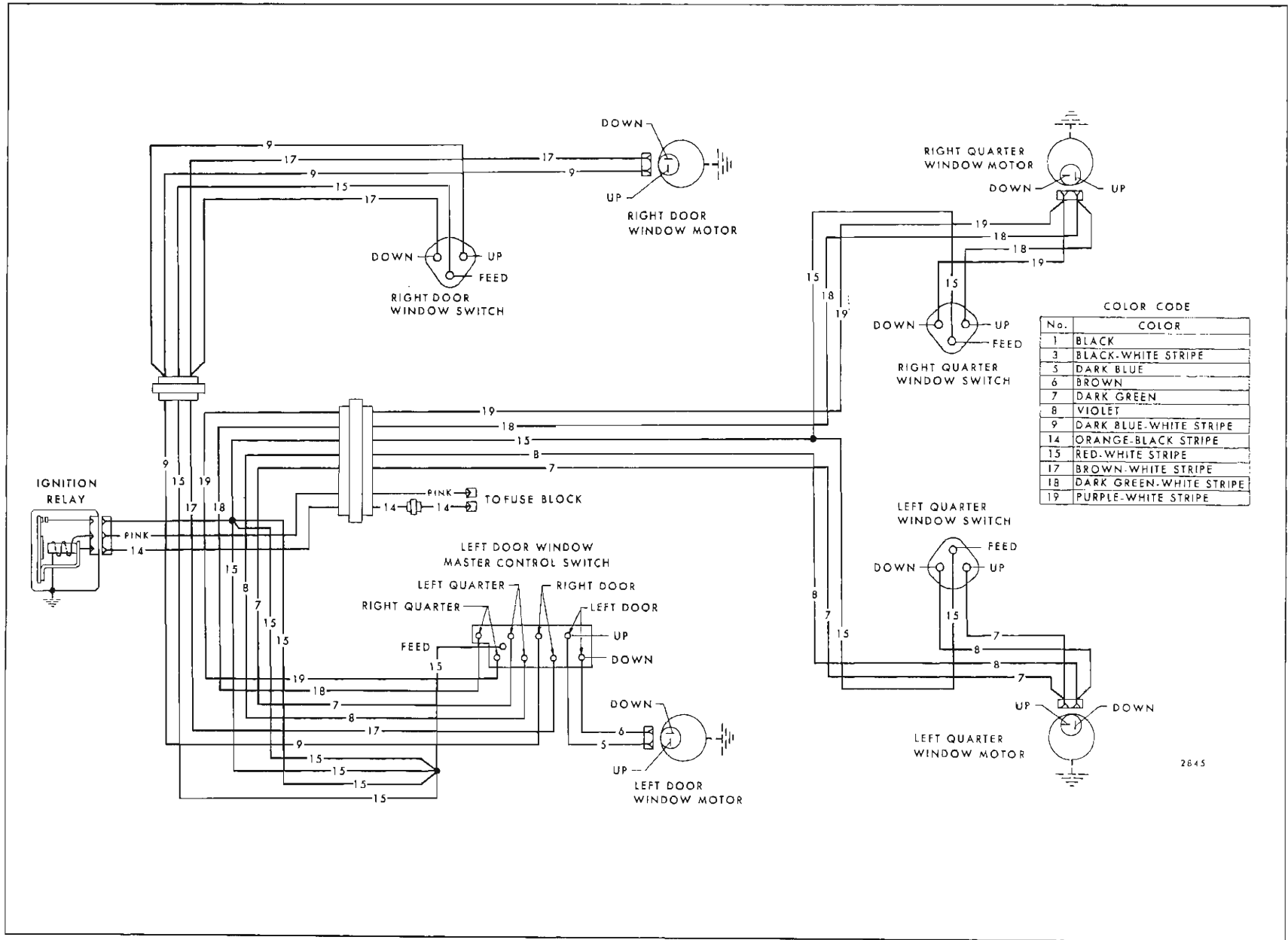
Fig. 16-4—Power Window Circuit - Buick "E" Styles
