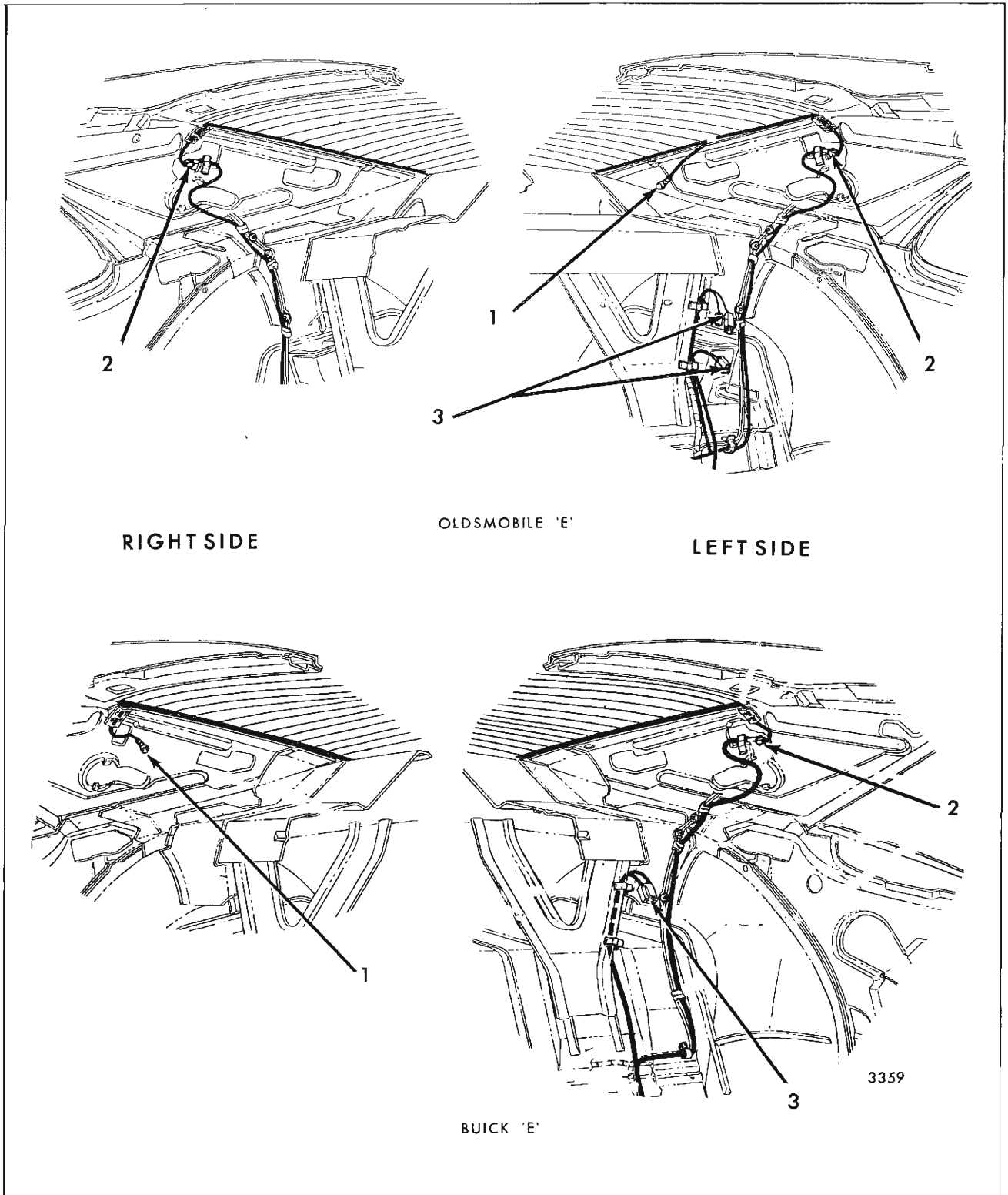
Fig. 16-47—Electric Back Window Grid Defogger
