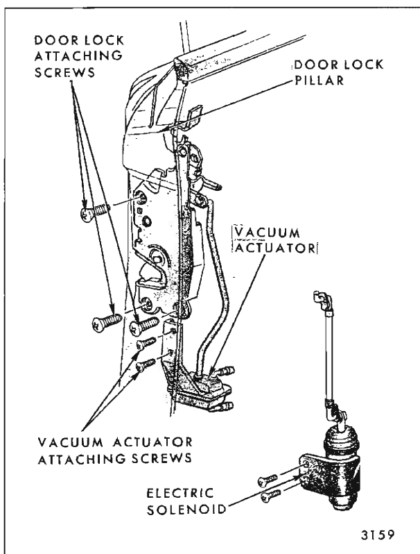
Fig. 6-27—Front Door Lock Vacuum Actuator or Electric Solenoid Installation
