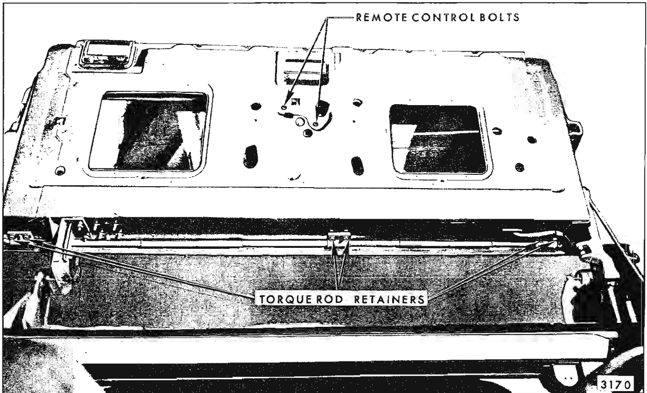
Fig. 9-22—Dual Gate Torque Rod Retention
