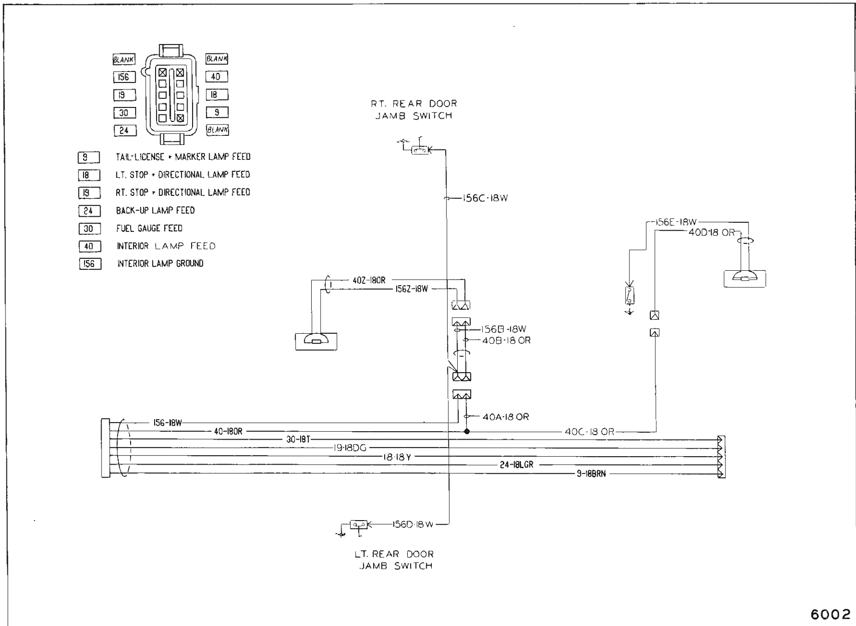
Fig. 16-17—Power Tail Gate Window Front Wiring Circuit - Buick "A" Styles
