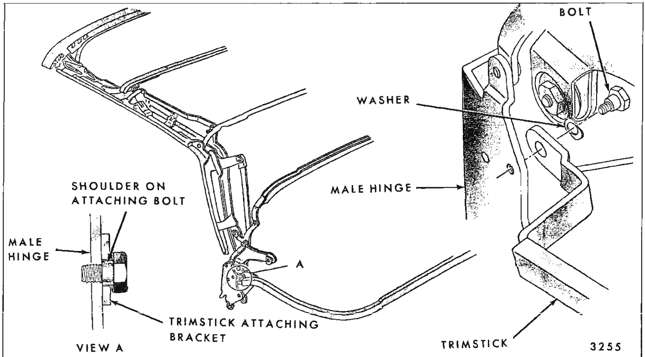
Fig. 13-29—Trimstick Attachment "B & C" Styles
