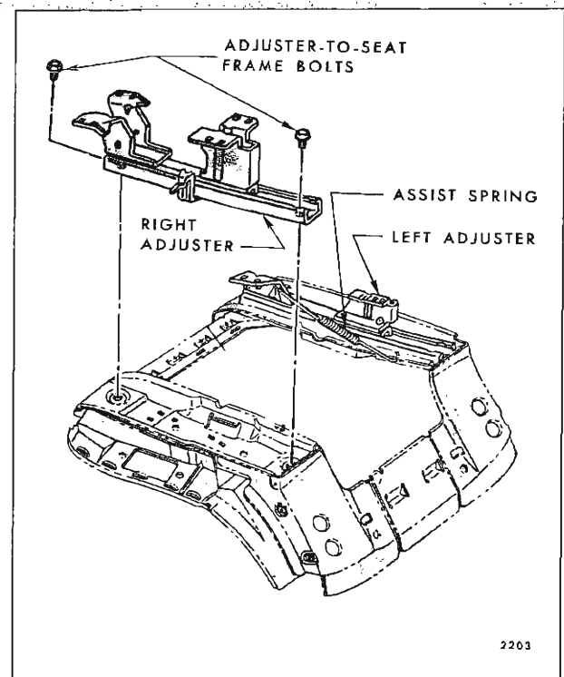
Fig. 15-43—Manual Bucket Seat Adjuster Removal
