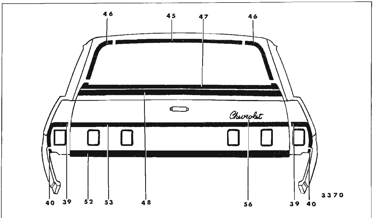
Fig. 17-26—Chevrolet 16636-46 Styles
