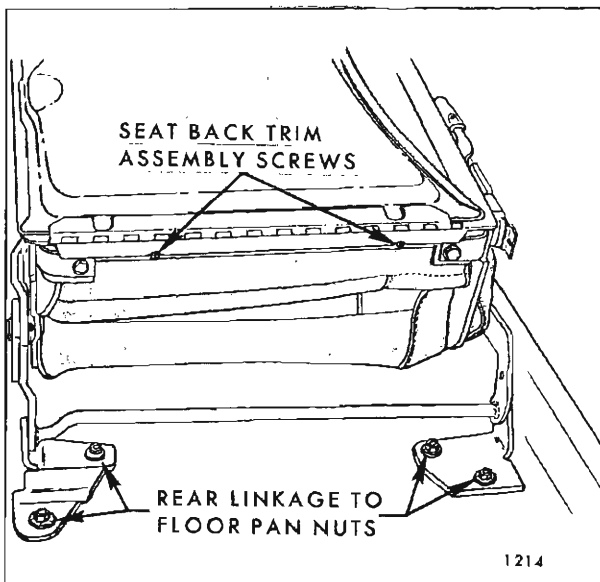
Fig. 15-85—Folding Second Seat Rear Linkage
