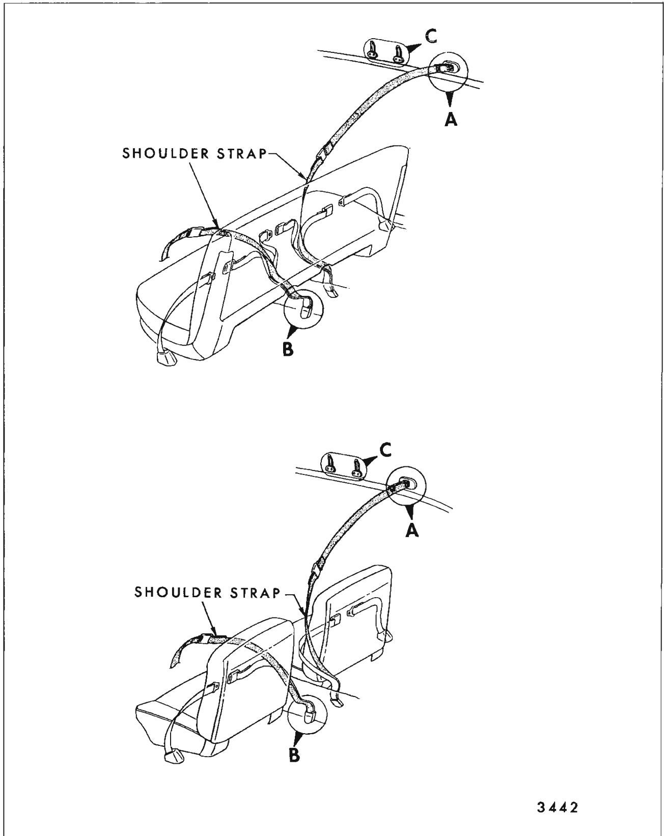
Fig. 15-102—Front Seat Shoulder Strap - All Styles Except Convertibles, "A-80" and "D" Styles
