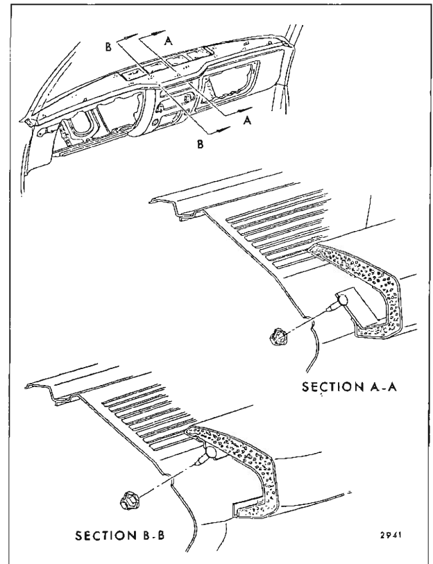
Fig. 5-23—Instrument Panel Cover - Chevrolet "Z" Styles
