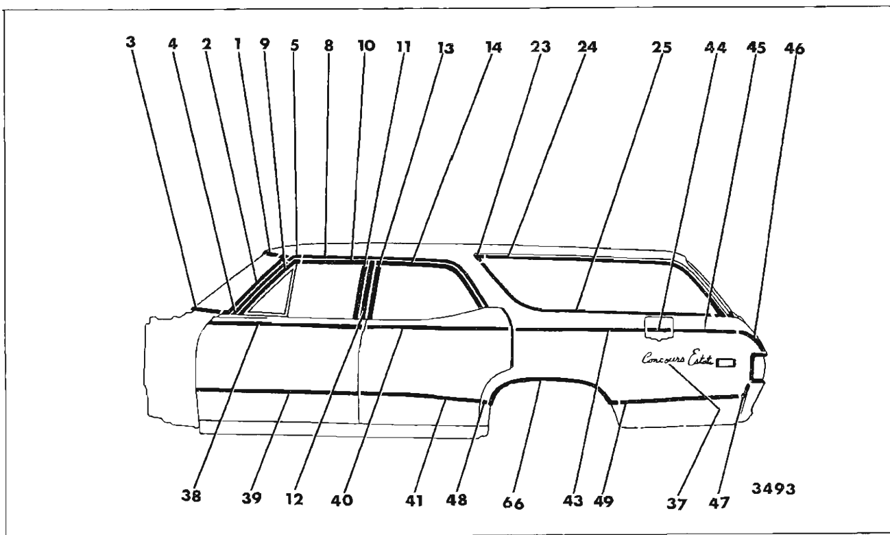
Fig. 17-12—Chevrolet 13836-46 Styles
