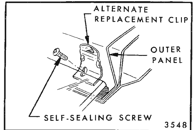
Fig. 17-5—Reveal Molding Clip Alternate Replacement
