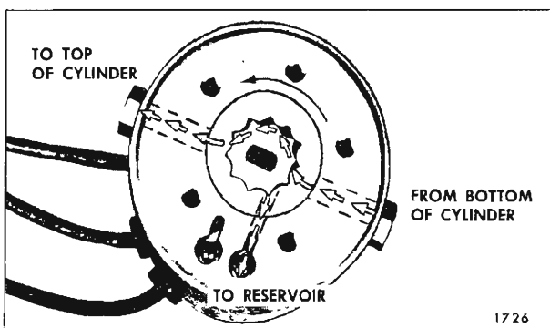
Fig. 13-62—Operation of Pump to Lower Top
