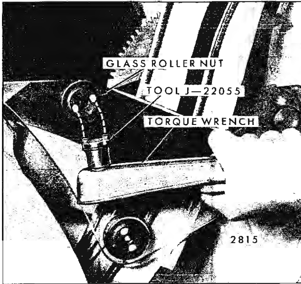
Fig. 7-21—Quarter Window Roller
