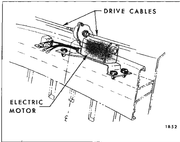
Fig. 13-73—Folding Top Electric Power Unit "Z" Styles
