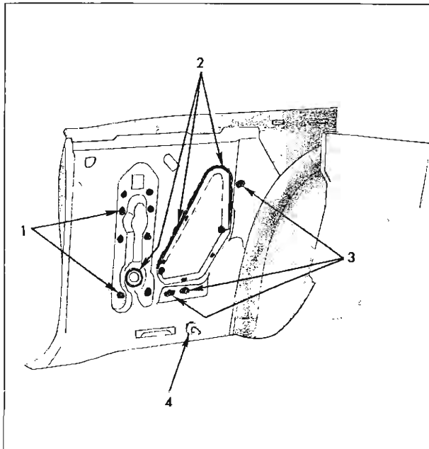
Fig. 7-2—Rear Quarter Typical Inner Panel Sealing - "67" Styles
