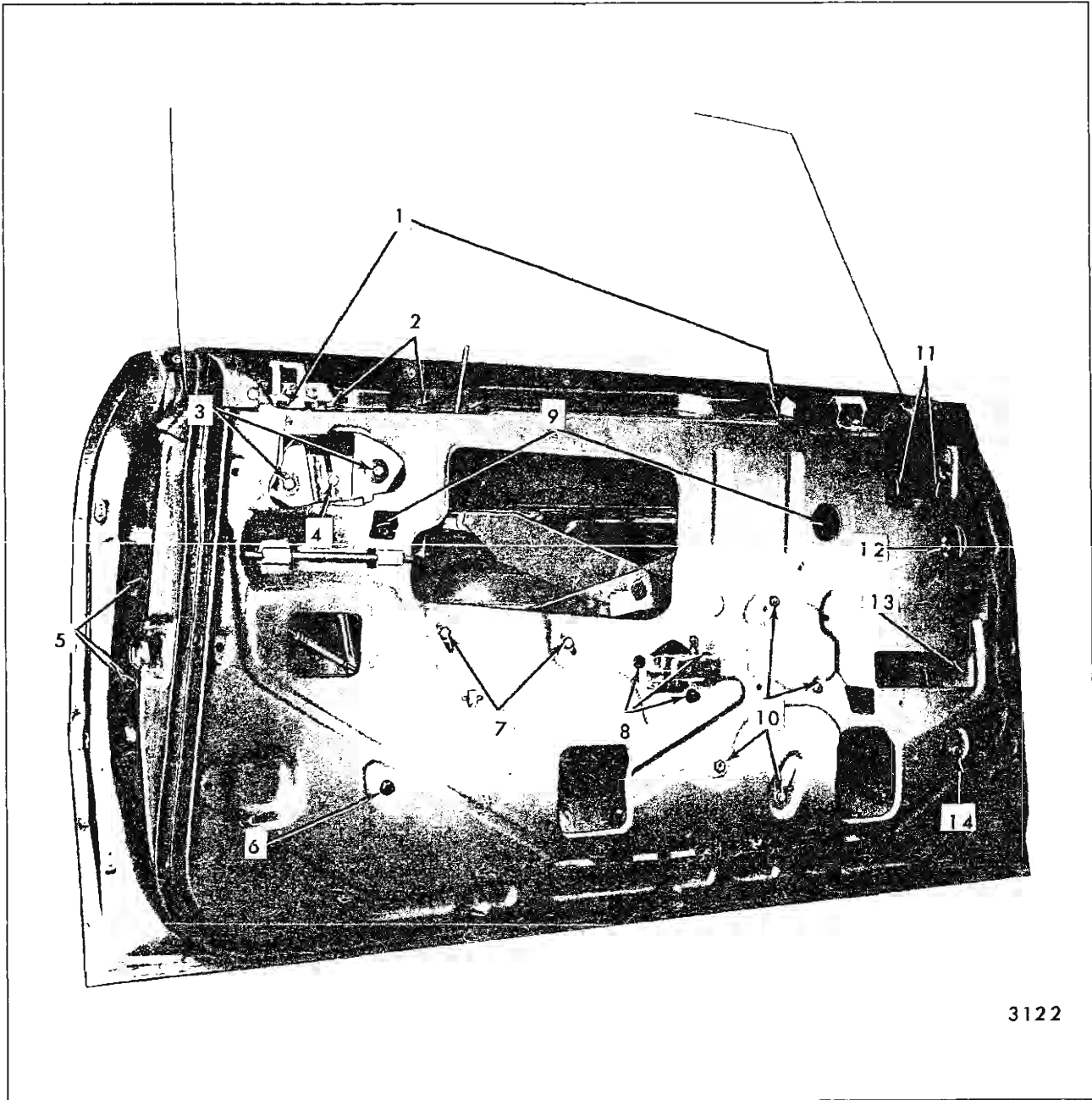
Fig. 6-42—Front Door Hardware - "G-57" Style Shown, "A-37, 67 and 87" Style Similar
