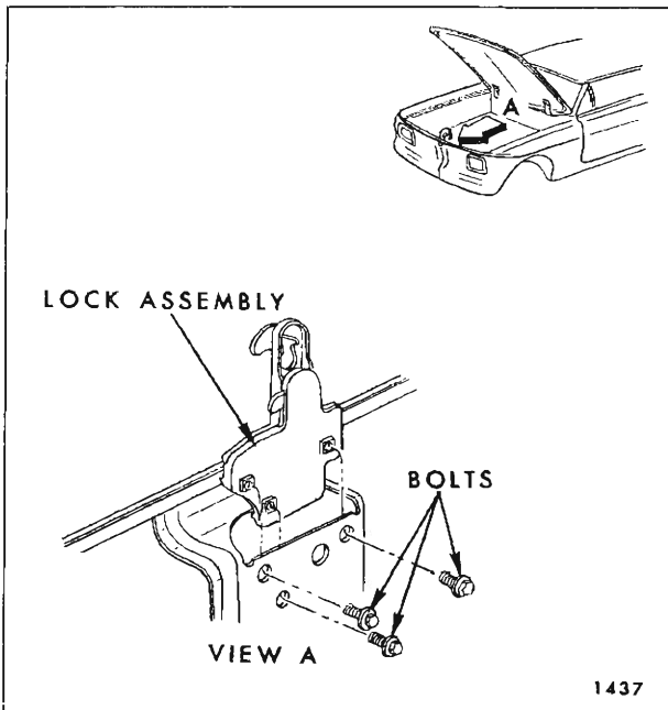
Fig. 5-29—Front Compartment Lid Lock
