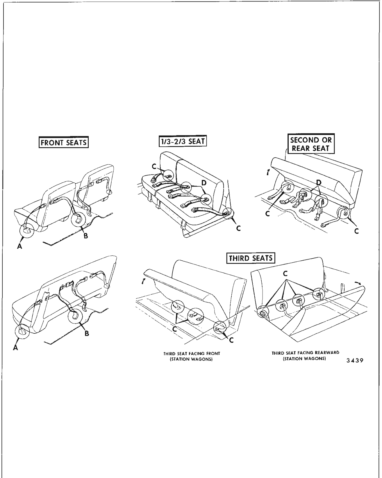
Fig. 15-99—Front and Rear Seat Belts (Including Station Wagon Second and Third Seats)
