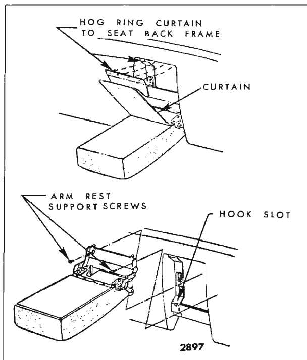
Fig. 15-38—Front Seat Back Center Arm Rest
