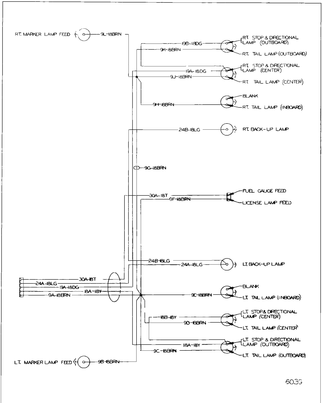
Fig. 16-60—Wiring Diagram Rear - Pontiac "B" Styles
