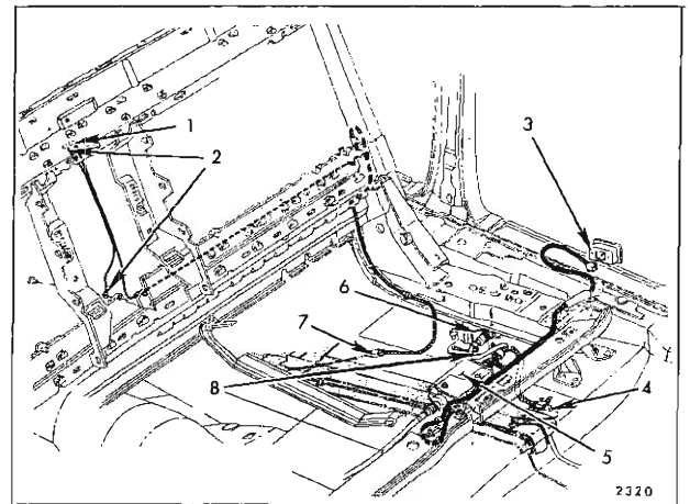
Fig. 16-25—Horizontal Bench Seat Wiring
