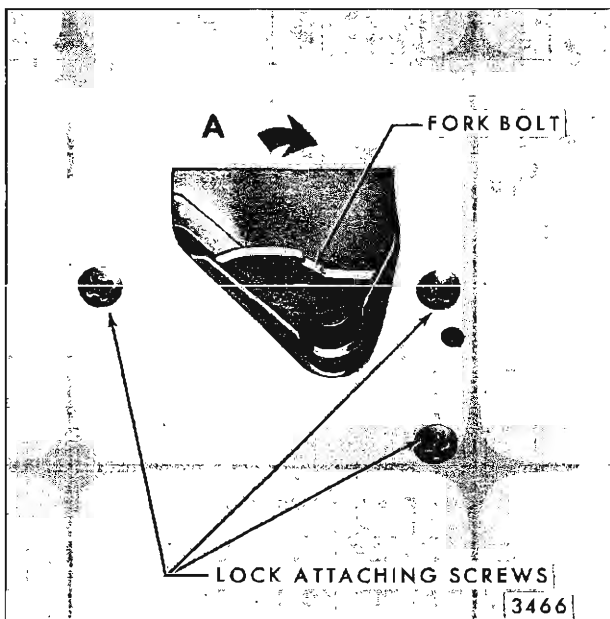
Fig. 9-5—Dual Tail Gate Right Upper Lock Engagement
