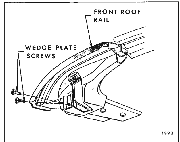
Fig. 13-85—Front Roof Rail Wedge Plate - "Z" Styles
