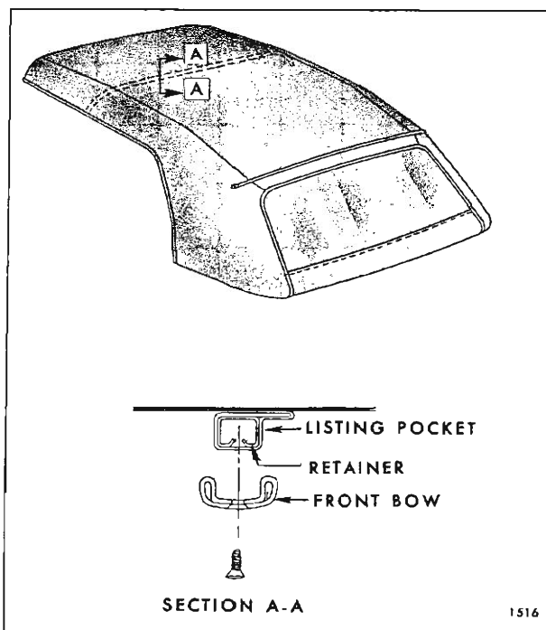
Fig. 13-3—Listing Pocket Retainer
