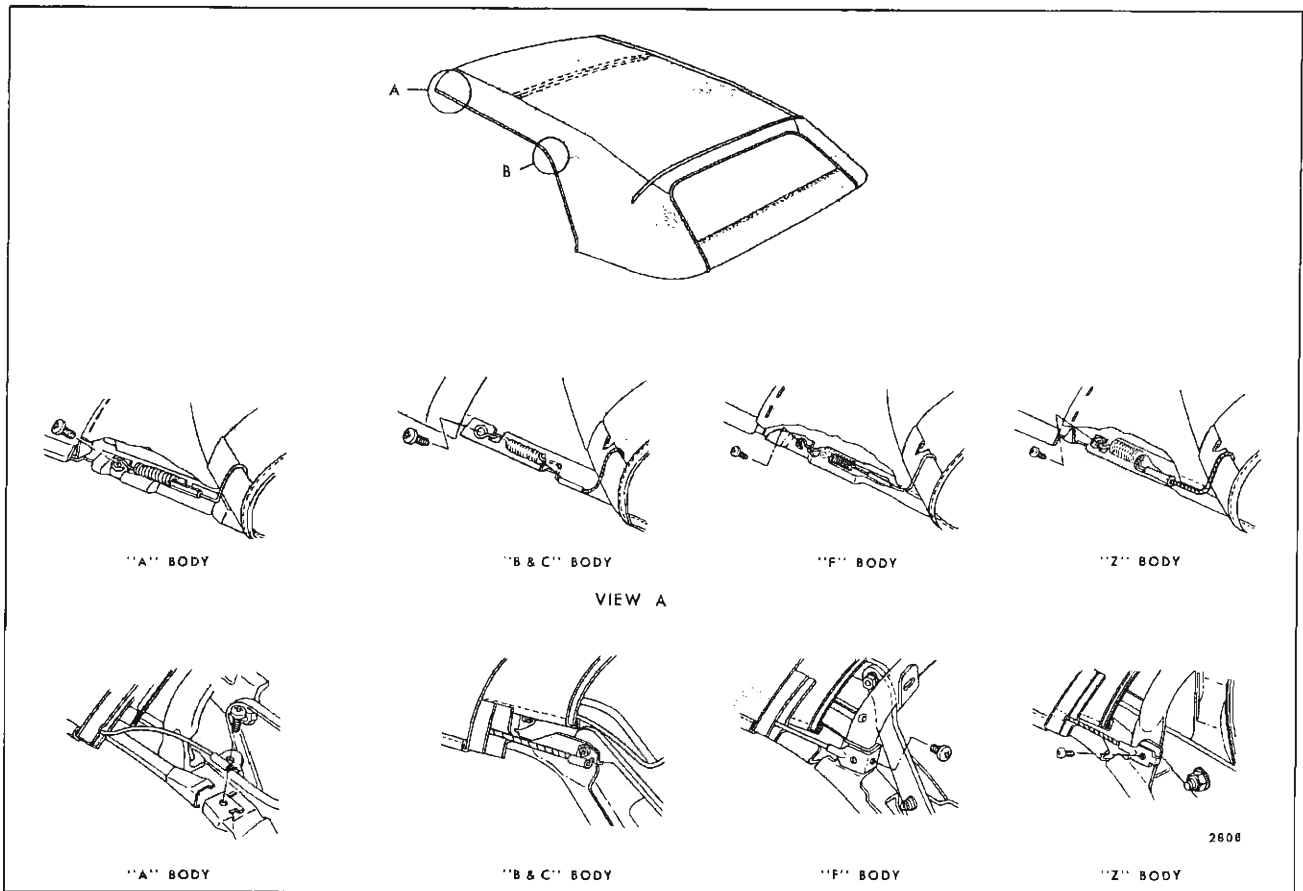
Fig. 13-2—Hold Down Cable Attachment
