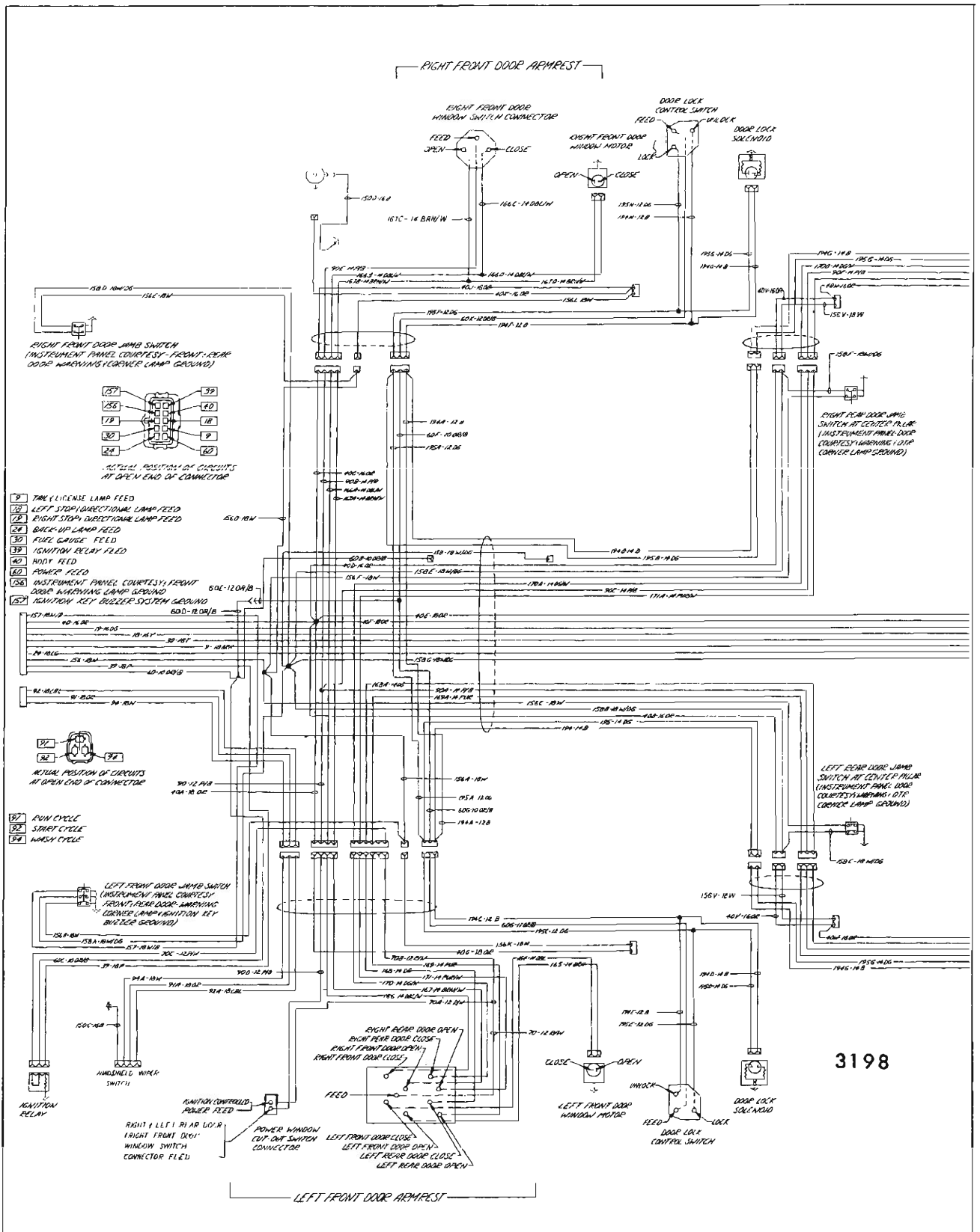
Fig. 16-70—Wiring Diagram - Cadillac "68069" Style
