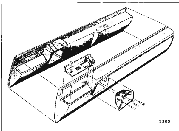
Fig. 14-12—Door Arm Rest - "E" Style Shown, Cadillac "C" Styles Typical
