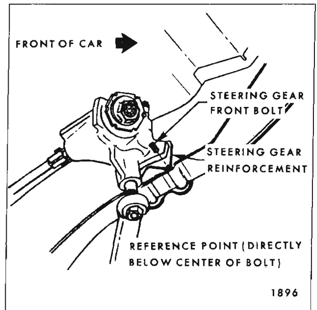
Fig. 3-4—Reference Point at Steering Gear Reinforcement
