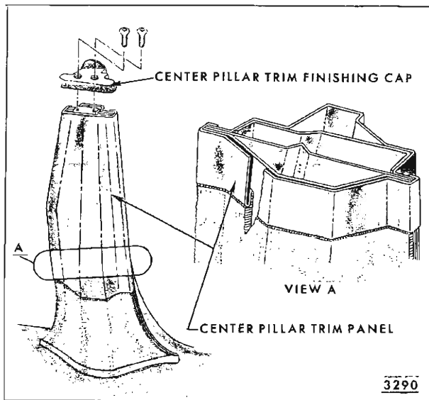
Fig. 14-38—Center Pillar Trim "A-B and C-39, 49" Styles. (26239 Custom, 48439, 682-68349 Styles Shown, Others Similar)
