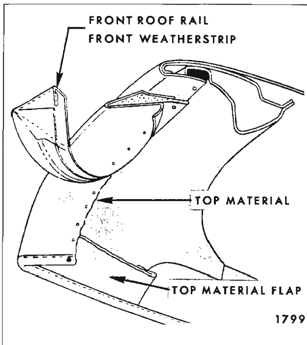
Fig. 13-39—Top Cover at Front Roof Rail
