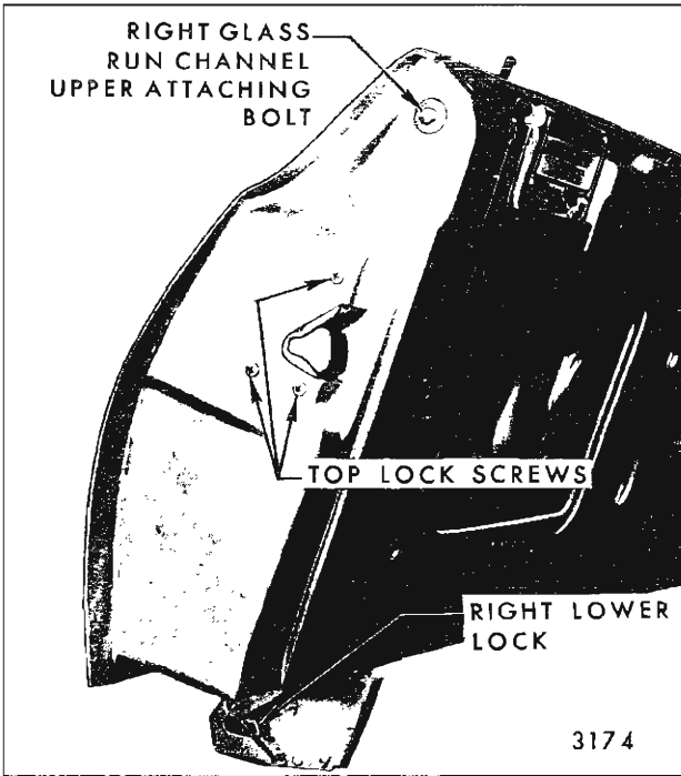
Fig. 9-30—Dual Tail Gate Lock Attachments - Right Side
