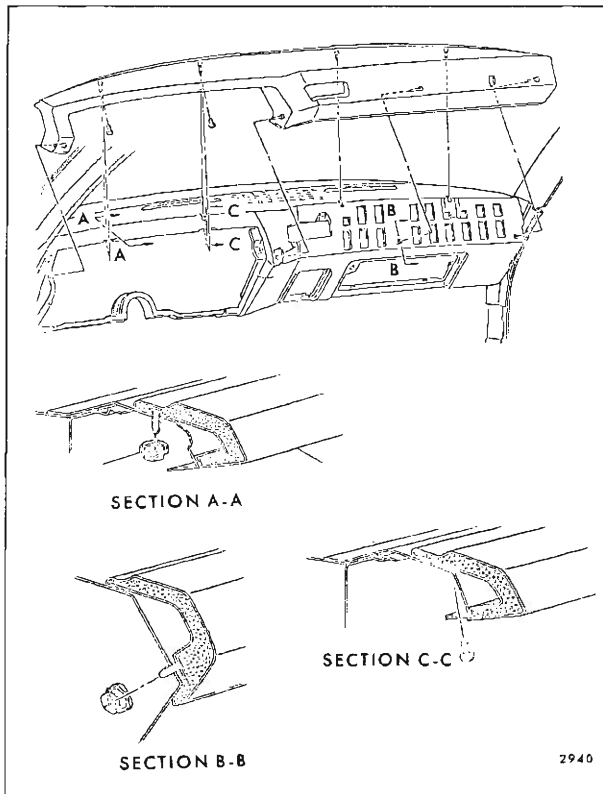
Fig. 5-22—Instrument Panel Cover - Chevrolet "X" Styles
