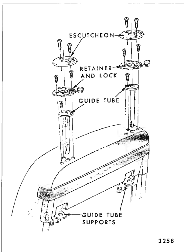
Fig. 15-52—Head Restraint - Strato Seats
