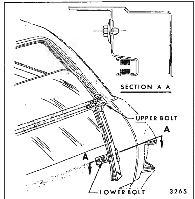
Fig. 9-19—Tail Gate Lower Glass Run Channel Attachment
