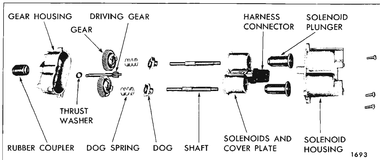
Fig. 15-14—Four-Way Seat Adjuster Transmission
