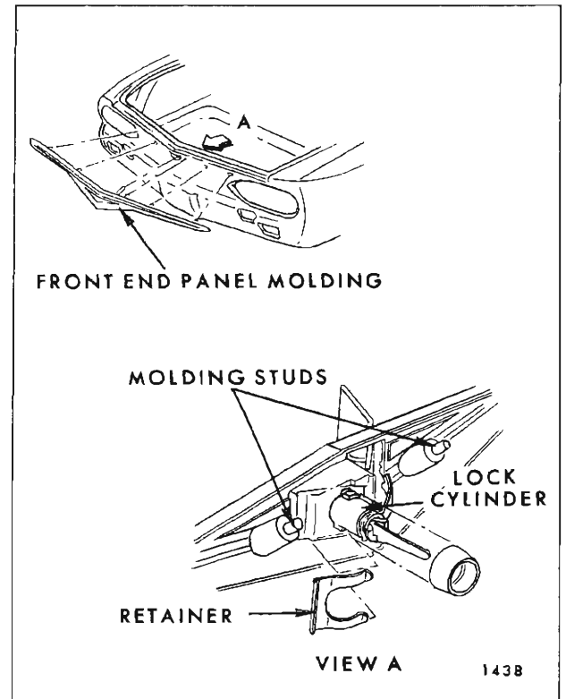
Fig. 5-28—Front Compartment Lid Lock Removal
