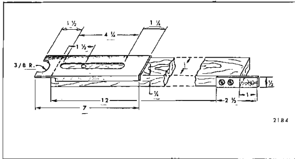
Fig. 13-42—Spacer Stick Fabrication
