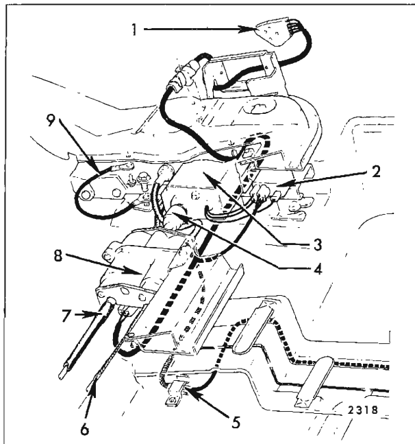
Fig. 16-28—Four-Way Bench Seat Wiring - "A" Body Styles
