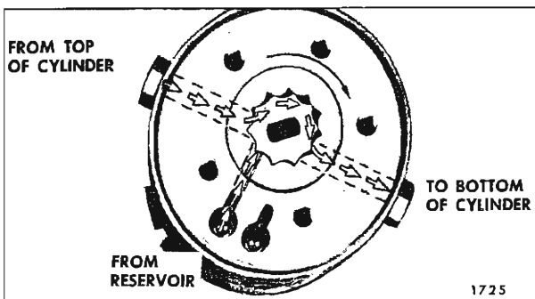
Fig. 13-61—Operation of Pump to Raise Top
