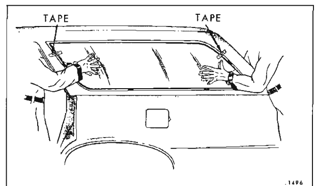
Fig. 4-9—Stationary Quarter Window Installation
