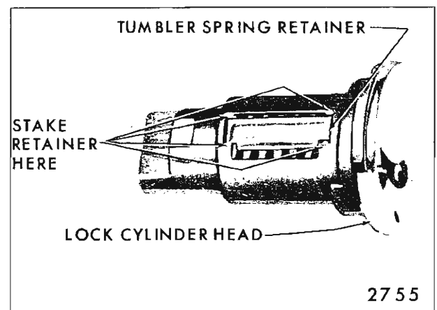
Fig. 1-6—Installing Spring Retainer
