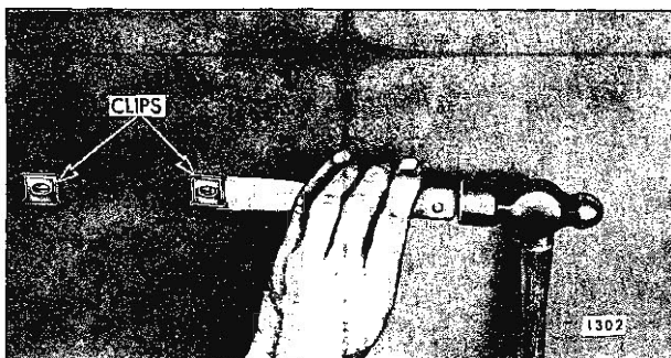
Fig. 17-4—Removal of Bath-Tub Type Molding Clip
