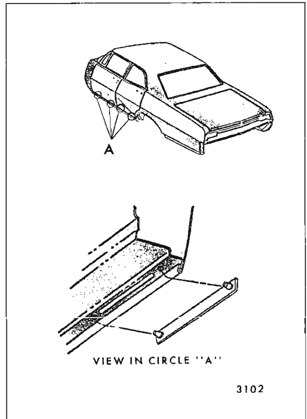
Fig. 6-5—Door Bottom Drain Hole Sealing Strips
