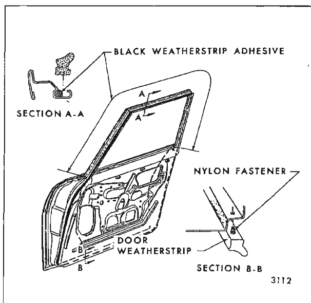
Fig. 6-2—Door Weatherstrip - "A & X" Closed Styles
