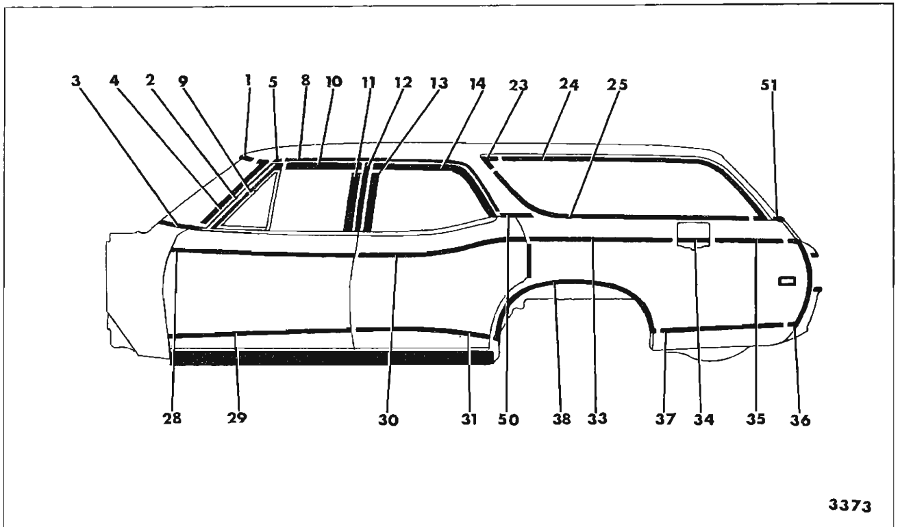
Fig. 17-40—Pontiac 23936 Style
