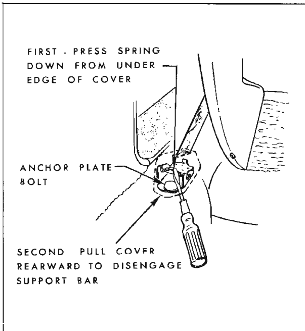
Fig. 15-96—Front Seat Belt Self-Locking Retractor - Removal
