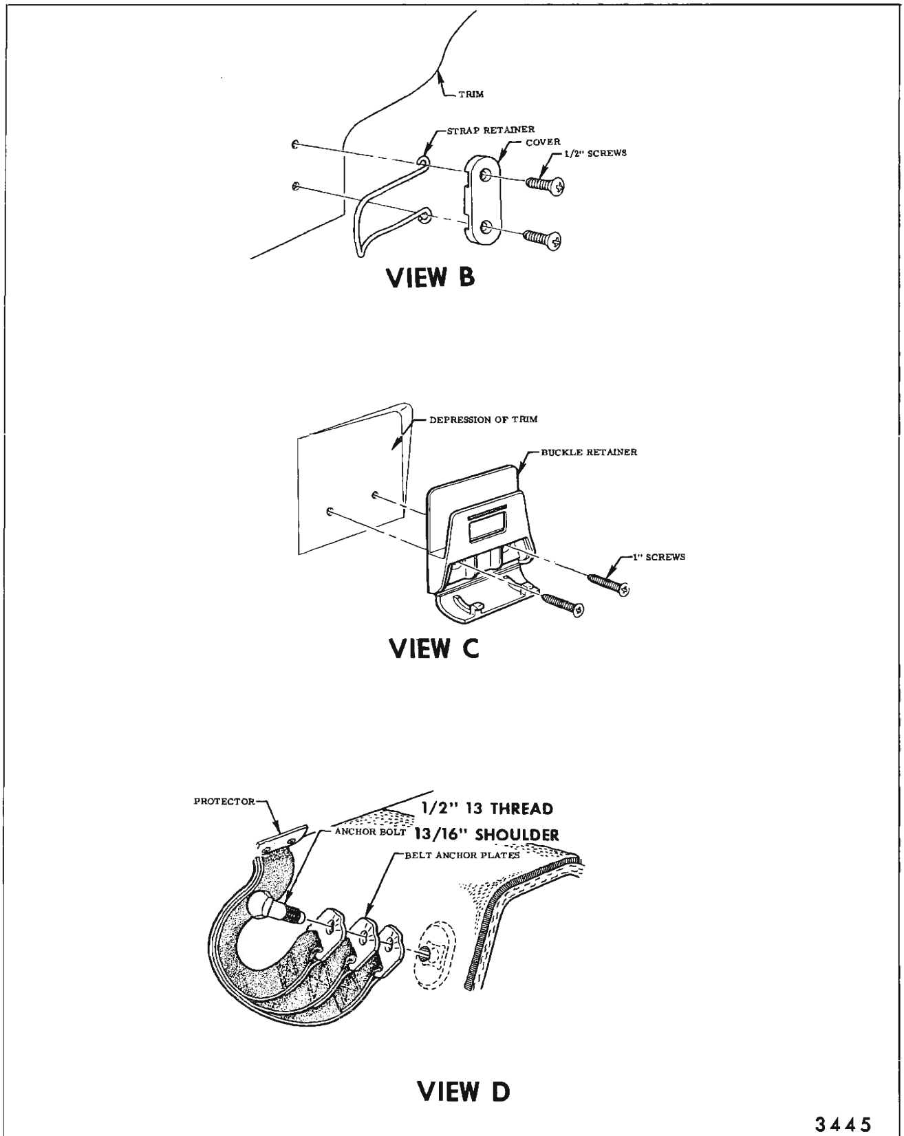
Fig. 15-105—Front Seat Shoulder Strap - "A-80" Styles (Refer to Fig. 15-104)
