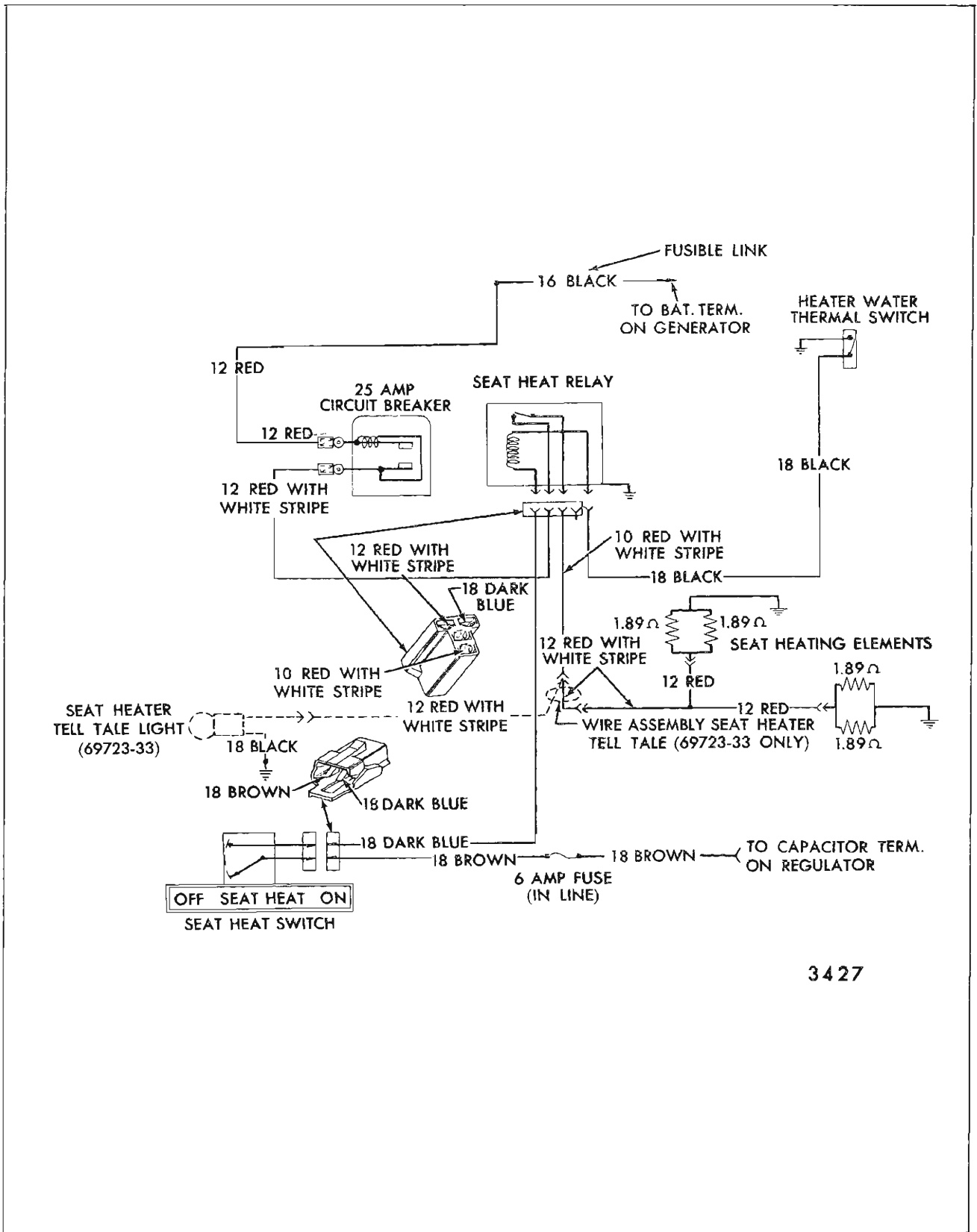
Fig. 16-46—Electric Seat Warmer
