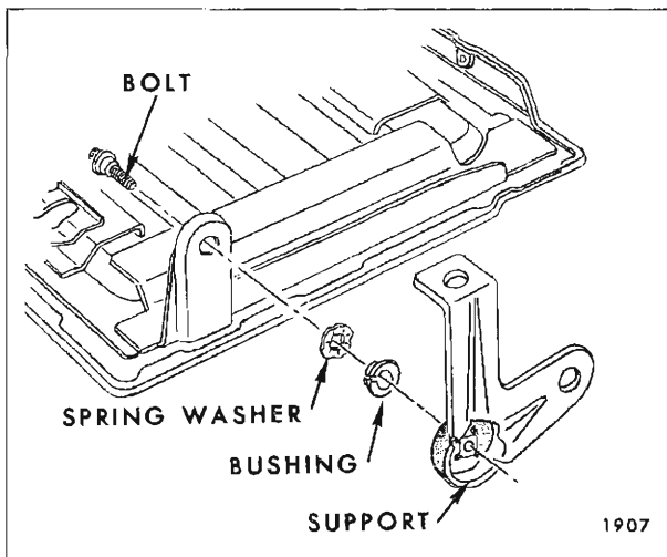
Fig. 15-73—Third Seat Cushion Panel and Support
