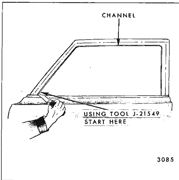
Fig. 6-102—Door Window Glass Run Channel Removal
