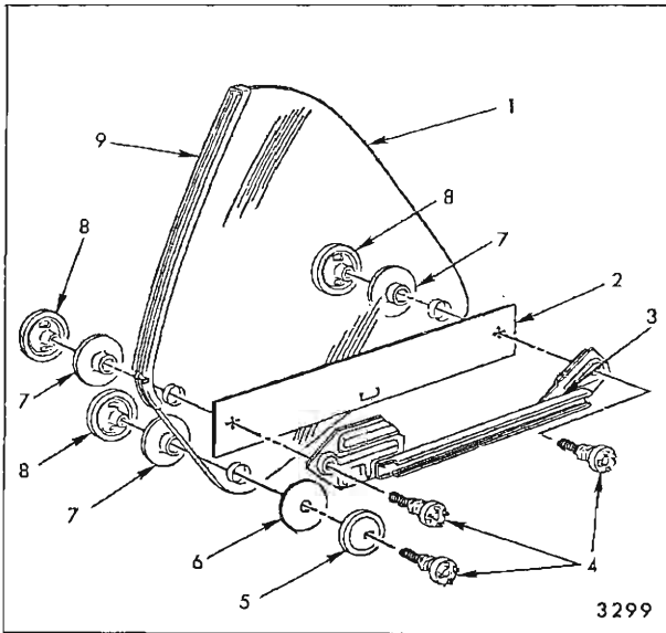
Fig. 7-41—Rear Quarter Window Assembly - "Z-67" Style
