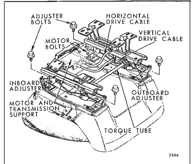
Fig. 15-45—Four-Way Bucket Seat Assembly
