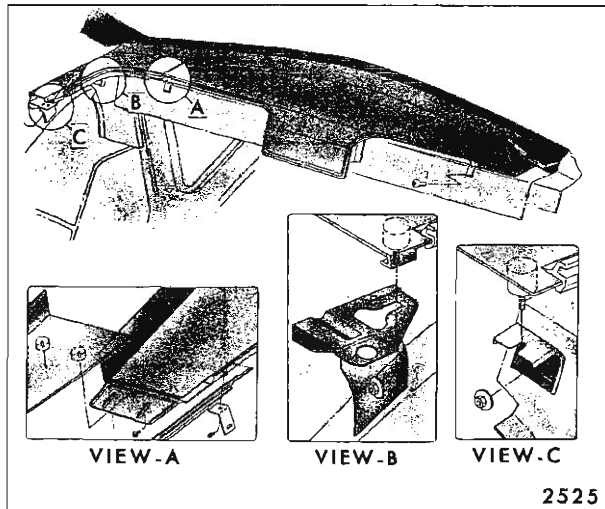
Fig. 14-43—Compartment Shelf Trim Panel - Cod. "E" Styles
