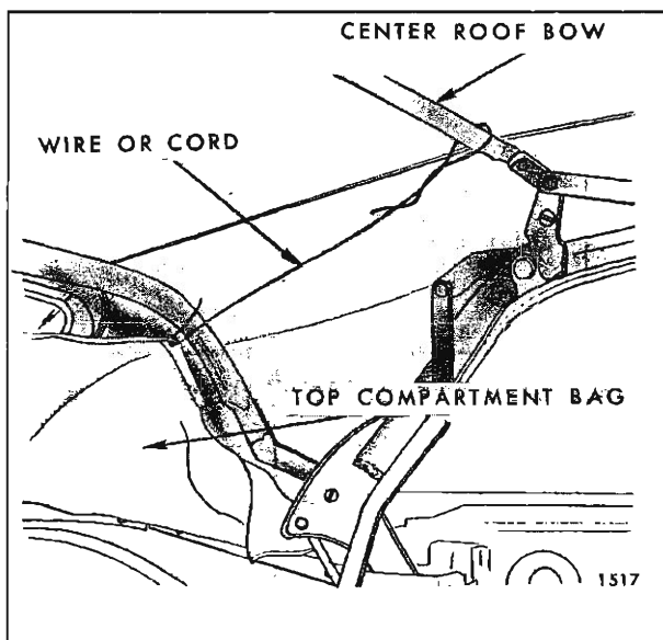
Fig. 13-30—Raising Folding Top Compartment Bag
