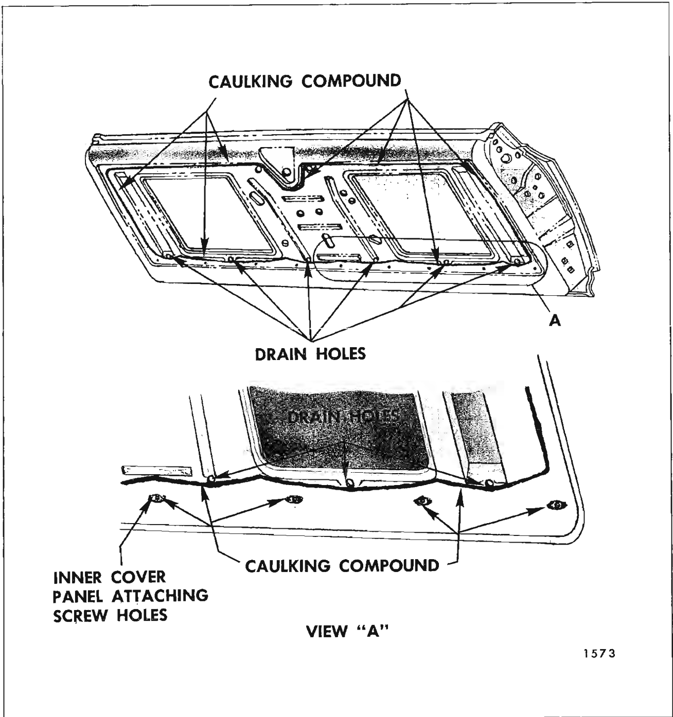
Fig. 9-2—Tail Gate Sealing
