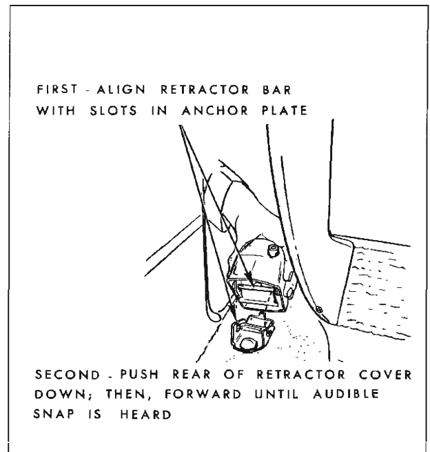
Fig. 15-97—Front Seat Belt Self-Locking Retractor - Installation
