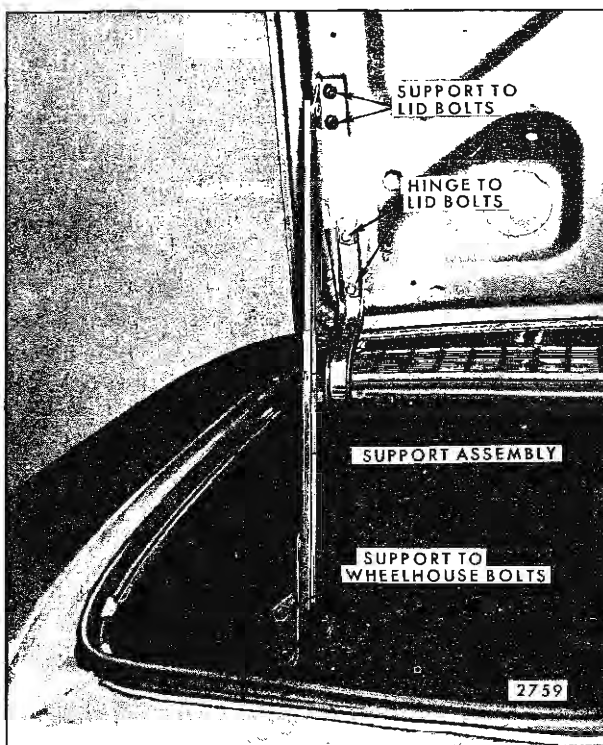
Fig. 8-11—Engine Compartment Lid Support - "Z" Styles
