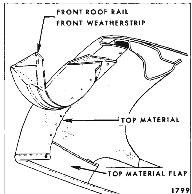
Fig. 13-23—Top Cover at Front Roof Rail
