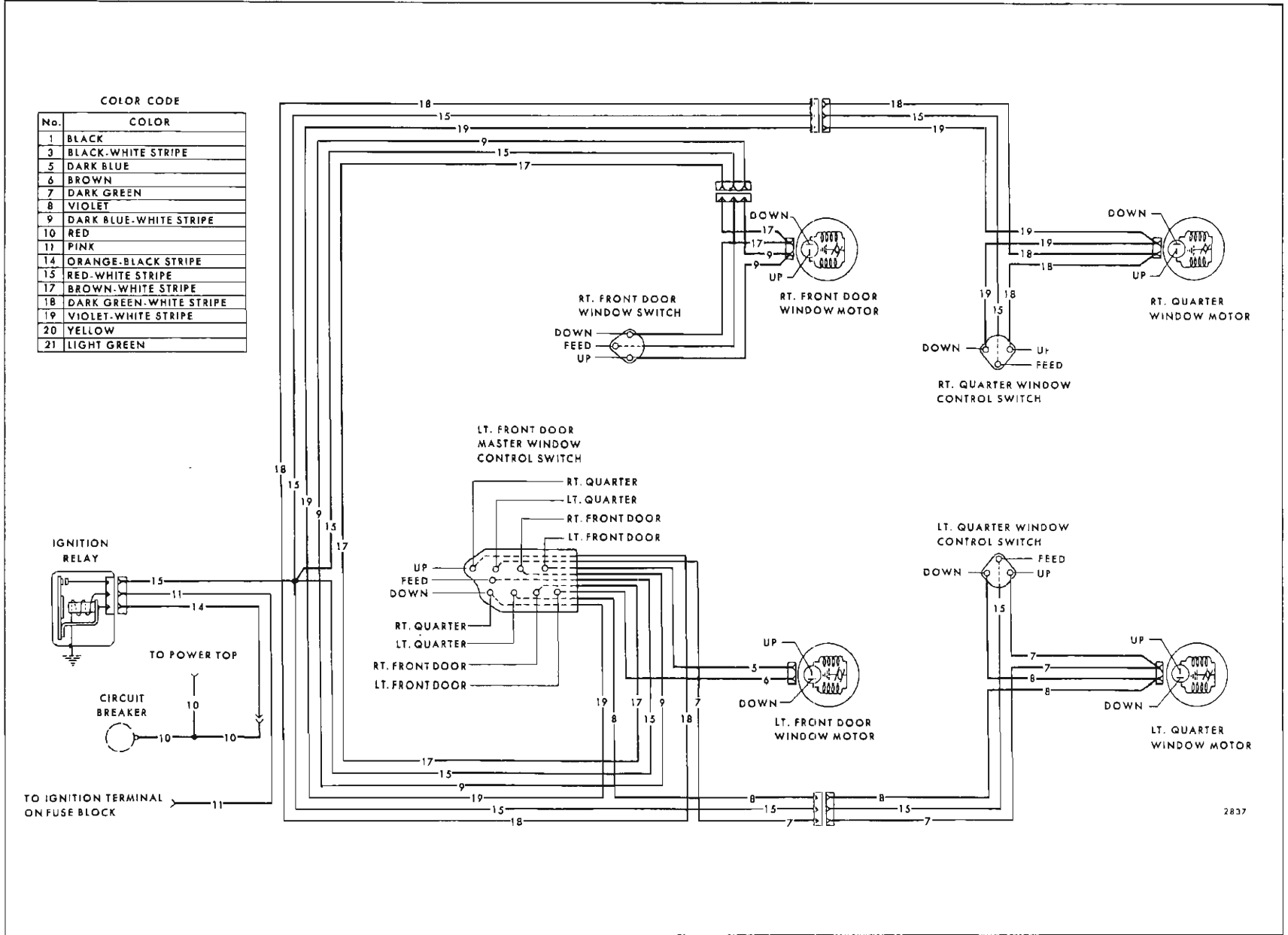
Fig. 16-3—Power Window Circuit - Chevrolet and Pontiac "F" Styles
