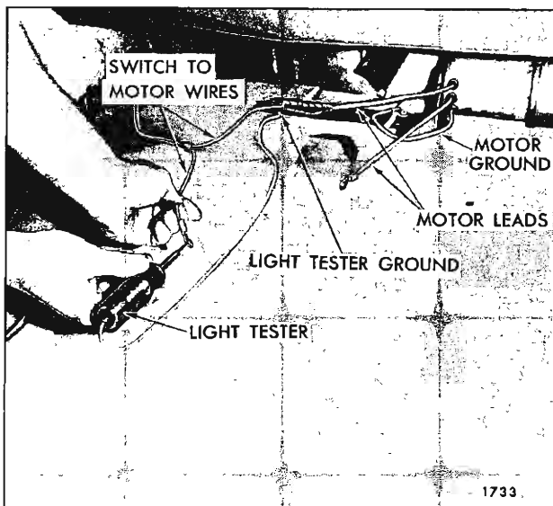
Fig. 13-66—Checking Wire Leads to Motor
