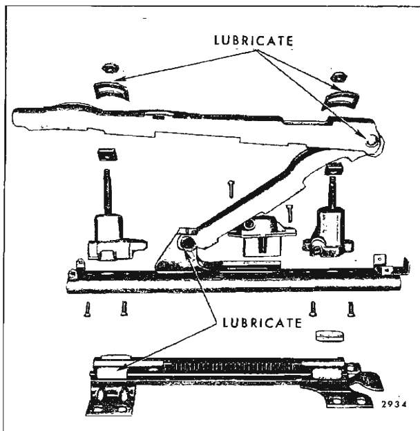
Fig. 2-15—Front Seat Adjuster Lubrication
