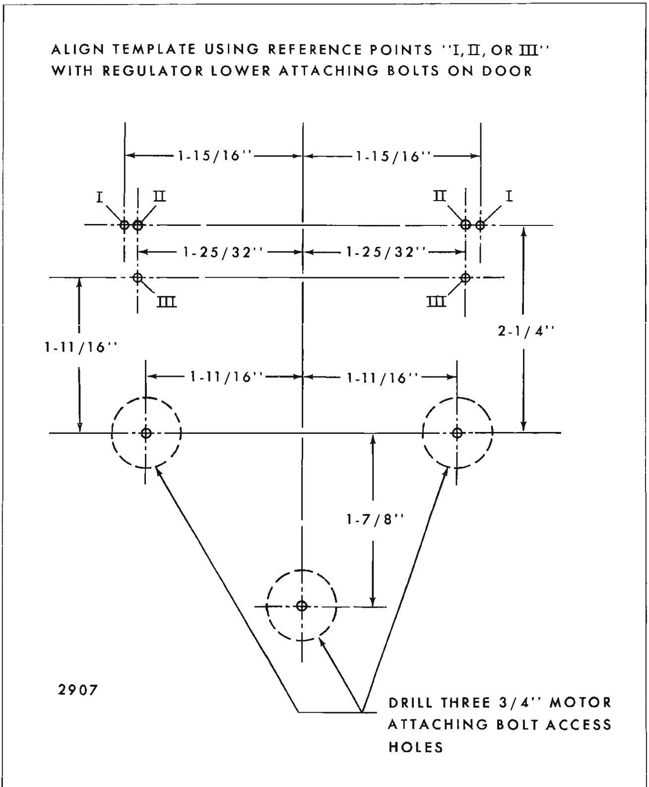
Fig. 6-34—Window Regulator Lower Attaching Bolts Reference Points for Locating Window Motor to Regulator Attaching Bolts: "I" for "B and C-11, 37, 47, 57 and 67" Style Front Doors; "II" for "C-69" Style Rear Doors; "III" for "B-36, 39, 46 and 69" and "C-49 and 69" Style Front and Rear Doors, Except "C-69" Style Rear Doors
