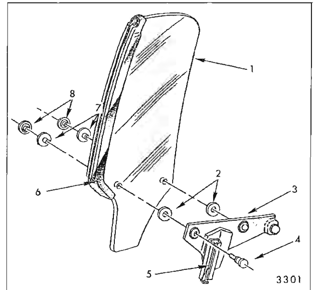
Fig. 7-30—Rear Quarter Window Assembly - “E-47” Styles
