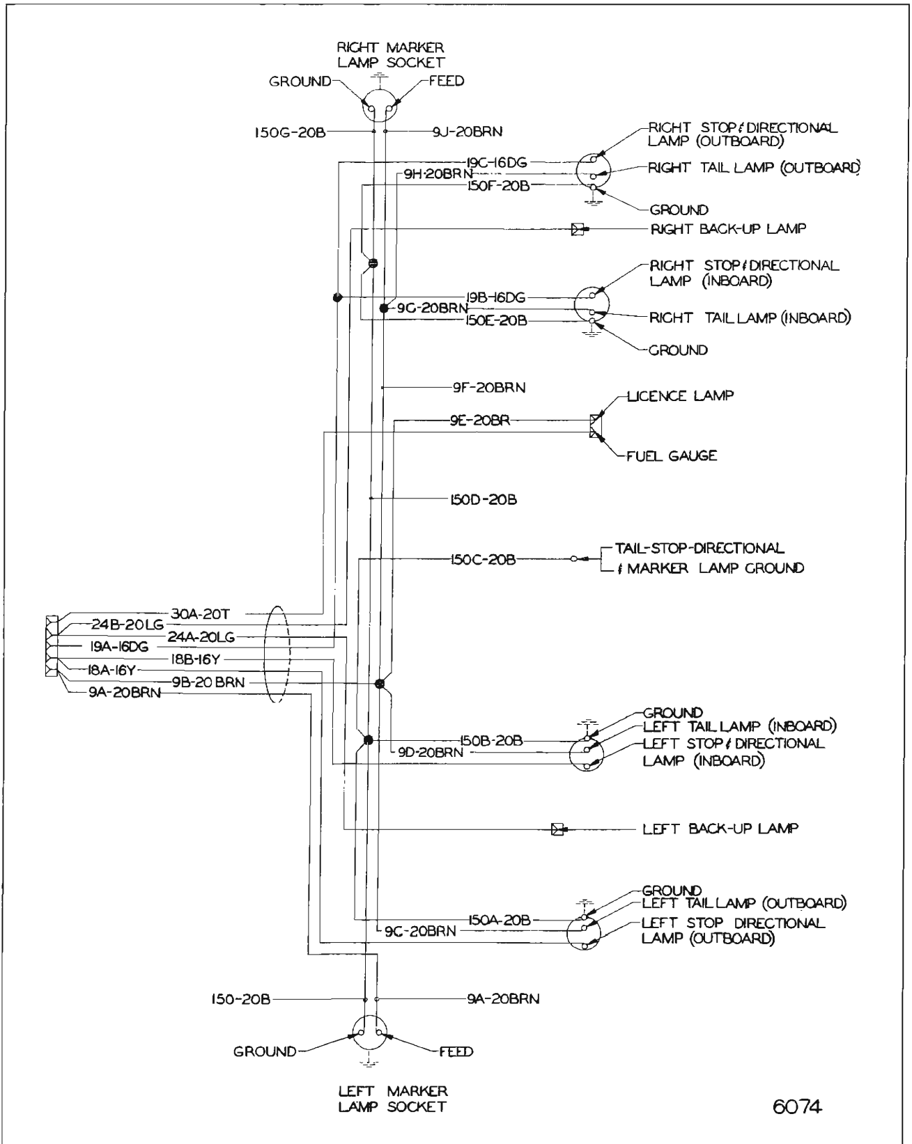
Fig. 16-53—Wiring Diagram Rear - Chevrolet "F" Styles
