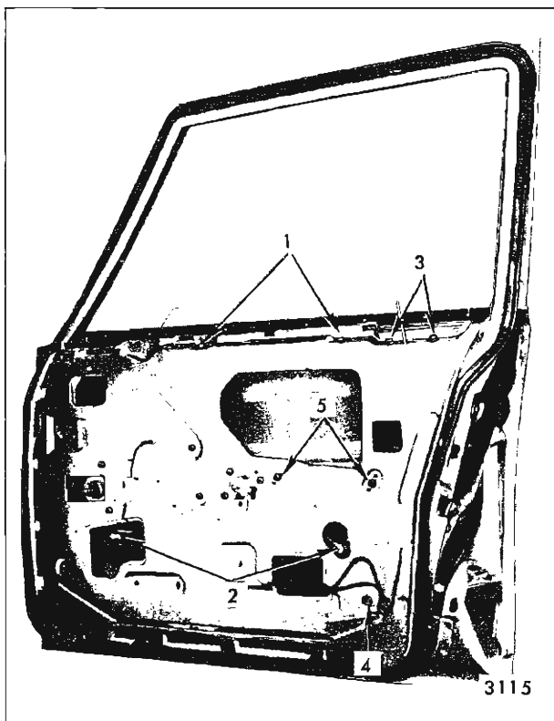
Fig. 6-86—Window Removal and Adjustment - "B-69" Styles
