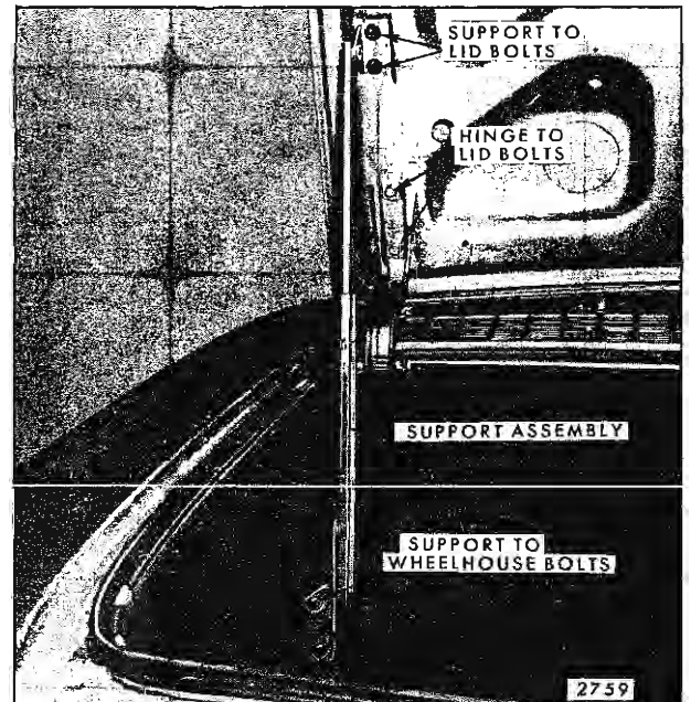
Fig. 8-3—Engine Compartment Lid Attachments - All "Z" Styles
