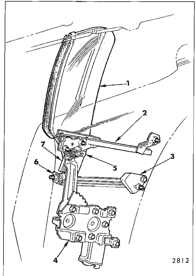
Fig. 7-26—Rear Quarter Hardware - Cadillac "E" Body
