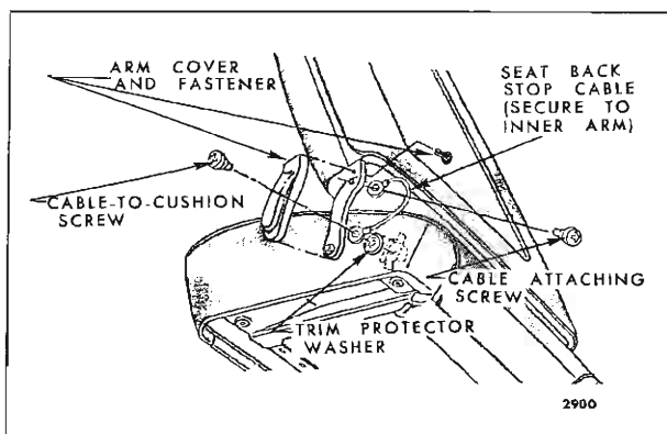
Fig. 15-47—Bucket Seat Back Stop Cable—"F & Z" Styles
