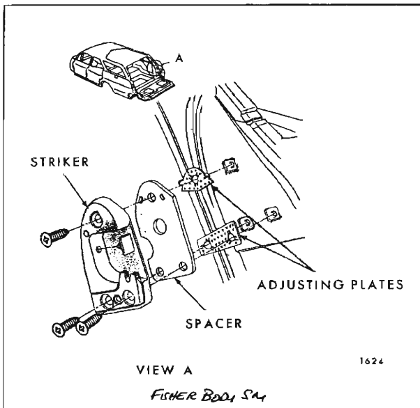
Fig. 9-48—Tail Gate Striker Assembly
