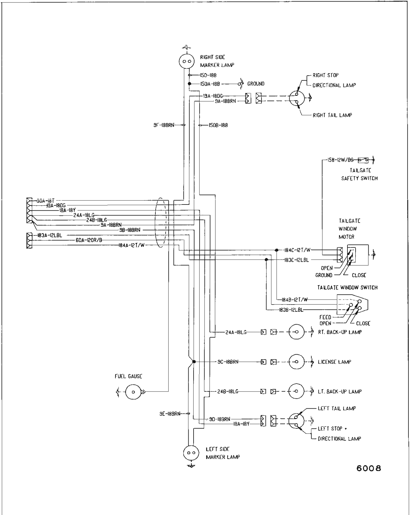
Fig. 16-18—Power Tail Gate Window Rear Wiring Circuit - Buick "A" Styles
