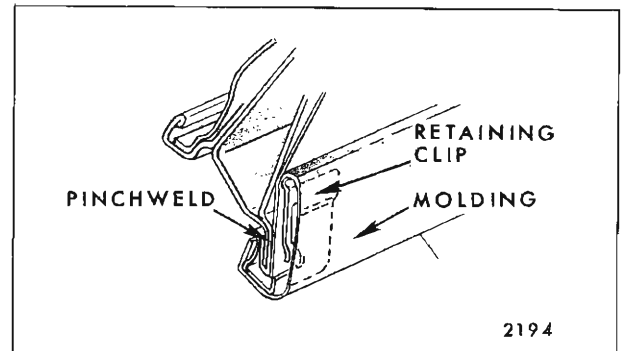
Fig. 11-2—Side Roof Rail Garnish Moldings
