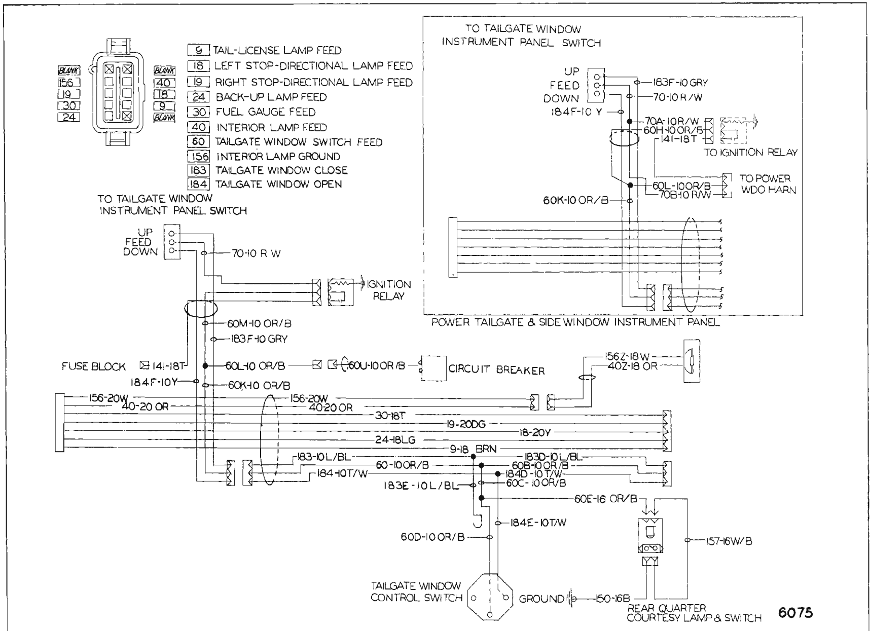
Fig. 16-11—Power Tail Gate Window Front Wiring Circuit - Chevrolet "A" Styles
