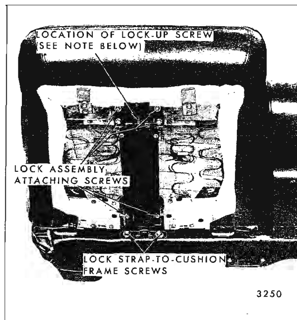
Fig. 15-53—Strato Seat Back Lock Assembly
