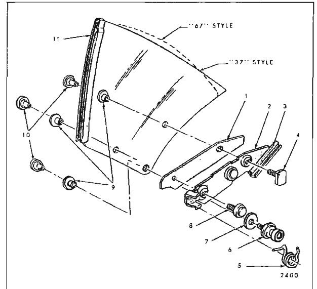
Fig. 7-35—Rear Quarter Window Assembly - "F" Style
