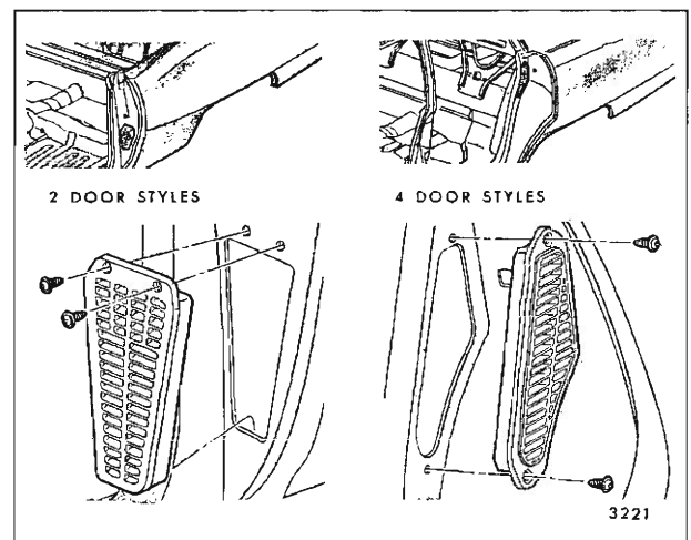
Fig. 5-17—Pressure Relief Valve - "B & C" Styles Shown
