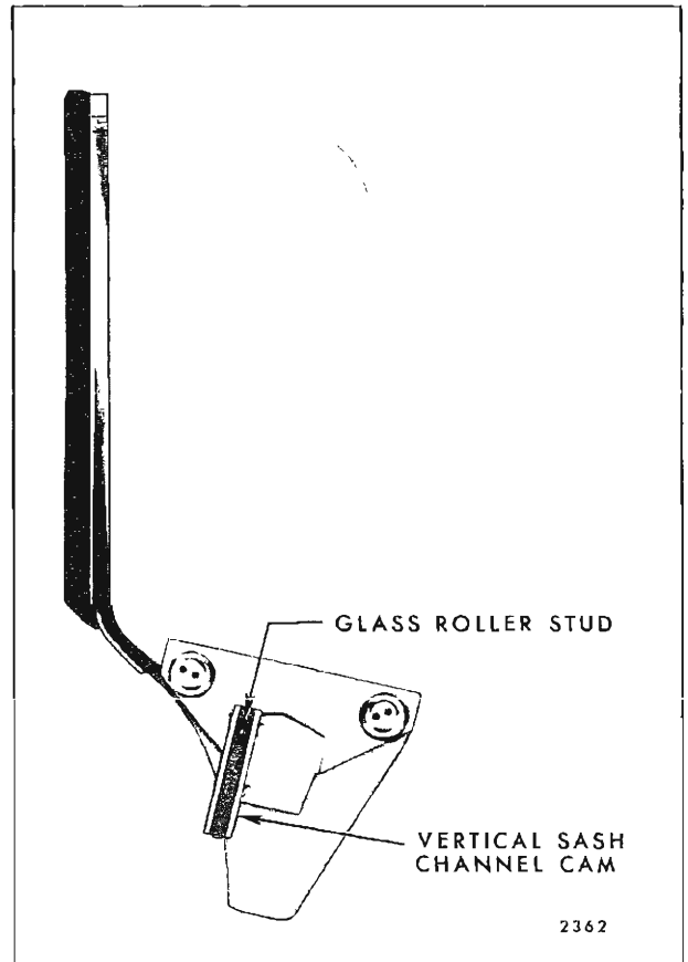
Fig. 7-28—Rear Quarter Window Assembly - "E-47" Styles
