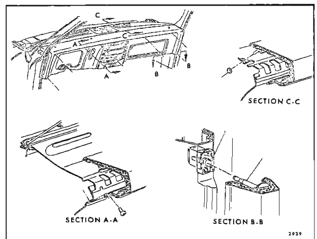
Fig. 5-21—Instrument Panel Cover - Pontiac "F" Styles
