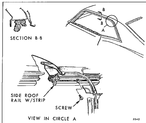
Fig. 6-13—Side Roof Rail Weatherstrip - "47-57" Styles
