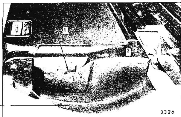
Fig. 2-11—Dual Acting Tailgate Lubrication - Right Side
