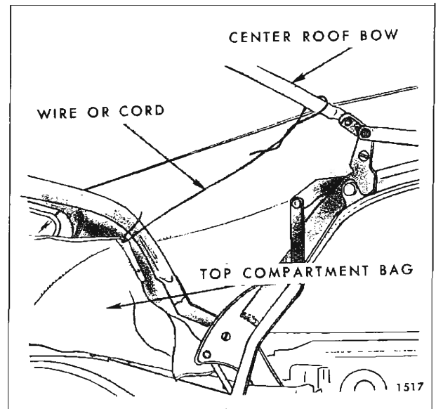
Fig. 13-9—Raising Folding Top Compartment Bag
