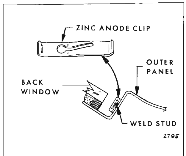
Fig. 17-6—Zinc-Anode Clip Installation
