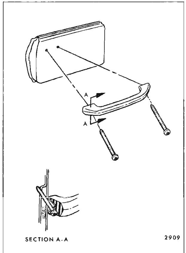
Fig. 14-3—Door Pull Handle Attachment - "F" Styles
