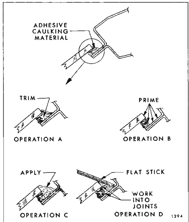
Fig. 4-11—Adhesive Caulked Glass Waterleak Correction
