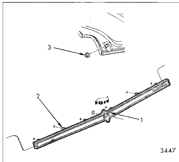
Fig. 8-19—Rear Compartment Lower Moldings
