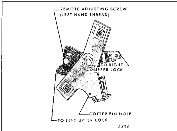
Fig. 9-24—Tail Gate Lock Remote Control - Gate Operation
