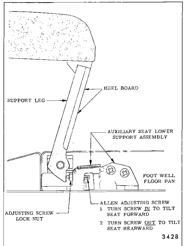
Fig. 15-63—Auxiliary Seat Adjustment - Cadillac Limousine Styles
