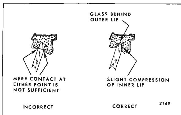
Fig. 6-125—Window to Side Roof Rail Weatherstrip Alignment
