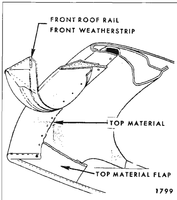
Fig. 13-17—Top Cover at Front Roof Rail
