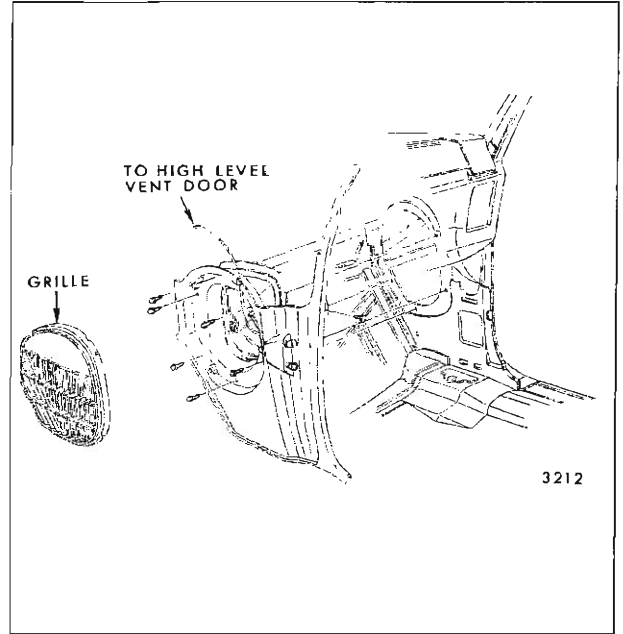
Fig. 5-8—Shroud Side Finishing Panel - "B & C" Styles
