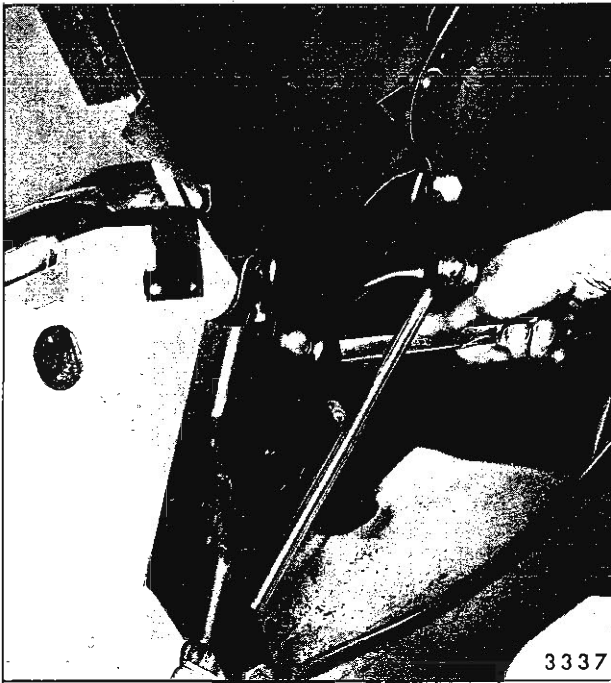
Fig. 13-7—Trimstick Removal "A" Styles
