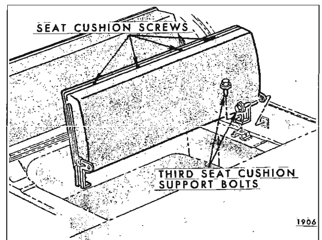
Fig. 15-72—Folding Third Seat Cushion
