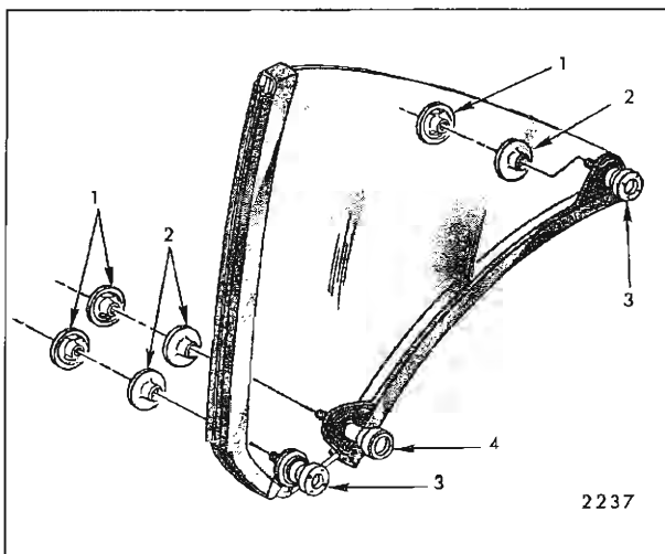
Fig. 7-25—Rear Quarter Window Assembly - "E-87" Style
