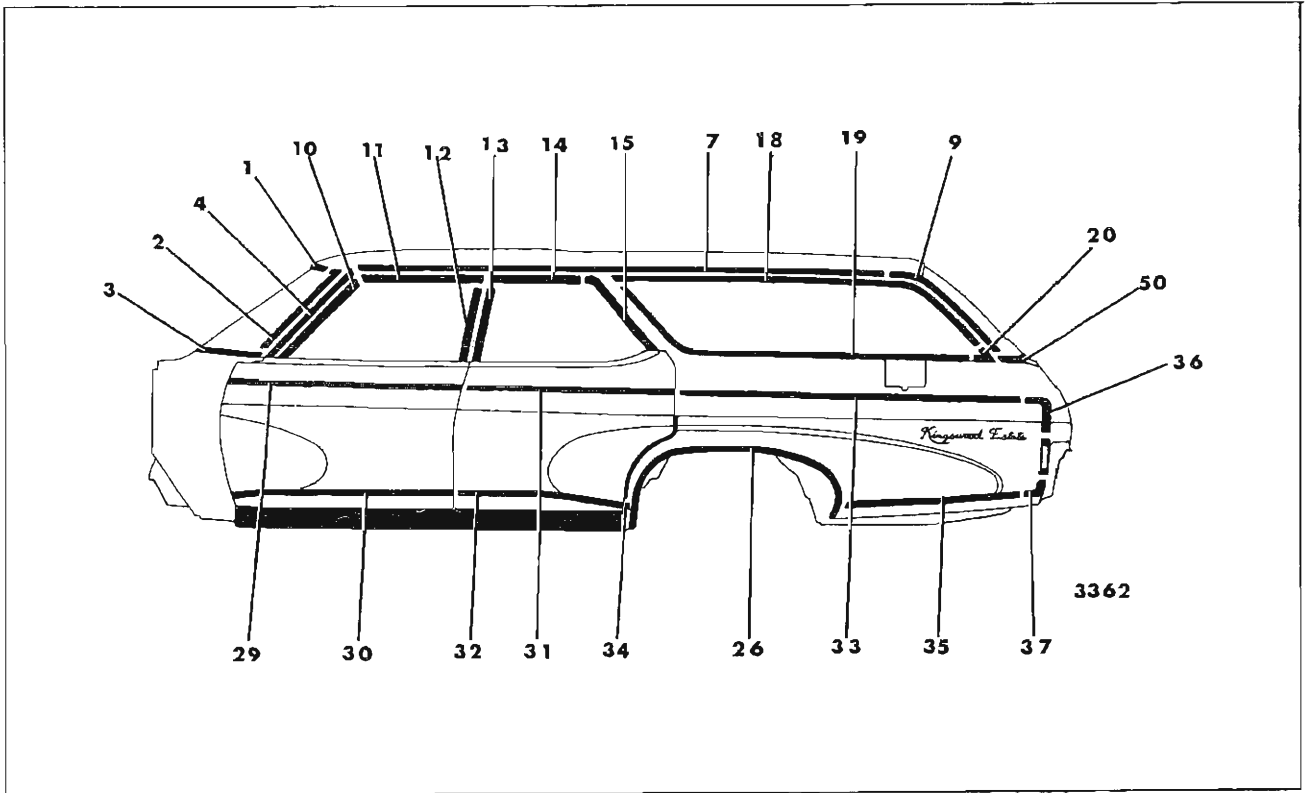
Fig. 17-23—Chevrolet 16636-46 Styles
