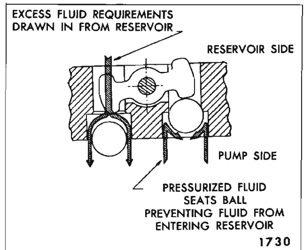
Fig. 13-64—Fluid Control Valve
