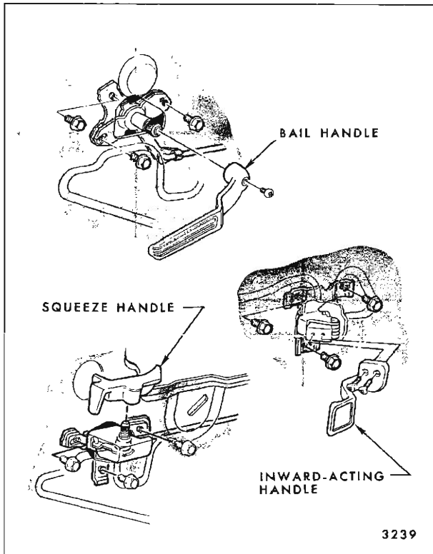
Fig. 14-9—Door Inside Remote Control Handles
