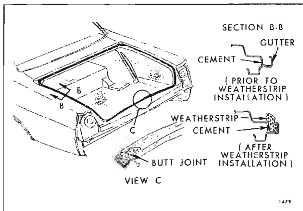
Fig. 8-31—Rear Compartment Weatherstrip Assembly
