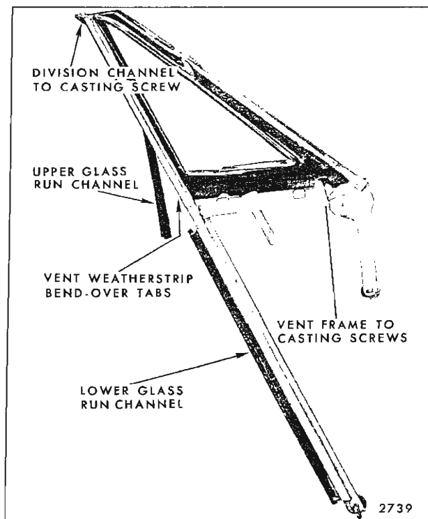
Fig. 6-71—Front Door Ventilator Assembly - "A" Closed Styles
