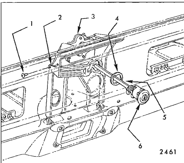
Fig. 8-14—Typical Rear Compartment Lid Lock Cylinder Installation (Side Load)
