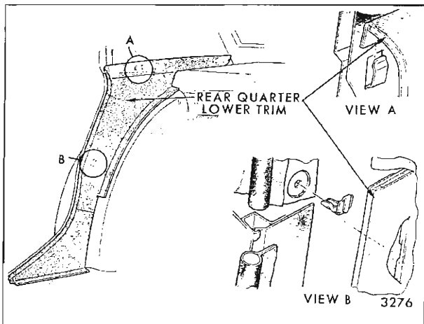
Fig. 14-31—Rear Quarter Trim Assembly - "C" Four-Door Style
