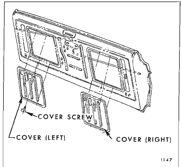
Fig. 9-3—Tail Gate Inner Panel Access Hole Cover
