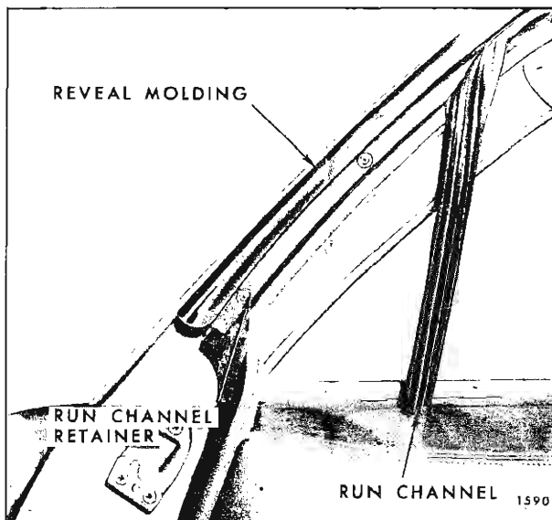
Fig. 9-54—Tail Gate Upper Glass Run Channel Retention
