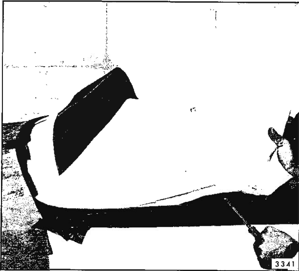
Fig. 13-48—Raising End of Trimstick "A" Styles
