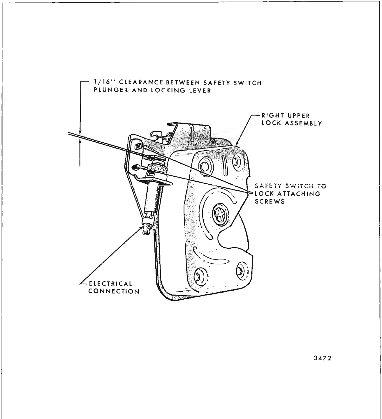
Fig. 9-27—Dual Tail Gate Electrical Safety Switch
