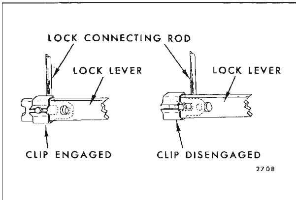
Fig. 6-19—Door Lock Spring Clip
