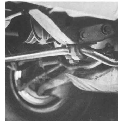
Ride & Handling Package (Code 621—UPC Y96). For improved cornering and handling—extra-firm front and rear springs and shocks, for all Pontiac models. Heavier stabilizer bar for Tempest and Pontiac series only. (F)
