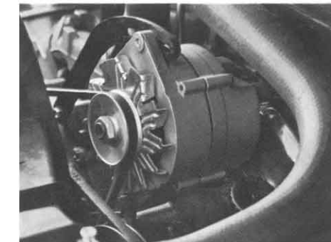
Delcotron Alternator-Regulator (62-Amp. Code 681—UPC K81; 55-Amp. Code 682—UPC K82; Self-regulated 55-Amp. Code 688—UPC K96). Special "solid state" voltage regulator, built into the alternator, provides improved voltage control and added reliability—increases battery life. Available for all series equipped with V-8 engines. Style and amperage determined by engine or equipment. (F)
