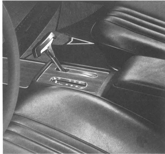
Console for 2-speed Automatic and Turbo Hydra-Matic. The console for the 2-speed automatic is extra-cost on LeMans (except 4-door Hardtop). Both consoles feature dark walnut wood grain appearance insert and padded top panel. The console for Turbo Hydra-Matic on GTO features a "Rally Sports" speed shift unit that permits fully automatic or manual shifting.
