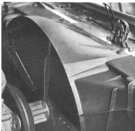
Heavy-duty Radiator (Code 701—UPC V01). Has greater cooling capacity; standard with air-conditioned cars. Available for all models. Also, SUPER-COOLING, HEAVY-DUTY RADIATOR (Code 702—UPC V02), for cooling under most severe driving conditions. Available for Catalina, Executive and Bonneville. (F)
