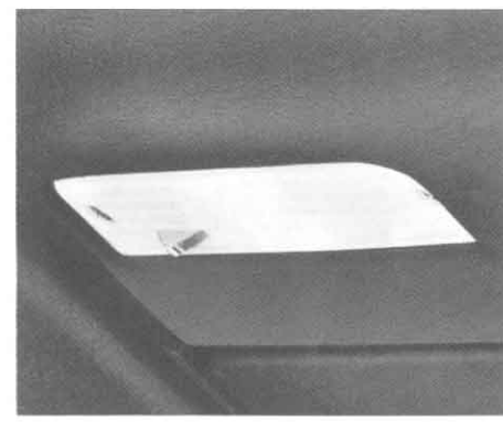
Instrument Panel Courtesy Lamp (Code 661—UPC U29). Available for Tempest and Custom S models only—included in Lamp Group (Code 322). Standard on all other models, all series. Lights when front doors are opened. Also may be manually operated by switch on lamp. (F,D)
